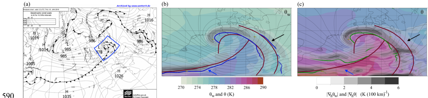
590 Figure 13. Comparison of UK Met Office fronts with objective fronts, case Friederike (18 January 2018, 12:00 UTC). (a) UK Met Office surface analysis chart. Blue box marks analysed area. (b) Objective 850 hPa 2-D fronts (blue lines) as detected from ECMWF HRES \theta_w (colour; grey shading shows |\nabla_h \theta_w| ), UK Met Office fronts (red lines), and mean sea level pressure (black contour lines, spacing 2 hPa). (c) Same as (b) but objective 2-D fronts (green lines) based on \theta . The secondary front (black arrow) is only detected when using \theta_w . When based on \theta , the cold front (blue arrow) breaks up and is less continuous compared to the cold front based on \theta_w .
