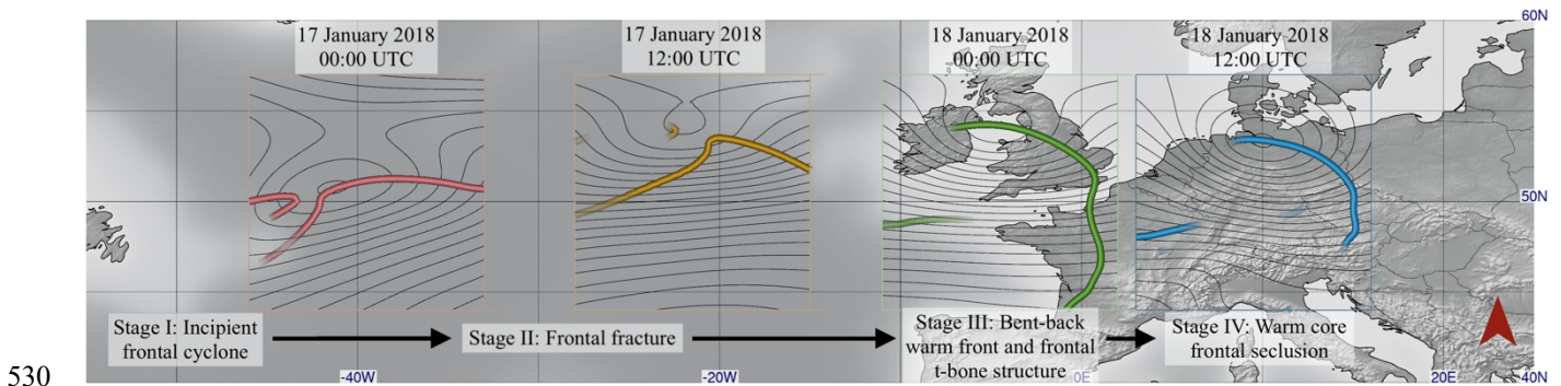
Figure 11: Successive time steps of objective 2-D frontal structures showing the temporal development of Friederike (17 and 18 January 2018), as detected in ERA-5 reanalysis data at 750 hPa and surface pressure (black lines). The displayed time steps are approximately assigned to the four ideal development stages of the Shapiro-Keyser cyclone model (Shapiro and Keyser, 1990). We find that not all characteristics of the individual stages can be observed in 2-D. As shown in the following, 3-D front detection is required to observe all characteristics (cf. Figure 12).
