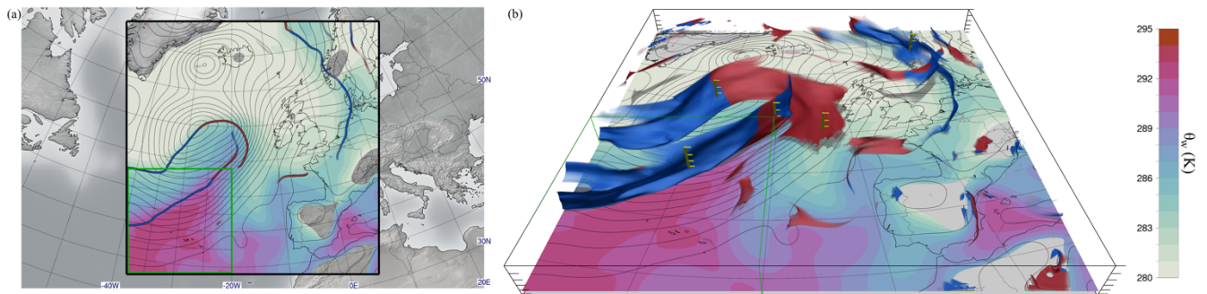
430 Figure 6. Cyclone Vladiana on 23 September 2016, 06:00 UTC. (a) Detected 2-D warm (red line) and cold (blue line) fronts at 850 hPa, \theta_w at 950 hPa (colours, in K), and mean sea level pressure (black contour lines, every 2 hPa) from a COSMO simulation (black frame shows domain boundaries; green frame shows the selected subregion for studying convection in the vicinity of the cold front, cf. Sect. 4.2.2). (b) Detected 3-D warm (red) and cold (blue) fronts between 950 hPa and 500 hPa, on top of a horizontal map showing \theta_w at 950 hPa and mean sea level pressure (black contour lines, every 2 hPa). Warm and cold front classification is computed according to warm and cold air advection at the front (following Hewson, 1998).
