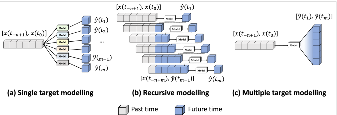
Figure 9. Three forecasting designs in DL-QPN with radar sequence. (a) Single, (b) recursive, and (c) multiple predictions.
