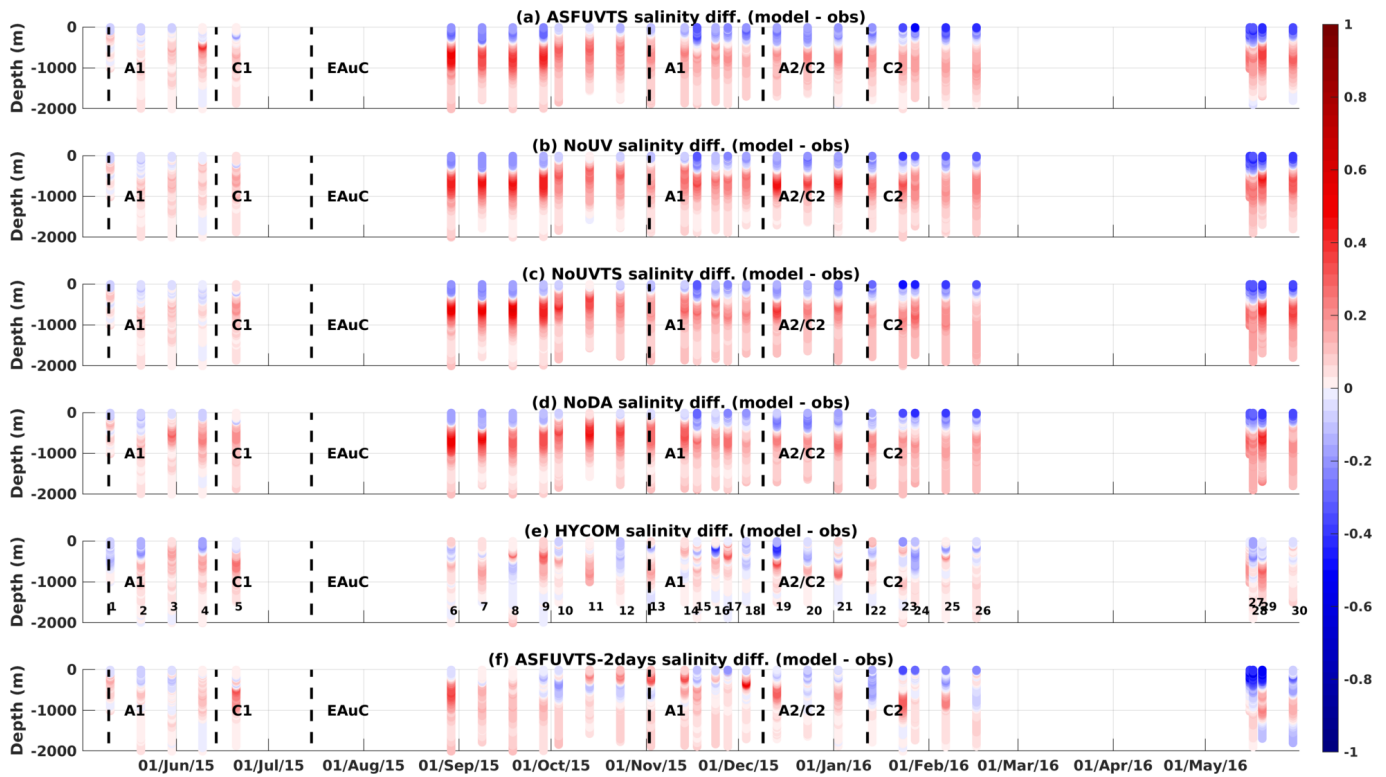
Figure 9. Salinity difference between modelled and Argo observations from experiments (a) ASFUVTS, (b) NoUV, (c) NoUVTS, (d) NoDA, (e) HYCOM-NCODA, (f) ASFUVTS-2days. The numbers in (e) show the dates when Argo profilers sampled the NZNES. The locations of the Argo floats are shown in Fig. 10e. The acronyms A1, C1, EAuC, A1, A2/C2, and C2 represent mesoscale structures near M5 which were studied in Santana et al. (2021).
