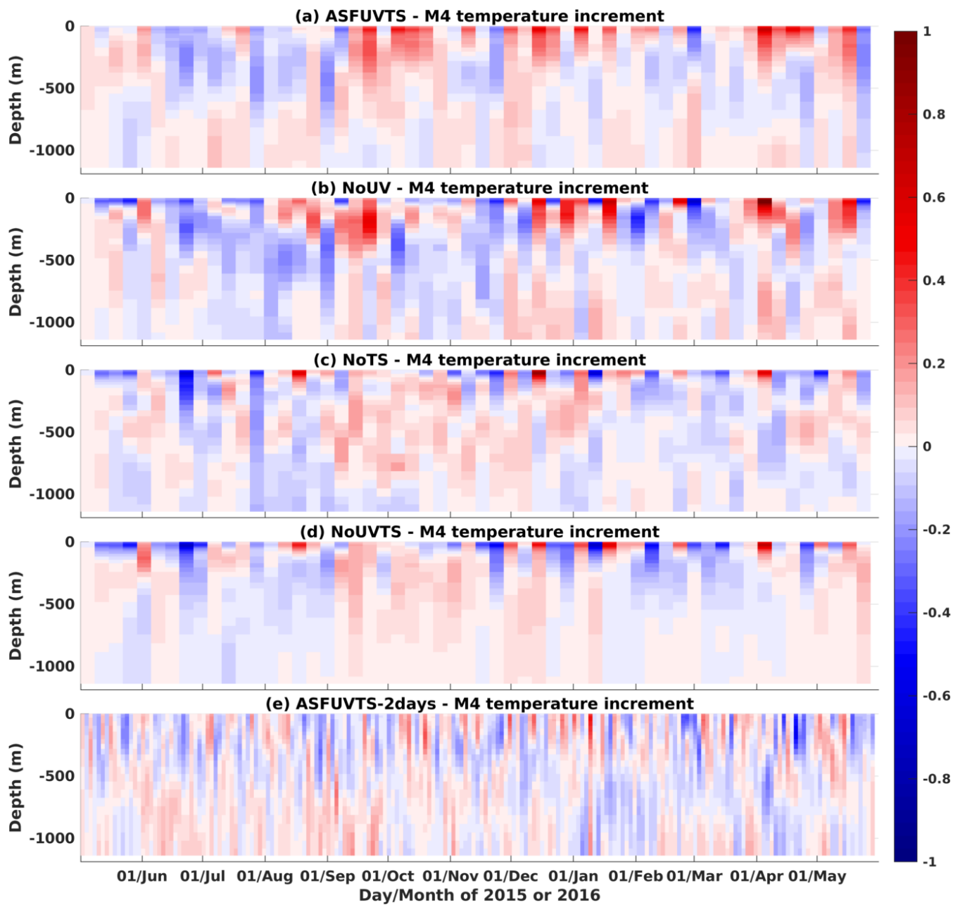
Figure 11. Time variability of temperature increments (°C) to the initial conditions at M4 from experiments (a) ASFUVTS, (b) NoUV run, (c) NoTS, (d) NoUVTS, and (e) ASFUVTS-2days.
