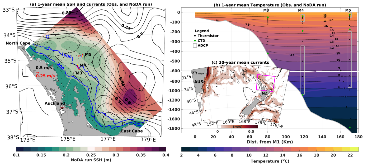
Figure 1. (a) Study area showing the one-year average SSH from AVISO (black contours) and NoDA run (green-red shade), and near-surface velocities NoDA run (black arrows). The stations M3 to M5 are indicated along the grey line. The coloured arrows represent the vertically averaged (bin = 280 m) in situ velocities centred at 140 m (red), 420 m (cyan), 700 m (blue), and 980 m (yellow). (b) Temporal averages of temperature from in situ measurements (coloured contours) and the NoDA run (coloured shade). The grey rectangles show regions sampled by ADCPs at M4 and M5 and the vertical positions of thermistors and CTDs are indicated as black and green dots, respectively. (c) Location of the study area (magenta contour) in the Southwest Pacific Ocean. The colours and arrows represent the 20-year average of geostrophic currents. Current speeds lower than 0.05 m/s were masked. The 200- and 1000-meter isobaths are shown as blue and black contours in (a) and (c).
