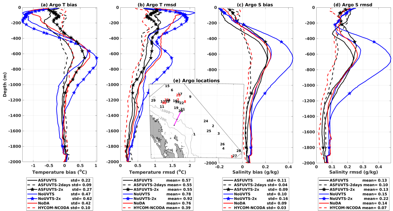
Figure 10. Profiles of mean bias and root mean square deviation (rmsd) between model and independent Argo observations of temperature (a,b) and salinity (c,d). Solid black line (ASFUVTS), dashed black line (ASFUVTS-2days), starred black line (ASFUVTS-2x), solid blue line (NoUVTS), starred blue line (NoUVTS-2x), red line (NoDA), and dashed red line (HYCOM-NCODA). The stars represent the median depth of thermistors and CTDs (CTDs) at M3, M4 and M5 in temperature (salinity) bias and rmsd profiles. Results from experiments NoUV and NoTS were not shown for better visualisation. (e) Map of Argo locations which are represented as numbers in black or red for better visualisation only. The moorings' locations are shown as black dots on the magenta line.
