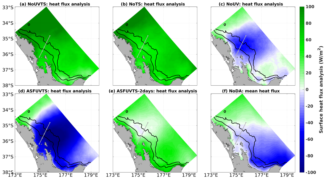
Figure 13. Average surface net heat flux analysis ( \text{W/m}^2 ) (positive = downward) in experiments (a) NoUVTS, (b) NoTS, (c) NoUV, (d) ASFUVTS, and (e) ASFUVTS-2days. (f) shows mean net heat flux in the freely evolving simulation (NoDA). Green (blue) colours show positive (negative) mean surface heat flux.
