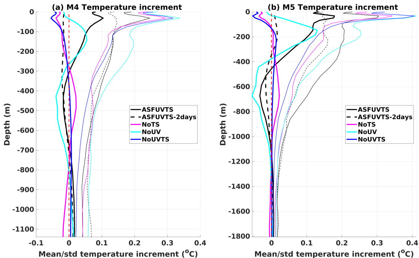
Figure 12. Profile of average (thick lines) and standard deviation (thin lines) increment to initial conditions of temperature at M4 (a) and M5 (b). Solid black line (ASFUVTS), dashed black line (ASFUVTS-2days), pink (magenta) line (NoTS), light blue (cyan) line (NoUV) and dark blue line (NoUVTS). The red dashed line marks the 0 °C increment.
