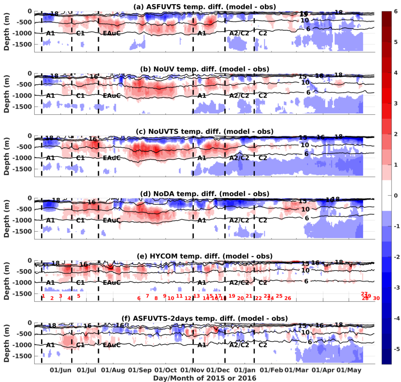
Figure 7. (a) Difference between model and observed daily average temperature at M5 for experiments (a) ASFUVTS, (b) NoUV, (c) NoUVTS, (d) NoDA, (e) HYCOM-NCODA, and (f) ASFUVTS-2days. The red numbers in (e) show the dates when Argo profilers sampled the NZNES. The locations of the Argo floats are shown in Fig. 10e. The acronyms A1, C1, EAuC, A1, A2/C2, and C2 represent mesoscale structures near M5 which were studied in Santana et al. (2021).
