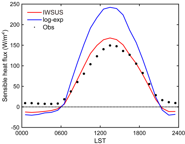
Figure 10 Daily variation of sensible heat flux. Red line and blue line represents fluxes obtained from IWSUS and exp-log law (Masson, 2000) respectively. Dots represent the flux observation from Offerle et al. (Offerle et al., 2006).
