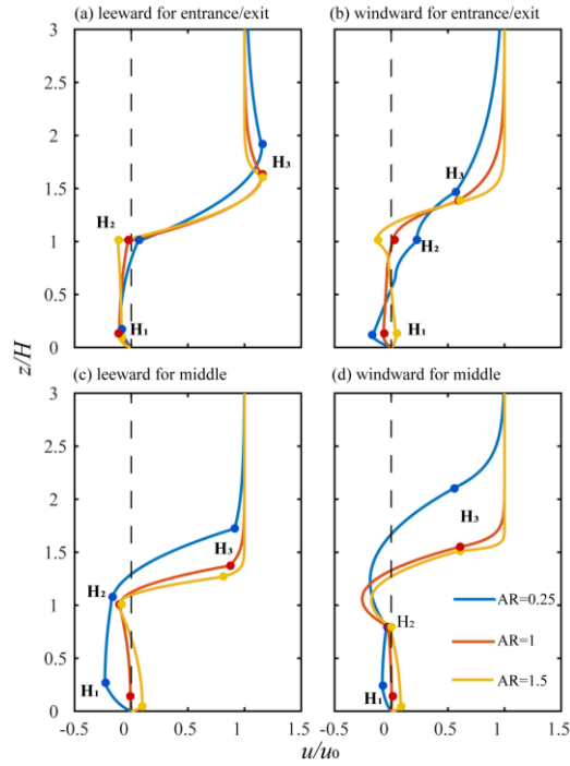
315 Figure 6 Wind profile of u component obtained from IWSUS at different positions with AR= 0.25, 1 and 1.5 . The point H_i are the segmentation points referred in Table 2 and Table 3.
