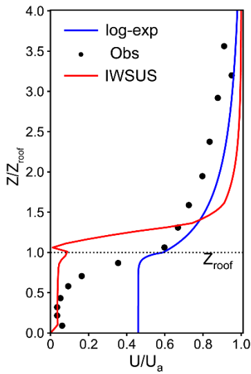
400 Figure 9 Overall averaged wind vertical profiles by IWSUS, exp-log law and the observation.
