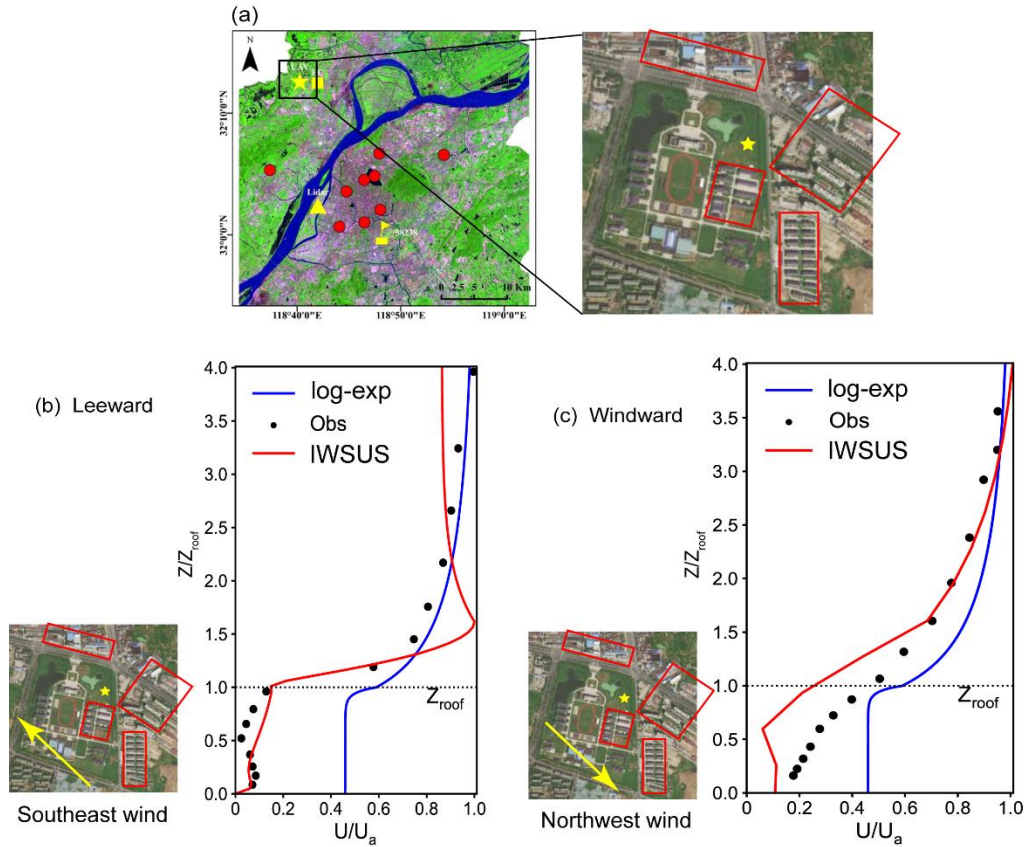
380 Figure 8 Overall wind vertical profiles comparison between IWSUS, exp-log law and observations in various wind direction scenarios. The location of the observation point is marked as a yellow pentagram (Liu et al., 2020; Liu et al., 2021) in the left of Figure 8a with the specific surrounding environment (from Baidu Maps) in the right; the red boxes are the main existence of the high-rise buildings nearby; Figure 8b and 8c show the vertical wind profile obtained from IWSUS (red line)m exp-log (blue line) and observations (black dots) at the observation site under leeward side with southeast wind scenarios and windward side with northwest wind scenarios, respectively. 385
