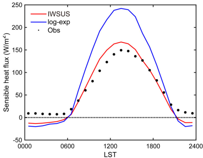
430 Figure 10 Daily variation of sensible heat flux. Red line and blue line represents fluxes obtained from IWSUS and exp-log law (Masson, 2000) respectively. Dots represent the flux observation from Offerle et al. (Offerle et al., 2006).
