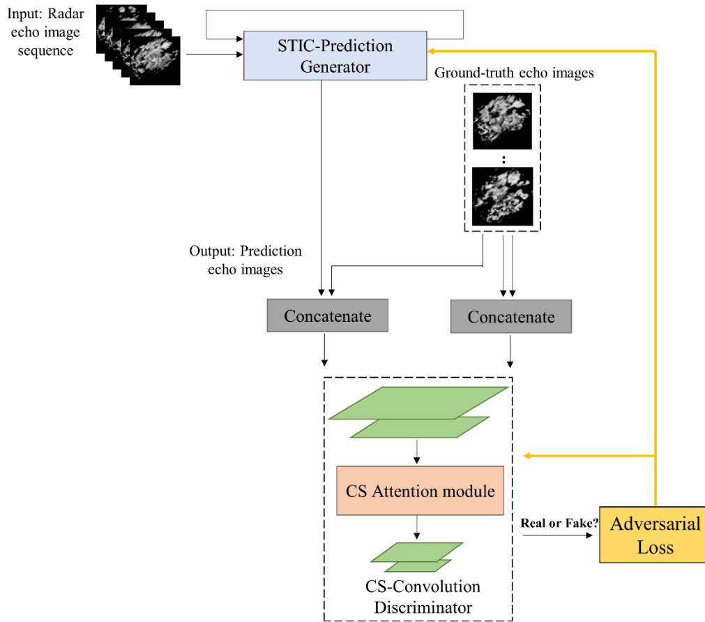
155 Figure 1 2: This is the structure of GAN-argcPredNet v2.0. Fifteen radar echo images are used in the testing set. Fifteen radar echo images are used as a test sequence. Here, the first five images are used as the input sequence, and the last ten images are used as the ground-truth images. The generator generates images based on input sequences. The discriminator judges both the predictive images and Ground-truth images. The adversarial loss is then obtained to optimize the model.
