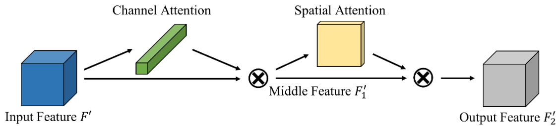
195 Figure 45: This is the structure of CS Attention. The calculation order is first through the Channel Attention module and then through the Spatial Attention module.
