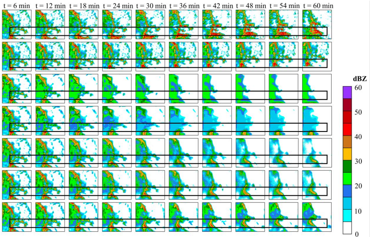
Figure 10: The example of rapid storm growth in radar echo extrapolation. From top to bottom: ground truth frames; prediction by the optical flow; prediction by ConvGRU; prediction by ConvLSTM; prediction by GA-ConvGRU; prediction by GAN-argcPredNet v1.0; prediction by GAN-argcPredNet v2.0. The rectangular region represents the prediction for rapid storm growth.
