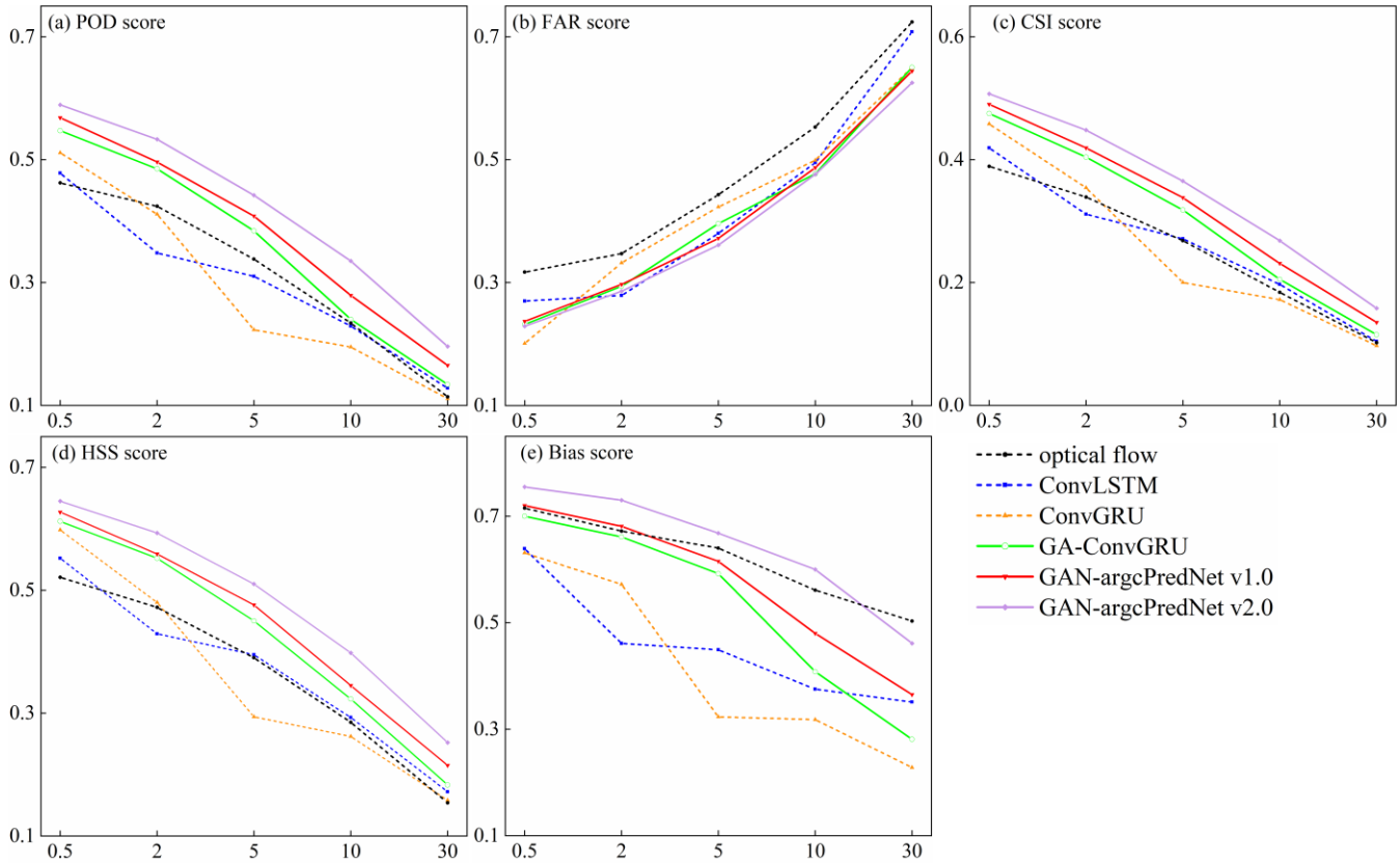
Figure 78: This is t he average scores of (a) POD, (b) FAR, (c) CSI, (d) HSS and (e) Bias under different threshold. All the time steps were used to compute the scores. The horizontal axis represents the threshold, in units of mm h -1 . The perfect score of FAR is 0, and while the others are 1.
