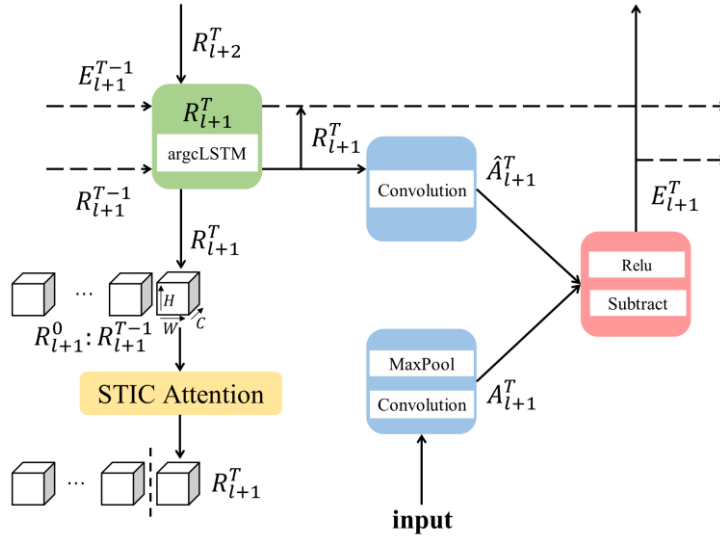
160 Figure 23: This is the structure of STIC Prediction. Modules are in l = 2 at time T . The STIC-Prediction structure at time T with l = 1 ( l = 0, 1, 2, 3 ). STIC Attention is after the third layer. Before R_{l+1}^T enters the R_l^T module, R_{l+1}^T forms a sequence R_{l+1}^0 : R_{l+1}^{T-1} with the previous R_{l+1} . STIC Attention focuses on the importance of different regions of the sequence. Finally, the new R_{l+1}^T is fed to the R_l^T module. See Section 2.2 for further explanation.
