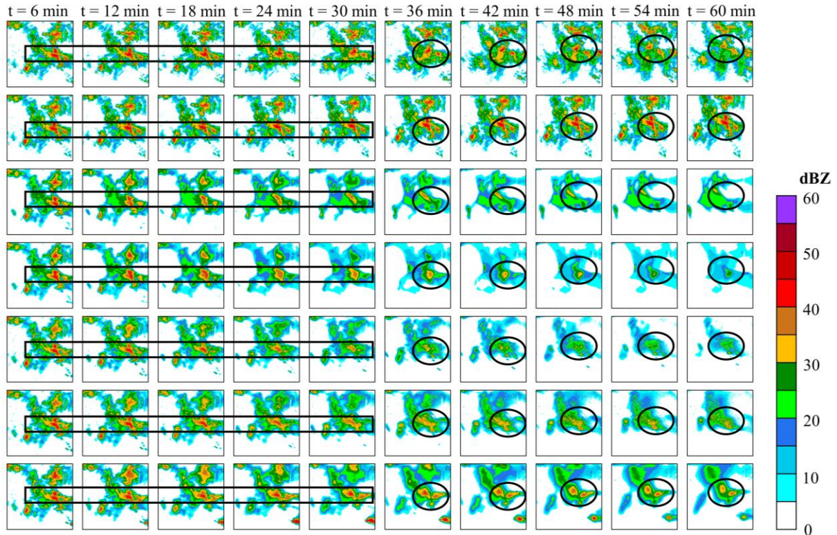
320 Figure 89: This is the example of the growth of weather system in radar echo extrapolation. From top to bottom: ground truth frames; prediction by the optical flow; prediction by ConvGRU; prediction by ConvLSTM; prediction by GA-ConvGRU; prediction by GAN-argcPredNet v1.0; prediction by GAN-argcPredNet v2.0. The circular and rectangular regions represent heavy rainfall prediction, where the performance of the models in extrapolating heavy rainfall can be observed.
