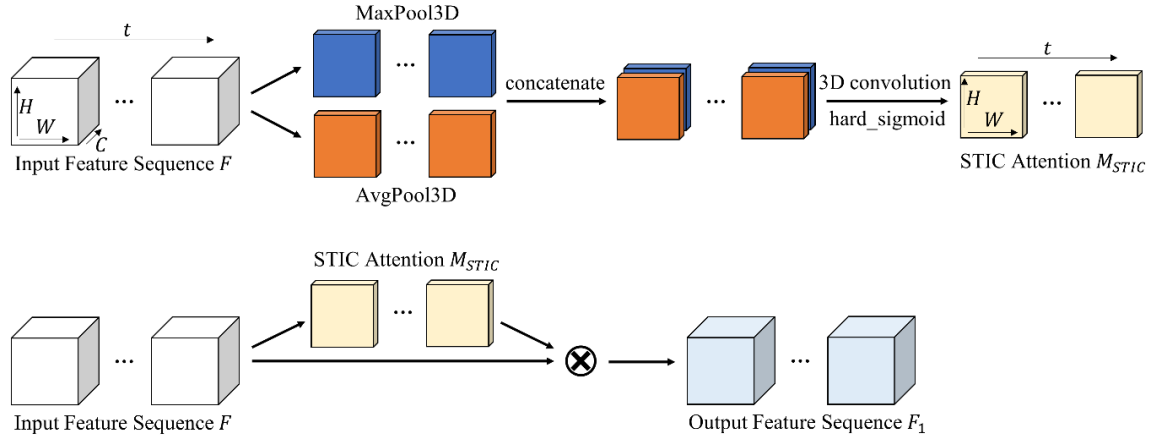
185 Figure 34: This is the structure of STIC Attention. The first line represents the calculation process of the STIC Attention map sequence. The second line represents the process of applying the STIC Attention map sequence to the input feature sequence.
