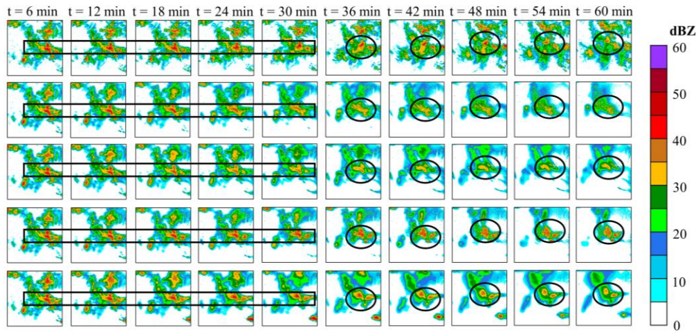
355 Figure 912: This is t The example of radar echo extrapolation. From top to bottom: ground truth frames; prediction by GAN-argcPredNet v1.0; prediction by CS-GAN; prediction by STIC-GAN; prediction by GAN-argcPredNet v2.0. The circular and rectangular regions represent heavy rainfall prediction.
