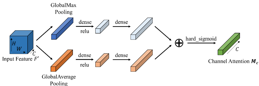
Figure 56: This is the structure of Channel Attention. Channel Attention utilizes maximum pooling outputs and average pooling outputs with their respective networks.
