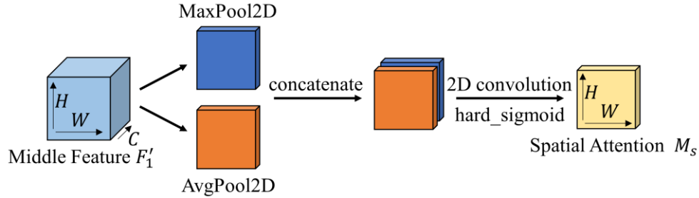
Figure 67: This is the The structure of Spatial Attention. Spatial Attention utilizes the maximum and average pooling outputs along the channel axis and forwards them to the convolutional layer.
