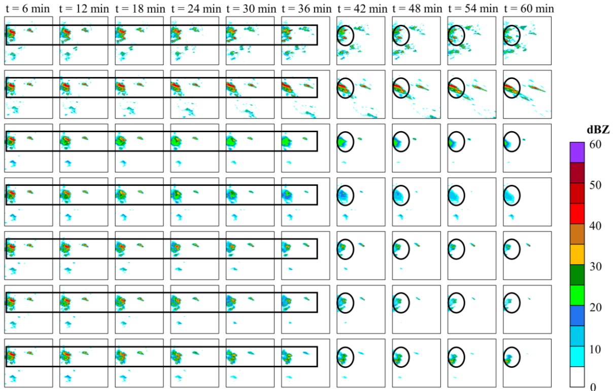
Figure 11: The example of storm decay in radar echo extrapolation. From top to bottom: ground truth frames; prediction by the optical flow; prediction by ConvGRU; prediction by ConvLSTM; prediction by GA-ConvGRU; prediction by GAN-argcPredNet v1.0; prediction by GAN-argcPredNet v2.0. The circular and rectangular regions represent heavy rainfall prediction.
