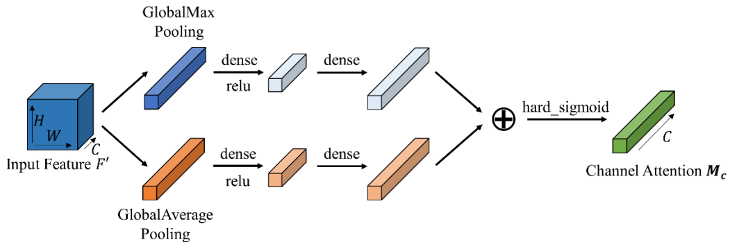
Figure 5: This is the structure of Channel Attention.
