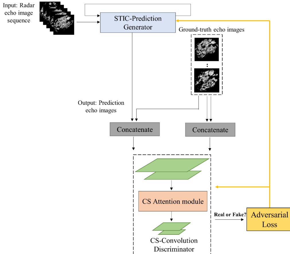
Figure 1: This is the structure of GAN-argcPredNet v2.0. Twelve-Fifteen radar echo images are used in the testing set. Here, five images are used as the input sequence, and seven-ten images are used as the ground-truth images.
