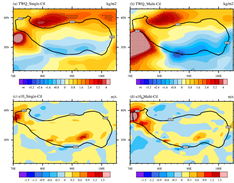
450 Figure 8. Difference of (a–b) total precipitable water ( \text{kg m}^{-2} ) and (c–d) 10-m wind speed ( \text{m s}^{-1} ) between Single, Multi and Ctl experiments. Dotted areas are statistically significant at the 90% confidence level.
