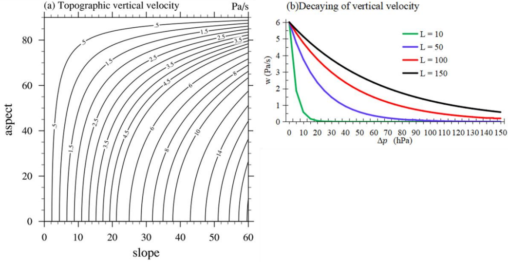
220 Figure 1. (a) Distribution of surface topographic vertical velocity (Pa/s) at different slope and aspect in 10m/s wind speed; (b) the decreasing of the unit topographic vertical velocity with height at different grid scales.
