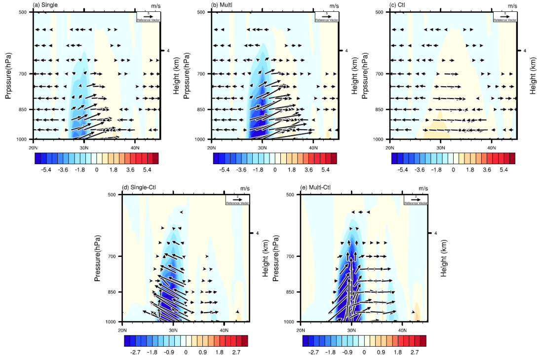
430 Figure 7. Meridional-vertical circulation (vectors) and vertical velocity (shading) averaged over 87°E–95°E in (a) Single, (b) Multi and (c) Ctl experiments, and their differences (d) between the Single and Ctl experiments and (e) between the Multi and Ctl experiments.
