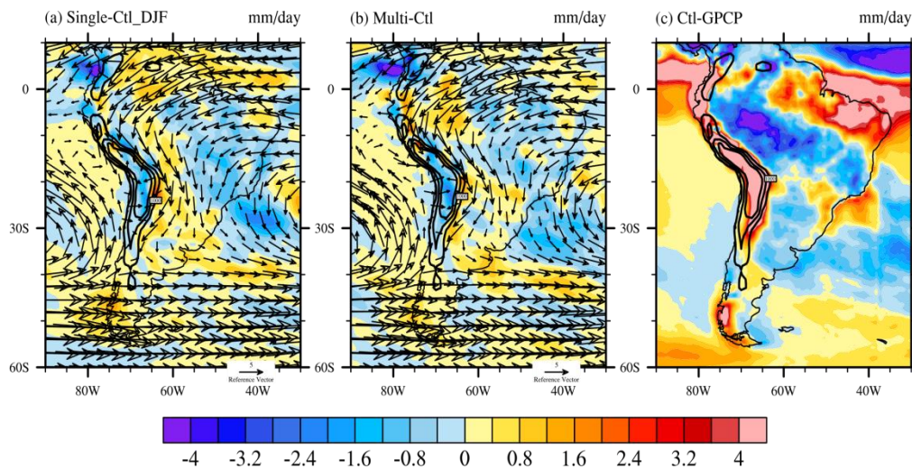
Figure 11. Differences of winter (December–February) average precipitation amount (mm day -1 ) (a) between Single and Ctl experiments, (b) between Multi and Ctl experiments and (c) between Ctl experiment and GPCP over South America. Vectors in Fig. 11a and 11b represent the 850 hPa wind in the Single and Multi experiments, respectively. Black contours indicate the altitudes of 1000 m and 2000 m.
