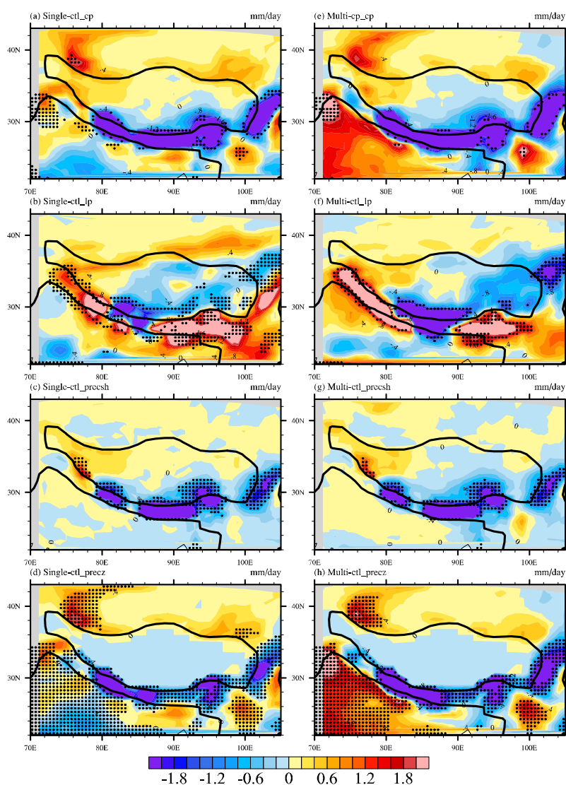
375 Figure 5. Difference of (a) convective precipitation, (b) large-scale precipitation, (c) shallow convection precipitation, (d) precipitation from ZM convection between Single and Ctl experiments. (e-h) As in (a-d) but between Multi and Ctl experiments. Black contours indicate the altitudes of 500 m and 4000 m. Dotted areas are statistically
