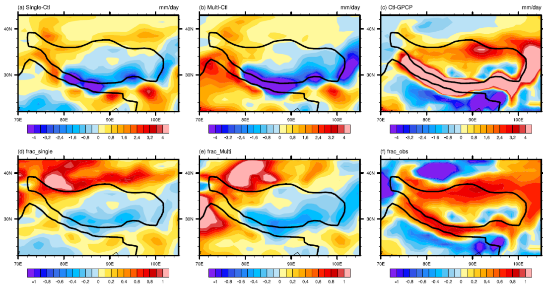
Figure 3. Differences of summer average precipitation amount ( \text{mm day}^{-1} ) (a) between
