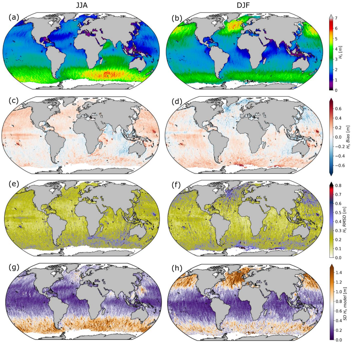
340 Figure 5. (a,b) Mean, (c,d) bias and (e,f) root mean square deviation ( RMSD ) between modelled significant wave height ( H_s ) and merged altimeter observations (MA_SUP03), and (g,h) model standard deviation ( SD_{model} ) across the global domain for GS512L4EUK-AN. Stats are aggregated every 15-days and averaged for the months June-July-August (JJA; left column) and December-January-February (DJF; right column) over 2019-2020.
