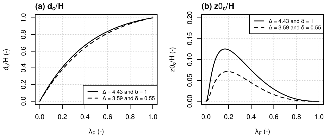
Figure 2. (a) d_c/\overline{H} and (b) z_{0_c}/\overline{H} as a function of the plan and frontal area densities ( \lambda_P and \lambda_F ) calculated with Maedonald et al. (1998) equations by Eq. 3.
