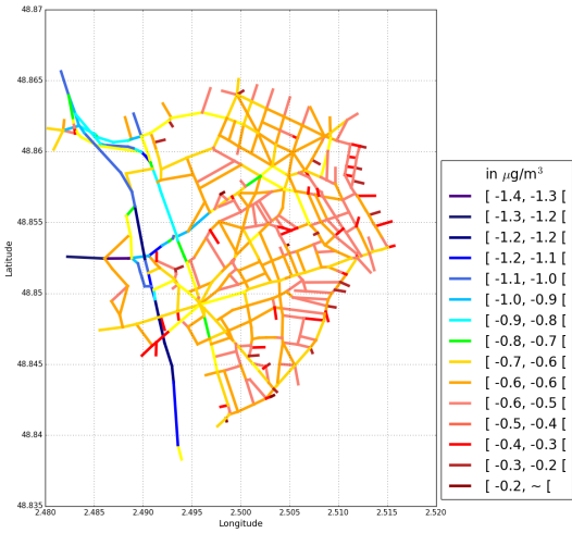
(b) Ammonium
