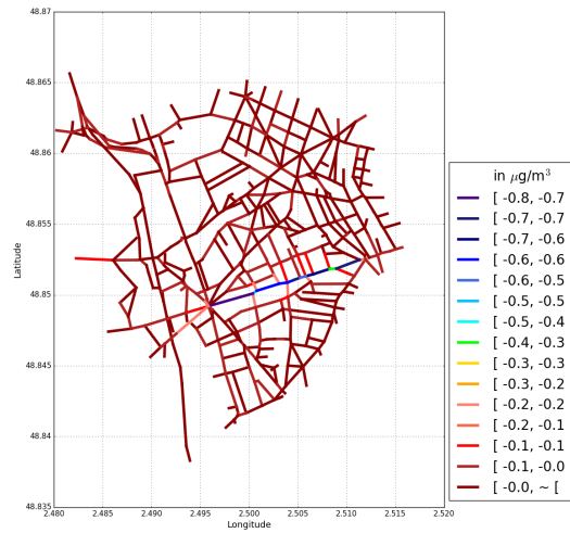
(a) \text{NO}_2
