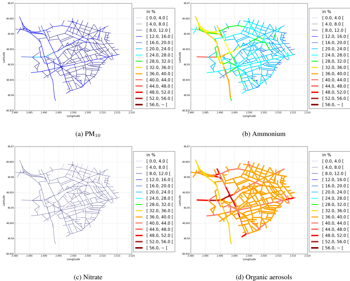
Figure 9. Temporal NME (in %) between Case-1 and Case-2 for (a) PM_{10} , (b) Ammonium, (c) Nitrate and (d) Organic aerosols. The absolute differences in the concentrations between the simulations are presented in additional figures in Appendix C.
