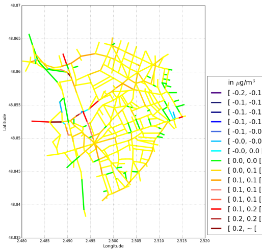
(b) Ammonium
