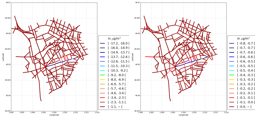
(a) \text{NO}_2
