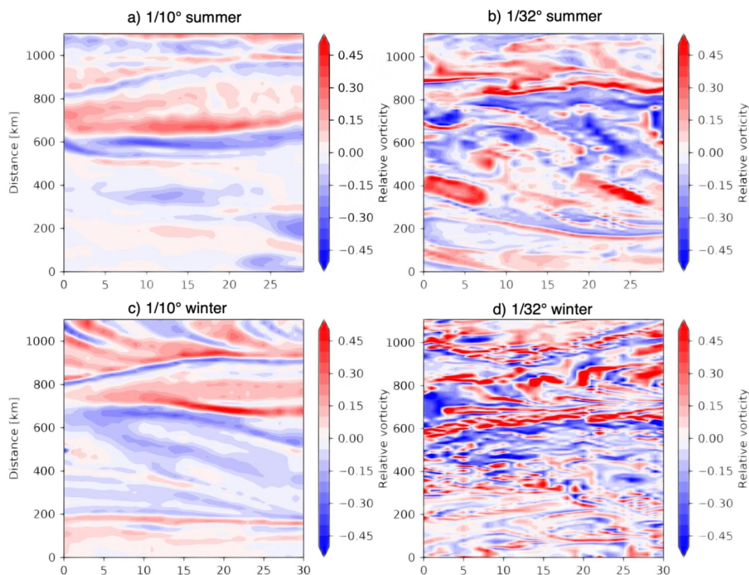
Figure A-3 Hovmöller diagram of relative vorticity along a section in Kuroshio extension region, marked as black line shown in Figure 6.
