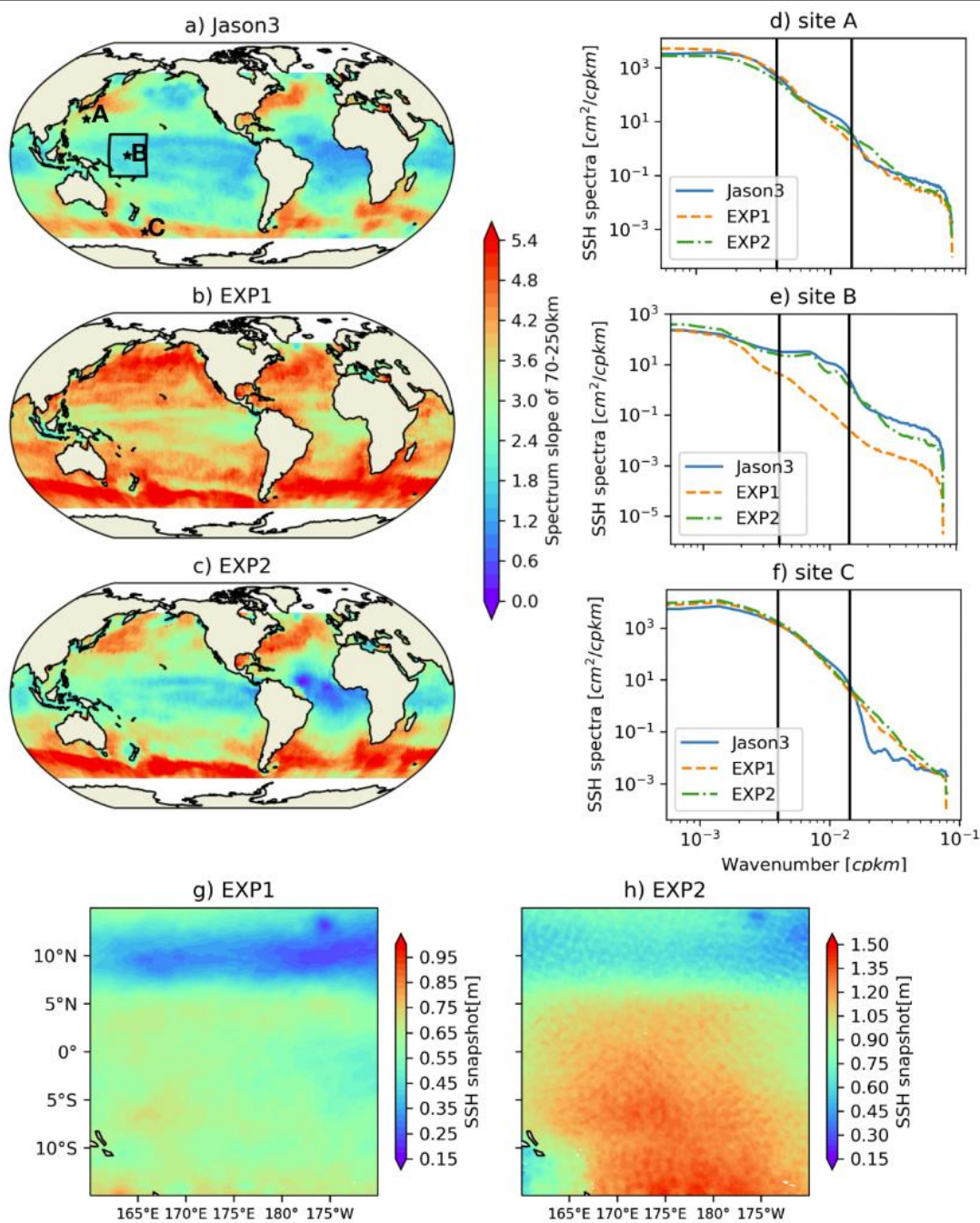
Figure 14 SSH wavenumber spectrum slope of 70-250 km of Jason 3 along track data (a), EXP1 (b) and EXP2 (c). SSH wavenumber spectrum at three sites in regions of Kuroshio extension (d), tropical Pacific Ocean (e) and Southern Ocean (f), the black lines denote the wavenumber of 70 and 250 km. Snapshots of SSH of EXP1 (g) and EXP2 (h) on 1 December 2018 in the rectangle region are shown in (a). Note that the sign of the spectrum slope is reversed to make them positive in a-c.
