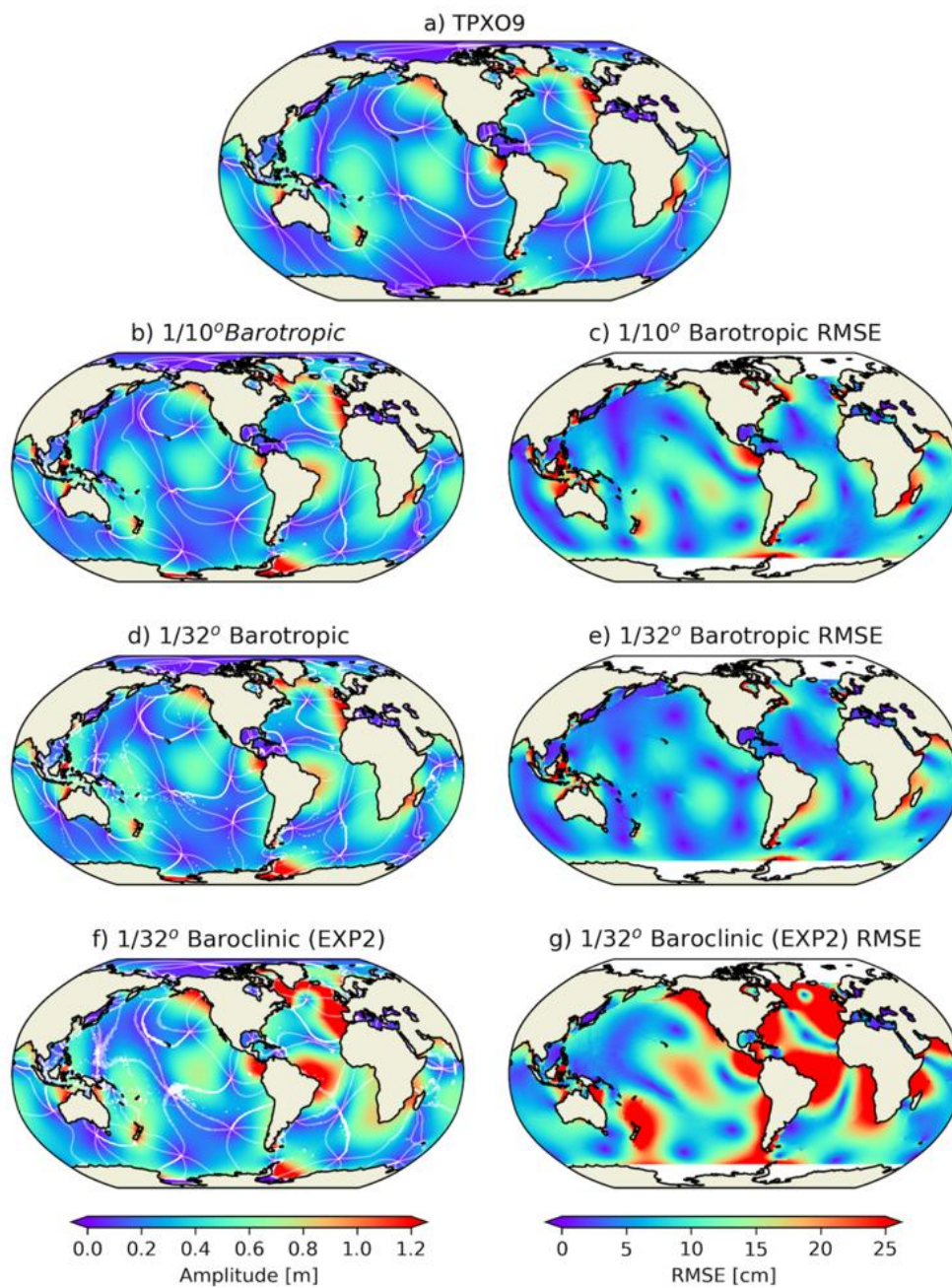
Figure 8 M 2 co-tidal charts of TPXO9 (a), barotropic tide model of 1/10° (b) and 1/32°(d) with topographic drag parameterisation best tuned, baroclinic tide model of 1/32° (EXP2) (f) without topographic drag parameterisation, and their RMSE errors (c, e and g).
