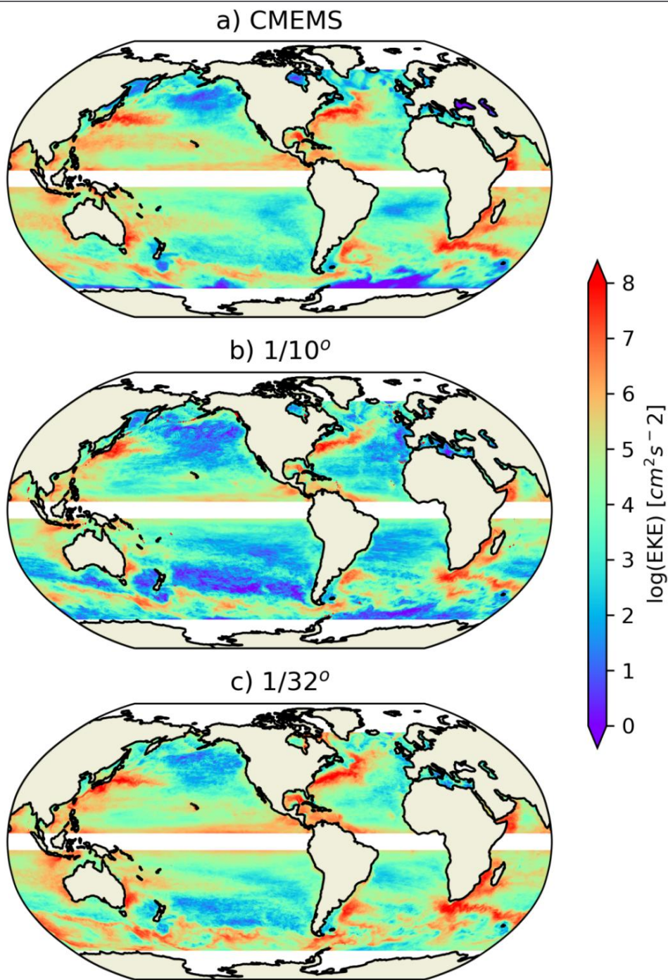
Figure 1 Eddy kinetic energy (EKE) of CMEMS from all satellite merged grided data (a), FIO-COM10 (EXP1Low) (b), and FIO-COM32 (EXP1) (c) model results.
