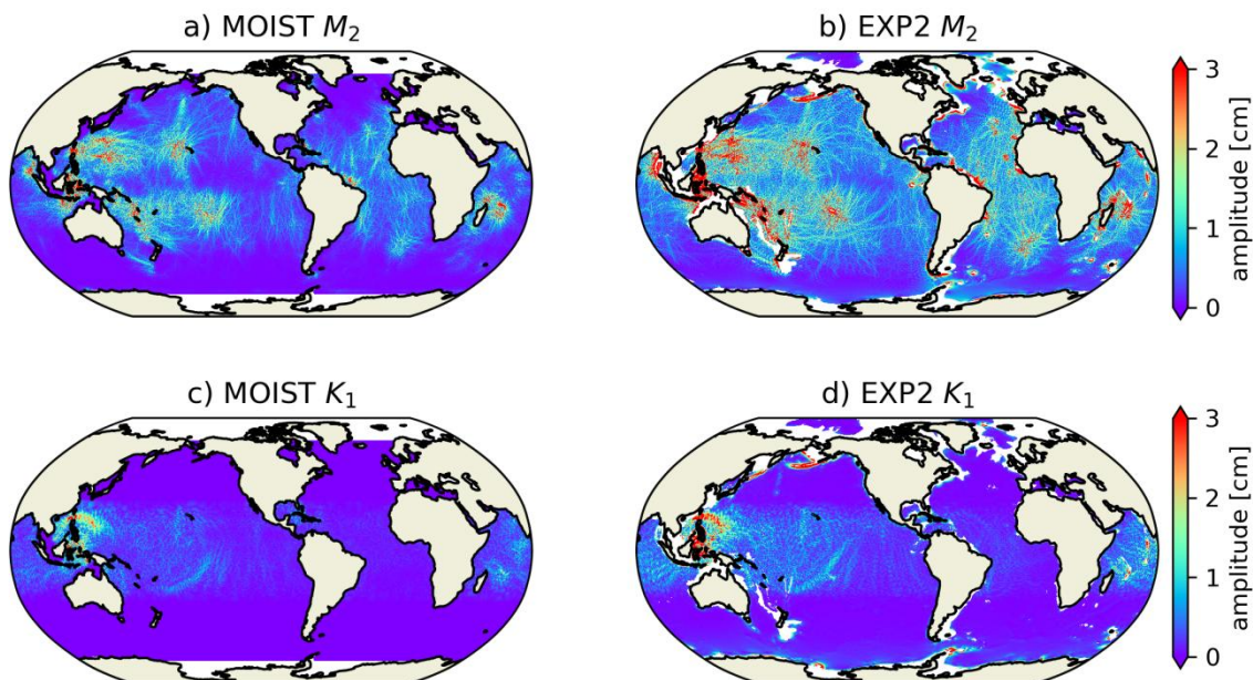
Figure 13 M_2 internal tide amplitude at the surface from MOIST (a), EXP2 (b); (c) and (d) are the same as (a) and (b) but for K_1 .
