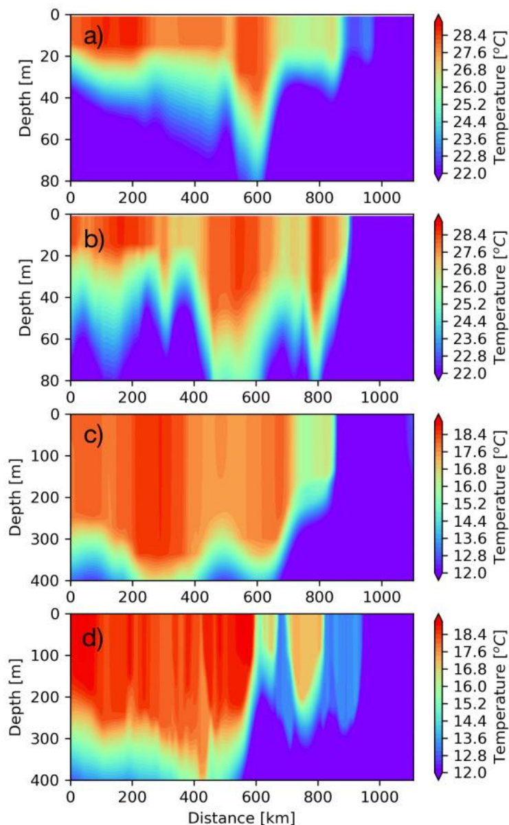
Figure A-4 Temperature along the section in Kuroshio extension region of 1/10^\circ (a, c) and 1/32^\circ (b, d) model during summer (a, b) and winter (c, d) respectively.
