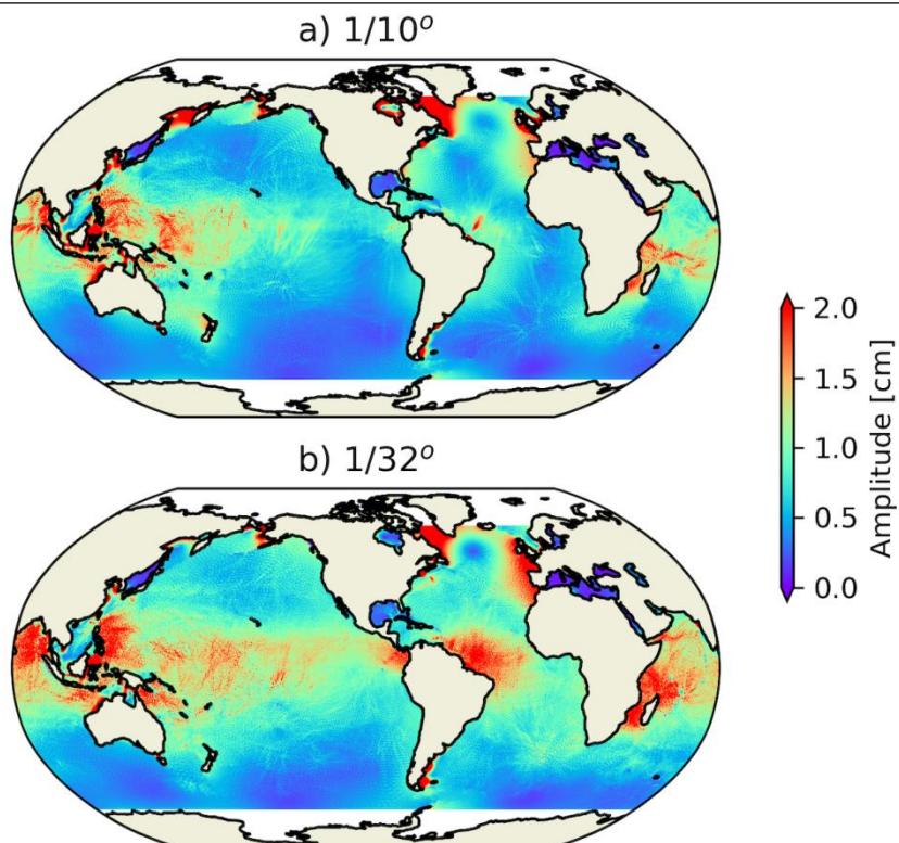
Figure 9 Incoherent tide amplitude of semi-diurnal tidal band of 1/10^\circ (a) and 1/32^\circ (b) model.
