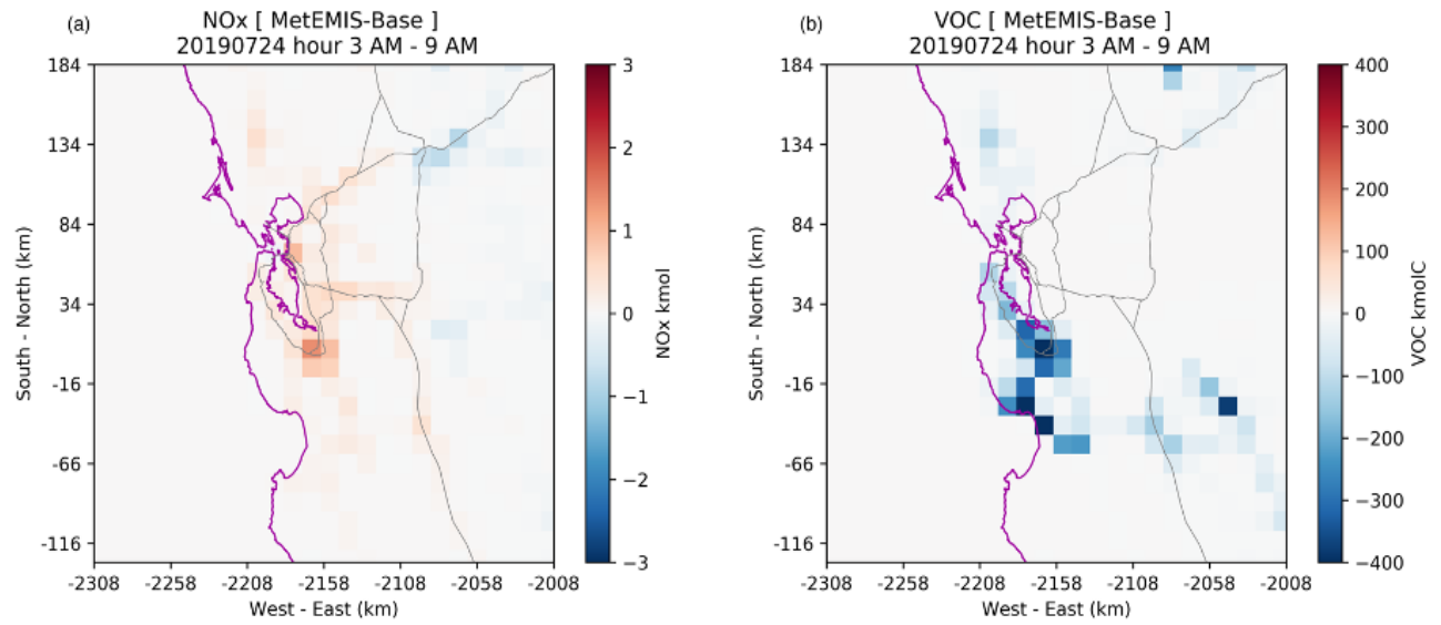
Figure 11. Spatial differences of NOx (a) and VOC (b) emissions from 3LST to 9LST on July 24, 2019 over San Jose, CA.
