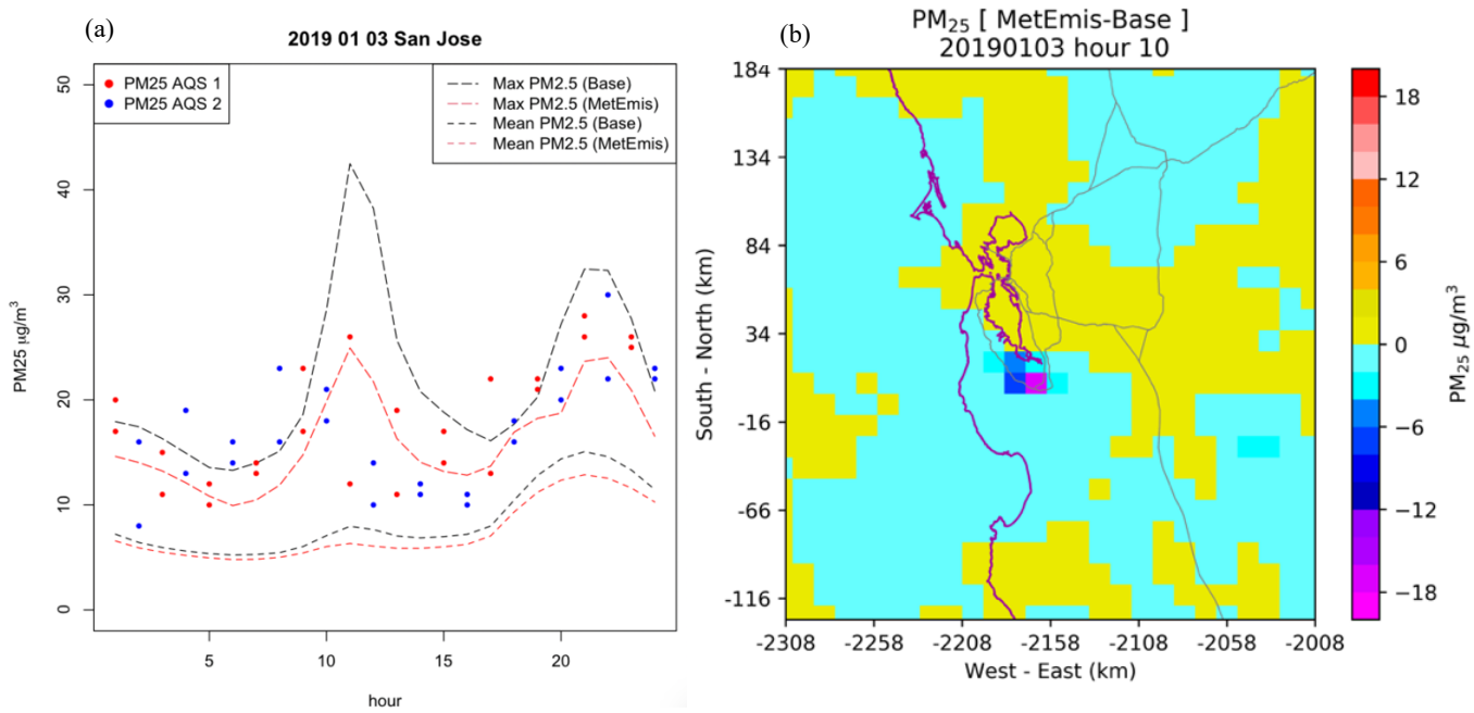
Figure 12. (a)Diurnal variation of PM 2.5 (maximum and mean) concentrations over San Jose targeted region, and (b) the spatial difference of PM 2.5 at 10LST on January 3, 2019.
