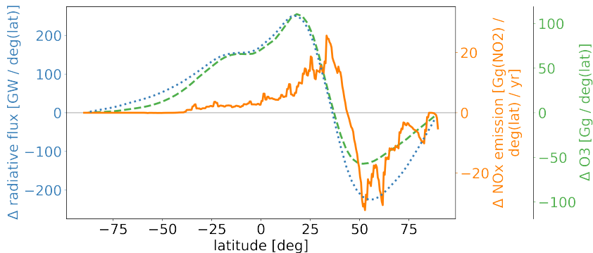
Figure 2. Differences (CMIP5 - CMIP6) of \text{NO}_x emissions (solid orange line), \text{O}_3 burden (dashed green line) and radiative flux (dotted blue line) from two simulations with identical total amount of aviation emissions, but different latitudinal distributions, as a function of latitude.
