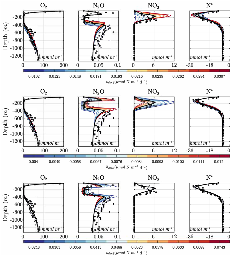
Figure 9. Model sensitivity to parameter values. Panels show changes to O_2 , N_2O , NO_2^- , and N^* for the Opt_{sel} parameter set after varying the maximum NO_3^- , NO_2^- , and N_2O reduction rate parameters ( k_{den1} , k_{den2} , and k_{den3} by \pm 5\% of their Opt_{sel} value in Table B1. Background gray shadings show O_2 concentrations, with horizontal lines highlighting O_2=1 (dotted lines) and O_2=10 (dashed lines)
