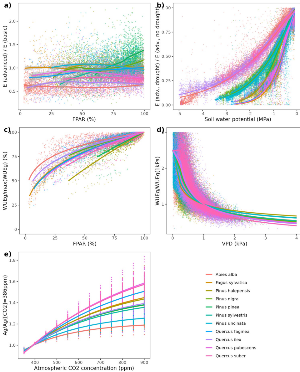
800 Fig. C1. (a) Cohort E_{basic}/E_{advanced} values against their available FPAR ; (b) Ratio of daily E_{advanced} values between simulations 805 with no water supply and simulations with unlimited water supply, as a function of soil water potential in the former case; (c) Annual WUE_g values (relative to the maximum WUE_g value obtained for each plot) against available FPAR ; (d) Daily WUE_g values (relative to WUE_g at VPD = 1kPa ) against VPD ; (e) Plot-level ratios between gross photosynthesis under increasing [CO 2 ] values and gross photosynthesis under [CO 2 ] = 386 ppm. Lines of panel (a) correspond to smoothed splines, whereas those of panels (b-e) indicate the non-linear models fitted for each species.
