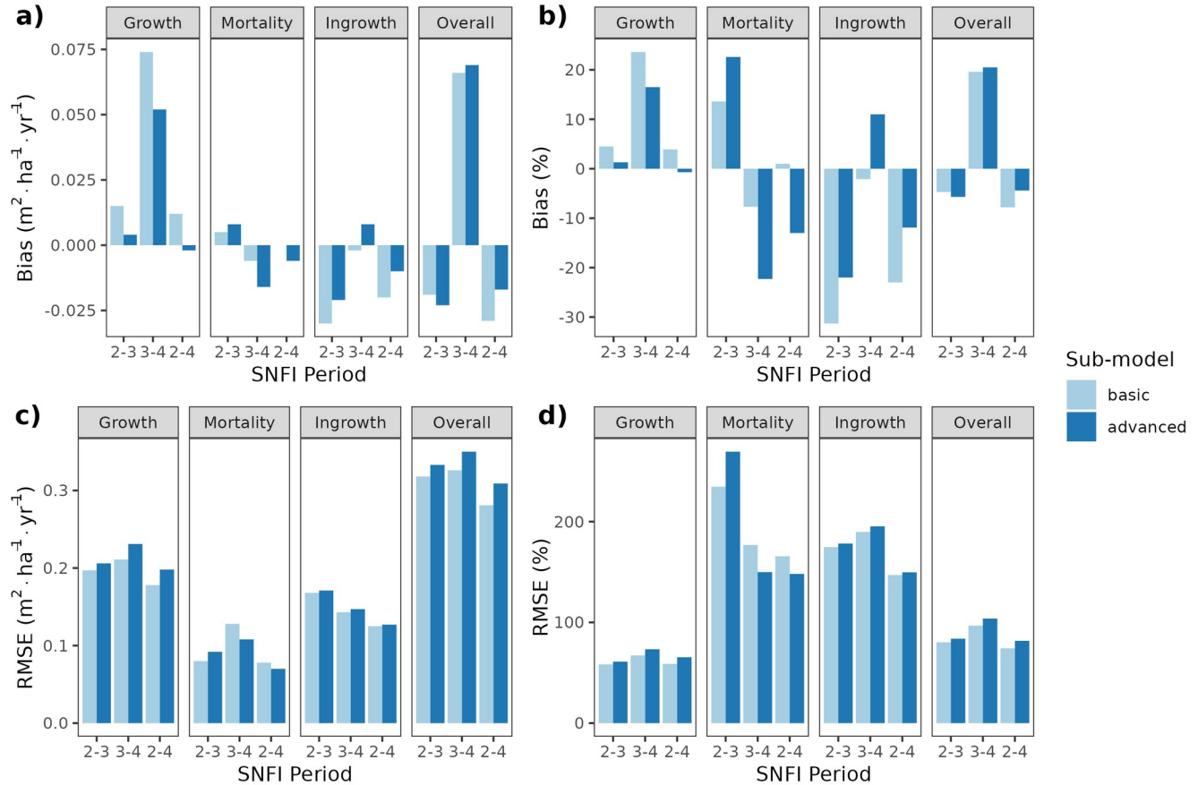
460 Fig. 3: Model evaluation results with respect to annual rates of basal area (BA) changes ( \text{m}^2 \cdot \text{ha}^{-1} \cdot \text{yr}^{-1} ) predicted for different processes (growth, mortality, ingrowth) and taking into account all of them (overall). Results are shown for the two sub- models and for simulations spanning different periods between forest inventory surveys (SNFI2-3, SNFI3-4 and SNFI2-4). Note that calibration of growth, mortality and recruitment parameters was performed using data for the SNFI2-3 and SNFI3- 4 periods. Fig. A5 shows model evaluation results for the SNFI2-3 and SNFI3-4 periods with parameters calibrated using 465 data from a different period.
