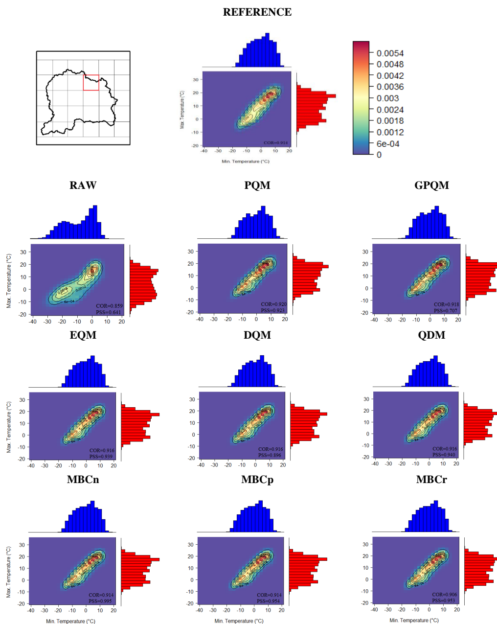
Figure 2: Two-dimensional kernel density plots for the highlighted grid box (red box). Blue histograms (and X-axis) refer to minimum temperature and red histograms (and Y-axis) refer to maximum temperature. Shadings represent the 2-D density distribution for the reference, raw and eight BC methods. Contour lines represent the probabilities in the reference dataset, which are overlaid on the model probabilities for the sake of comparison. COR depicts the Pearson correlation coefficient between daily minimum and maximum temperatures and PSS represents the two-dimensional Perkins skill score of distributional similarity.
