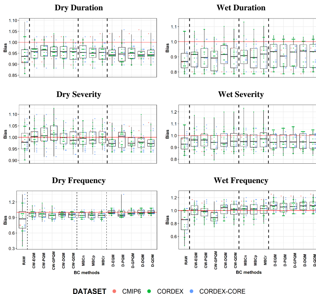
10 Figure 5: Biases (as a ratio of model to reference) in spatially averaged SPEI indices over Upper Jhelum Basin computed from the raw (first box in each panel) and bias corrected data (rest of boxes; CW: component-wise, D: direct). Each box represents the interquartile range of biases across all models, which are depicted individually with colored dots (CMIP6 in red, CORDEX in green, CORDEX-CORE in blue), whiskers expand the full range of biases. Red horizontal lines depict perfect performance, for reference.
