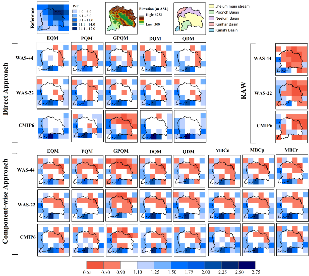
Figure S5: Same as figure S2, but for absolute wet frequency (WF) expressed as total number of wet events.
