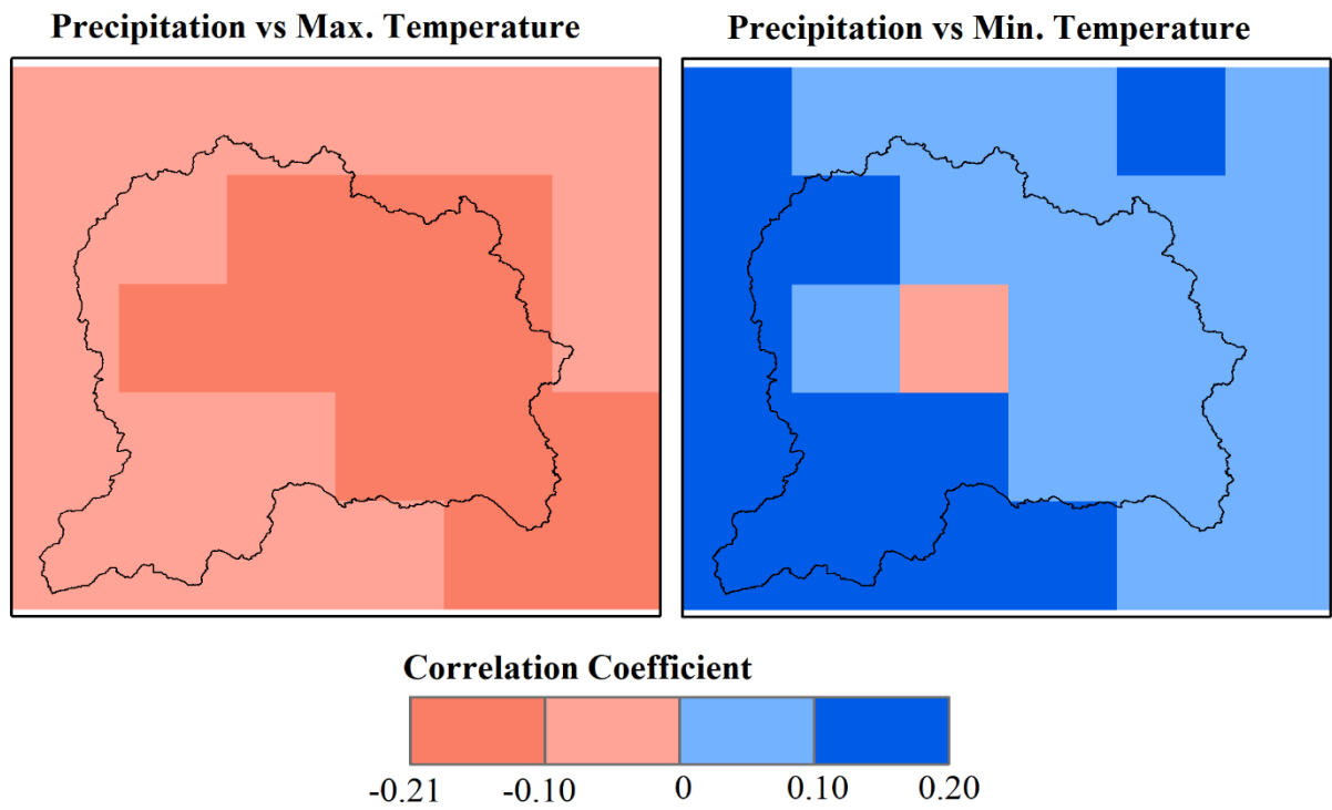
Figure S1: Spearman correlation coefficient between precipitation and maximum temperature (left panel) and precipitation and minimum temperature (right panel) for the reference data.
