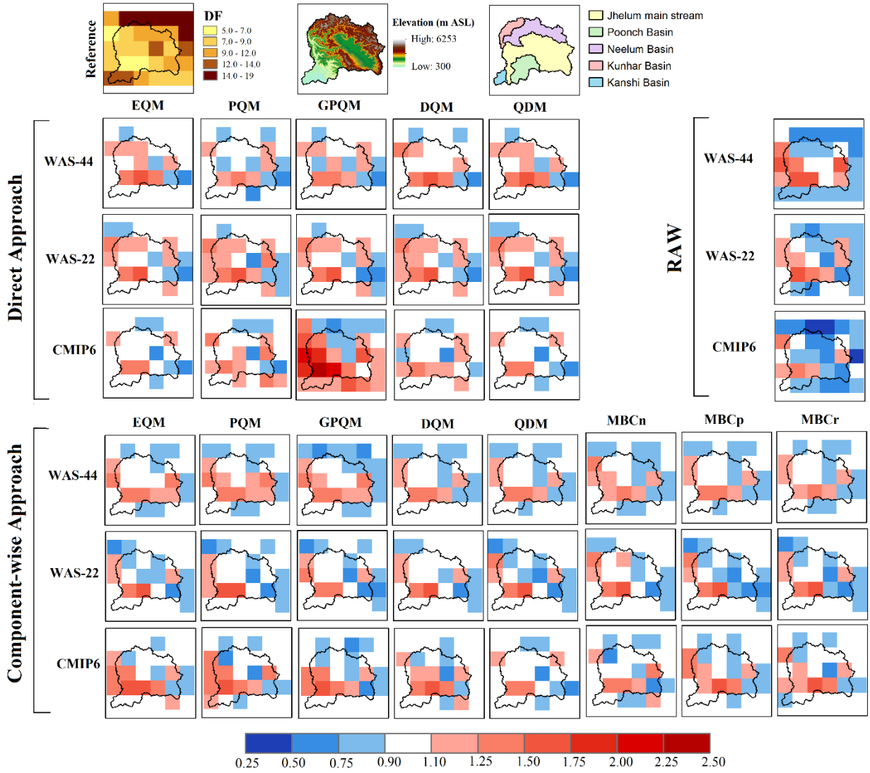
Figure S4: Same as figure S2, but for absolute dry frequency (DF) expressed as total number of dry events.
