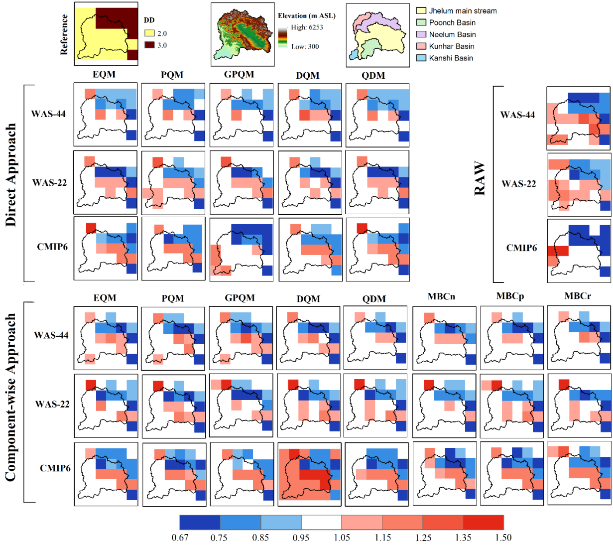
Figure S2: Median dry duration (DD) expressed in months in the reference dataset (first row, left), digital elevation model in meter above sea level (first row, center) and location of sub-basins (first row, right), and biases (as a ratio of model to reference) for the multi-model raw ensembles and bias-corrected ensembles, for the two bias correction approaches and all methods (columns).
