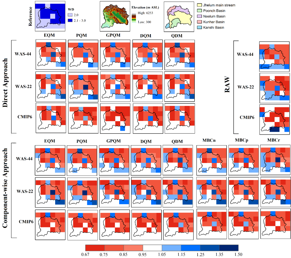
Figure S3: Same as figure S2, but for median wet duration (WD) expressed in months.
