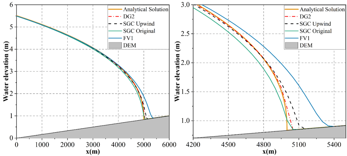
Figure 3: The water elevation profile calculated by the four solvers (dg2, fv1, original SGC and improved SGC) under n=0.06m^{-1/3}s at t=5000s and an enlarged view at the waterfront.
