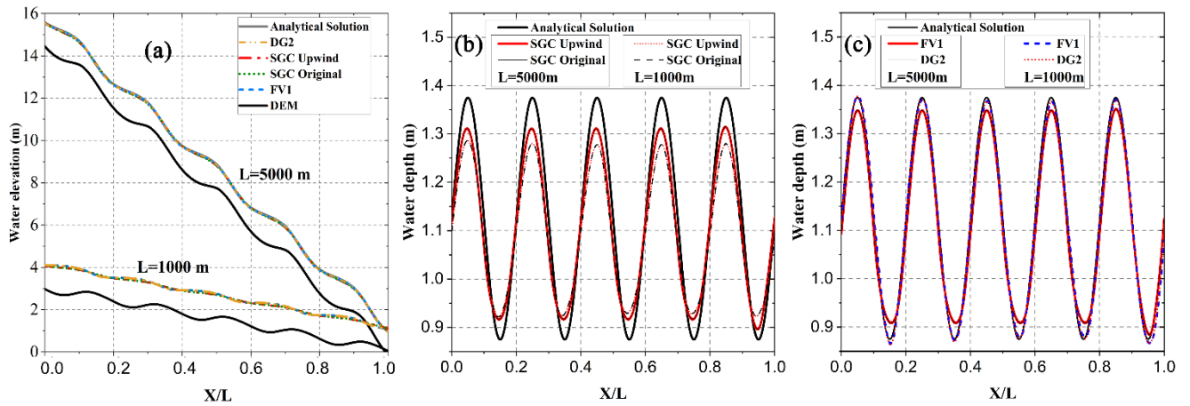
475 Figure 6: Water depth profile predicted by four solvers under L=1000\text{m} and L=5000\text{m} . (a) water elevation and the river channel bed elevation profiles. (b) water depth predicted by two SGC solvers under different oscillating frequency. (c) water depth predicted by the fv1/dg2 solvers.
