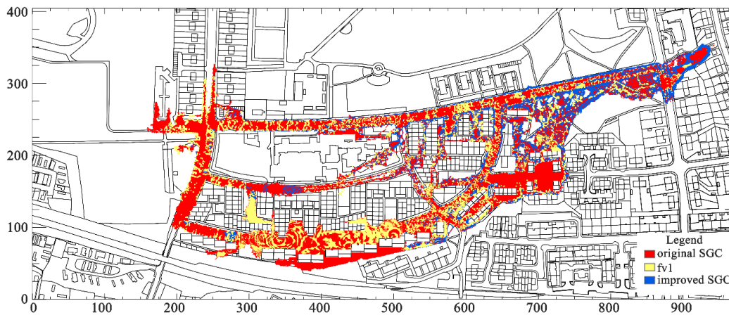
535 Figure 8: Maximum water elevation difference out of the fv1 and SGC solvers compared with dg2. Background vector data are © Ordnance Survey OpenData.
