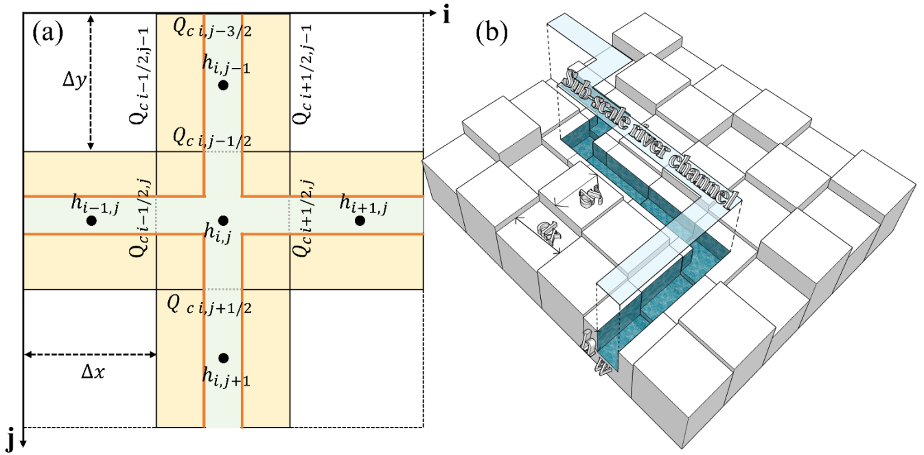
215 Figure 1: Sub-scale representation of the river channel on a coarse resolution DEM. Subgrid cells are in shaded colour, with the black line showing the boundary of the DEM cells. Green shadow represents the river channel, while the yellow shadow represents the floodplain proportion with a subgrid cell. (a) a channel network with the river confluence. (b) a perspective view of a sub-scale river channel on the DEM grid.
