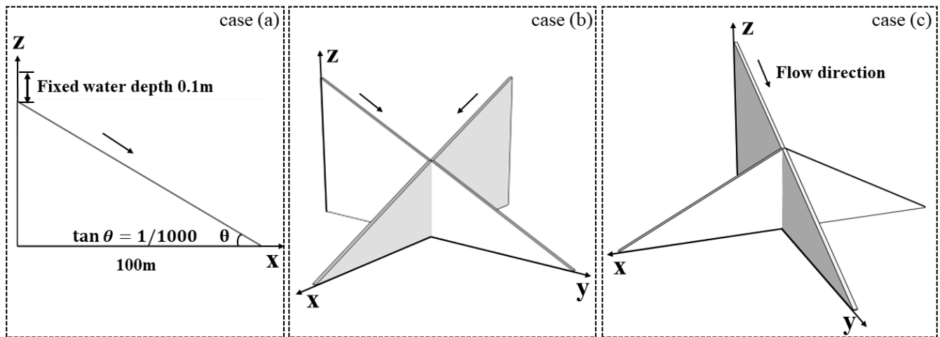
Figure 4: Validation of the new solution strategy at a river junction with different arrangements of a sloping rectangular river channel. (a) a single river channel. (b) two identical sloping channels intersecting at a junction cell. (c) a main stream provides flow for three same downstream channels.
