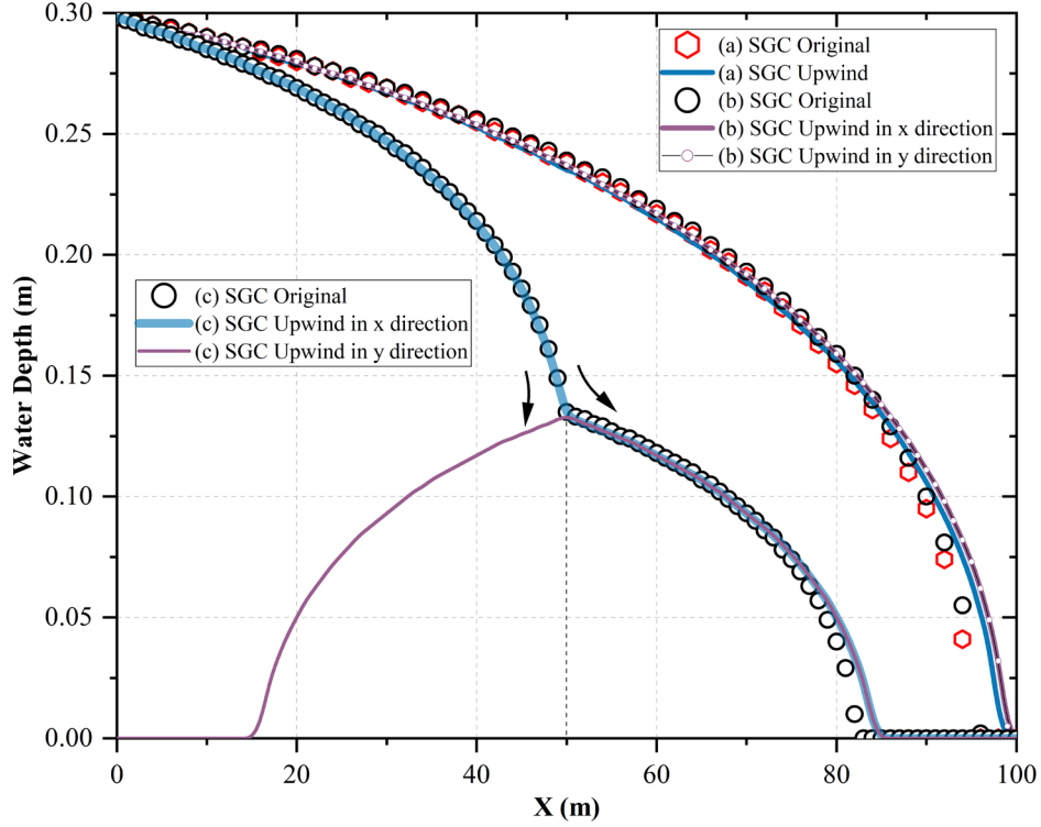
430 Figure 5: Water depth profile predicted by the two SGC solvers at t=131s . Group (a) shows the water depth predicted by a single sloping river channel, and (b) is the 2 channels intersecting at a confluence, and (c) shows the flow distribution from a main stream to three downstream channels.
