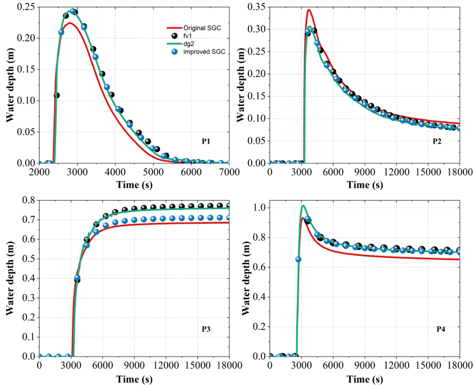
560 Figure 9: Time-series of water depth variation in four locations P1-P4 (locations of P1-P4 are shown in Figure 7).
