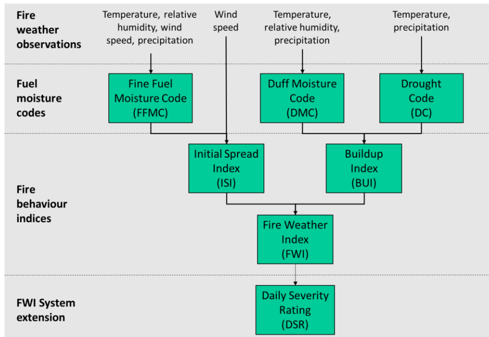
Figure 1: Fire weather components of the Canadian Fire Weather Index (FWI) System. Adapted from Natural Resources Canada (2021).
