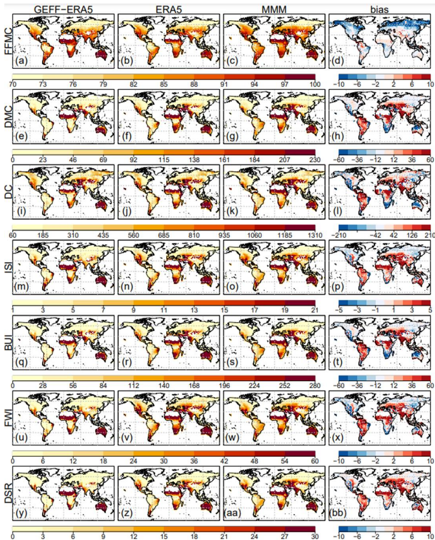
Figure 3: Annually-averaged values of monthly climatology of the 90 th percentile for GEFF-ERA5 (first column), ERA5 (second column) and the CIP6 multi-model mean (third column), and bias in the CIP6 multi-model mean with respect to ERA5 (fourth column) for FFMC (a-d), DMC (e-h), DC (i-l), ISI (m-p), BUI (q-t), FWI (u-x) and DSR (y-bb). Lighter yellow colour represents lower danger and darker brown represents higher danger. Meanwhile, white colour represents lower bias and darker blue/red higher negative/positive bias.
