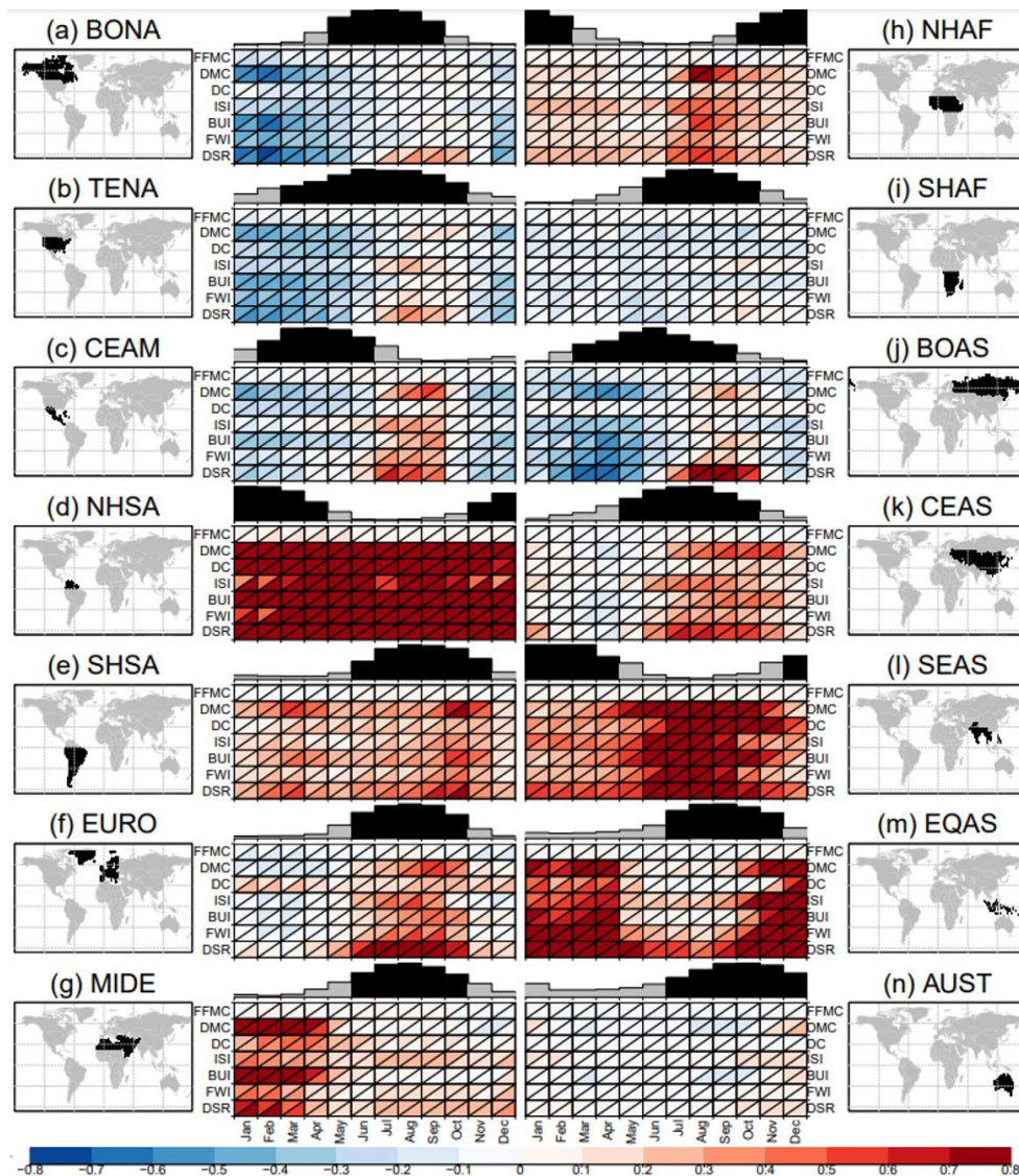
Figure 4: Bias in monthly means and 90 th percentiles in seven CFWIS components simulated by the CMIP6 multi-model mean with respect to ERA5 across 14 GFED fire regions: (a) Boreal North America (BONA); (b) Temperate North America (TENA); (c) Central America (CEAM); (d) Northern Hemisphere South America (NHSA); (e) Southern Hemisphere South America (SHSA); (f) Europe (EURO); (g) Middle East (MIDE); (h) Northern Hemisphere Africa (NHAF); (i) Southern Hemisphere Africa (SHAF); (j) Boreal Asia (BOAS); (k) Central Asia (CEAS); (l) Southeast Asia (SEAS); (m) Equatorial Asia (EQAS); (n) Australia and New Zealand (AUST). Results show overall model performance, with blue shading indicating underestimation and red shading overestimation. The lower right triangle represents the monthly mean and the upper left triangle the monthly 90 th percentile. Bar plots show the average monthly-burned area for each GFED region, represented as a fraction of the monthly maximum. Black bars highlight months that constitute the ‘fire season’, defined as those months for which the average burned area is greater than 50% of the monthly maximum.
