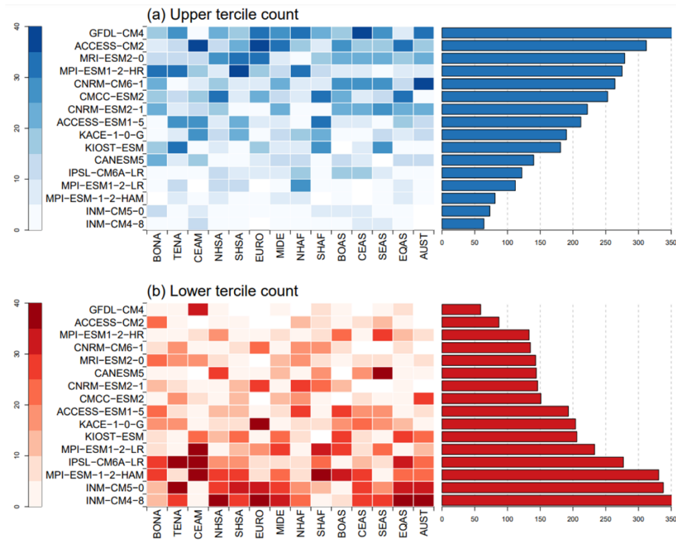
Figure 9: (a) Counts of the number of times that each CMIP6 model is ranked in the upper tercile (top 5) across all 7 CFWIS components and 3 x 2 skill metrics (correlation, RMSE, and ratio of standard deviation for the mean and 90 th percentile). The grid (left) shows the breakdown of total counts for each of the 14 GFED regions. The bars (right) indicate the total count across all regions. (b) As (a) but for the lower tercile (bottom 5).
