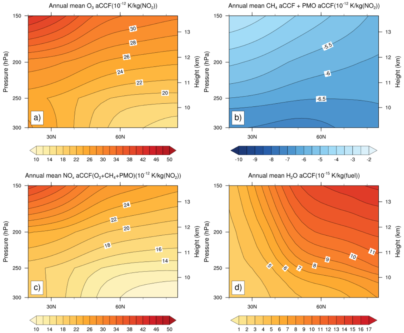
385 Figure 7 Annual zonal mean aCCFs (F-ATR20) in the northern hemisphere and the between 150 to 300 hPa attributed to a) \text{NO}_x - \text{O}_3 effects; b) \text{NO}_x - \text{CH}_4 (+PMO) effects; c) overall \text{NO}_x effects ( \text{O}_3 + \text{CH}_4 +PMO); d) \text{H}_2\text{O} effects
