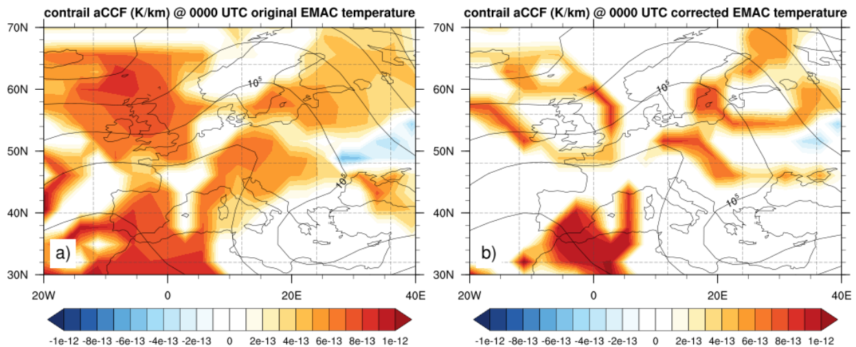
550 Figure 13 Geographical distribution of contrail aCCF in K/km on 18 th December 2015 at 250 hPa for a) the original EMAC temperature and b) the bias-corrected EMAC temperature.
