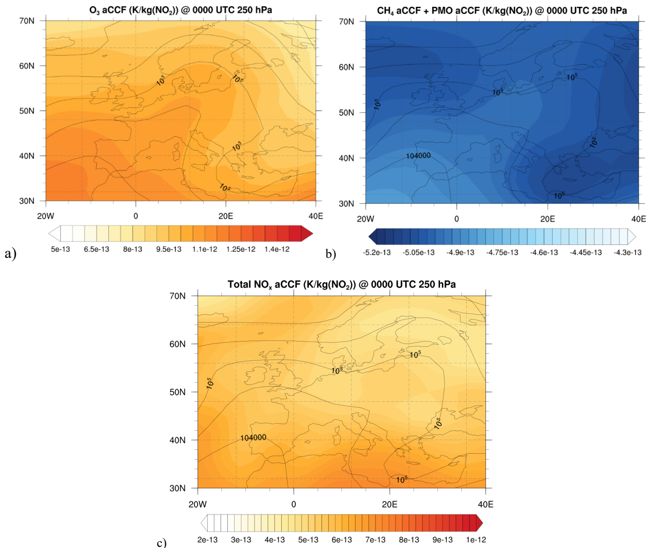
Figure 4 NO x aCCF in K/kg(NO 2 ) on December 18 th 2015 at 250 hPa for: a) O 3 -aCCF; b) the combined CH 4 -aCCF and PMO-aCCF and c) the total NO x aCCF (O 3 -aCCF + CH 4 -aCCF + PMO-aCCF). The black contour lines are geopotential in m 2 /s 2 .
