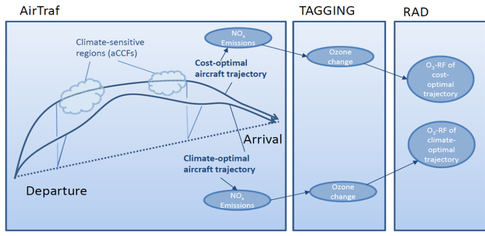
410 Figure 9 Sketch of the radiative forcing calculations for ozone changes caused by online air traffic NO x emissions for cost- and climate-optimized flight trajectories. Cost-optimal aircraft trajectories minimize the simple operating cost of the flight, while, climate-optimal aircraft trajectories minimize the climate impact (here only the NO x -induced O 3 effect is included).
