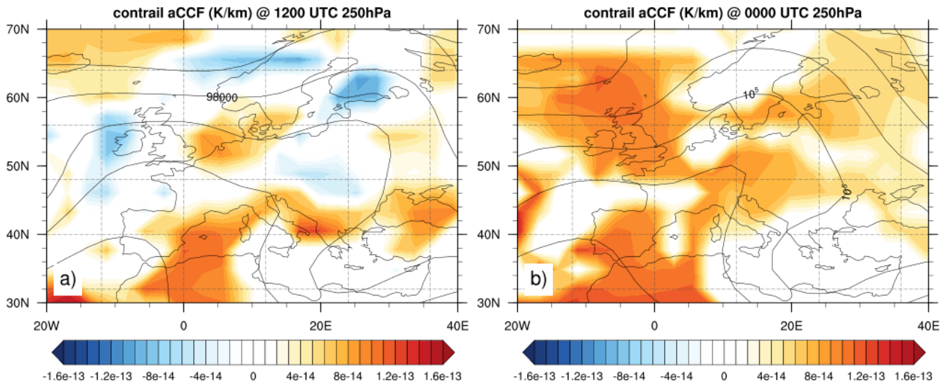
325 Figure 6 Contrail-cirrus aCCFs (colored contour) in K/km and geopotential height (black contour) in m 2 /s 2 on December 18 th 2015 at 250 hPa: a) 1200 UTC; b) 0000 UTC.
