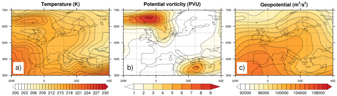
Figure 3 Geographical distribution of a) Temperature (K); b) Potential Vorticity in standard potential vorticity unit (PVU, 1 \text{ PVU} = 10^{-6} \text{ K m}^2 \text{ kg}^{-1} \text{ s}^{-1} ); c) Geopotential ( \text{m}^2/\text{s}^2 ) over Europe at 250 hPa on December 18 th 2015.
