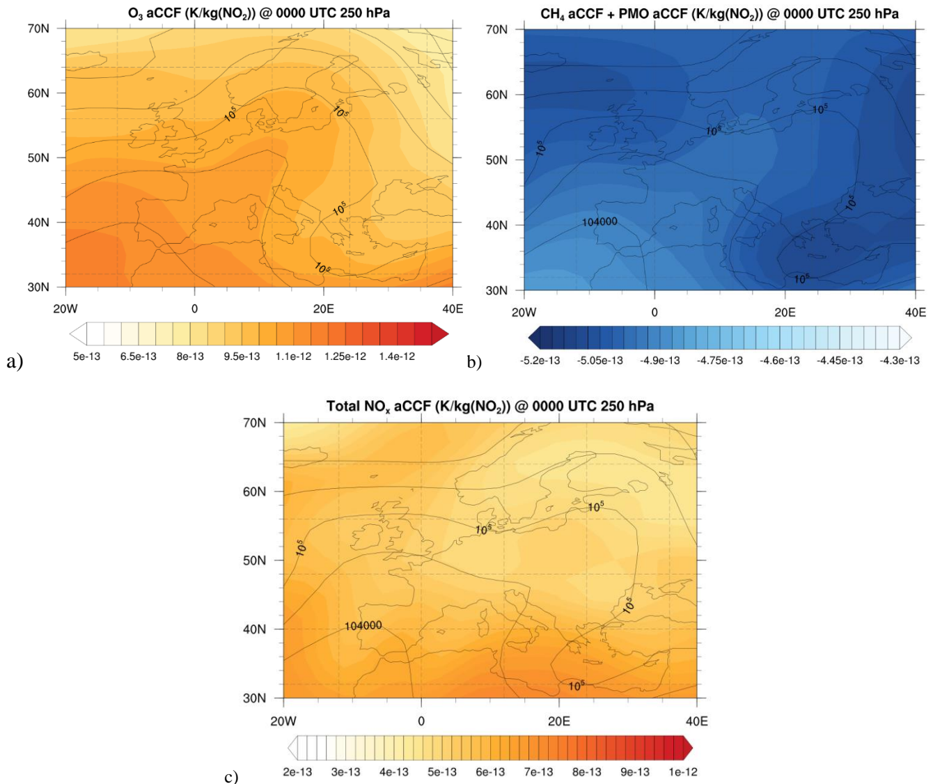
Figure 4 \text{NO}_x aCCF in \text{K/kg}(\text{NO}_2) on December 18 th 2015 at 250 hPa for: a) \text{O}_3 -aCCF; b) the combined \text{CH}_4 -aCCF and PMO-aCCF and c) the total \text{NO}_x aCCF ( \text{O}_3 -aCCF + \text{CH}_4 -aCCF + PMO-aCCF). The black contour lines are geopotential in \text{m}^2/\text{s}^2 .
