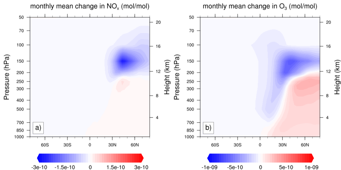
455 Figure 11 Changes of a) NO x mixing ratio and b) resulting changes in O 3 mixing ratio caused by NO x -O 3 -optimized flight trajectories using only O 3 aCCF. The baseline is cost-optimized flights.
