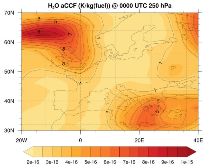
275 Figure 5 H 2 O aCCF (colored contour) in K/kg(fuel) and potential vorticity (black contour) in standard potential vorticity unit (PVU) on December 18 th 2015, at 250 hPa.
