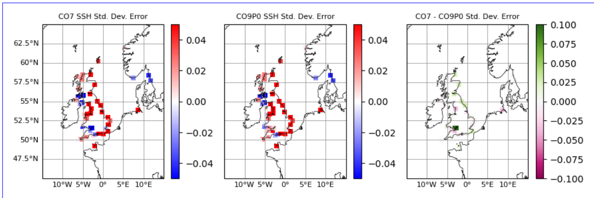
Figure 4. Errors in Total Water Level standard deviations, calculated over the 10 year model run for the CO7 and CO9p0 configurations. The two panels on the left show the errors for the CO7 and CO9p0 configurations.
