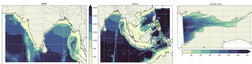
Figure 2. Bathymetry (m) from South East Asia, South Asia and Severn Estuary worked example configurations.
