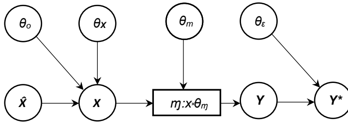
Figure 1: A configuration of a network coupling some elements in \mathcal{M}, \mathbf{X}, \boldsymbol{\theta}, \mathbf{Y}, \mathbf{Y}^*
