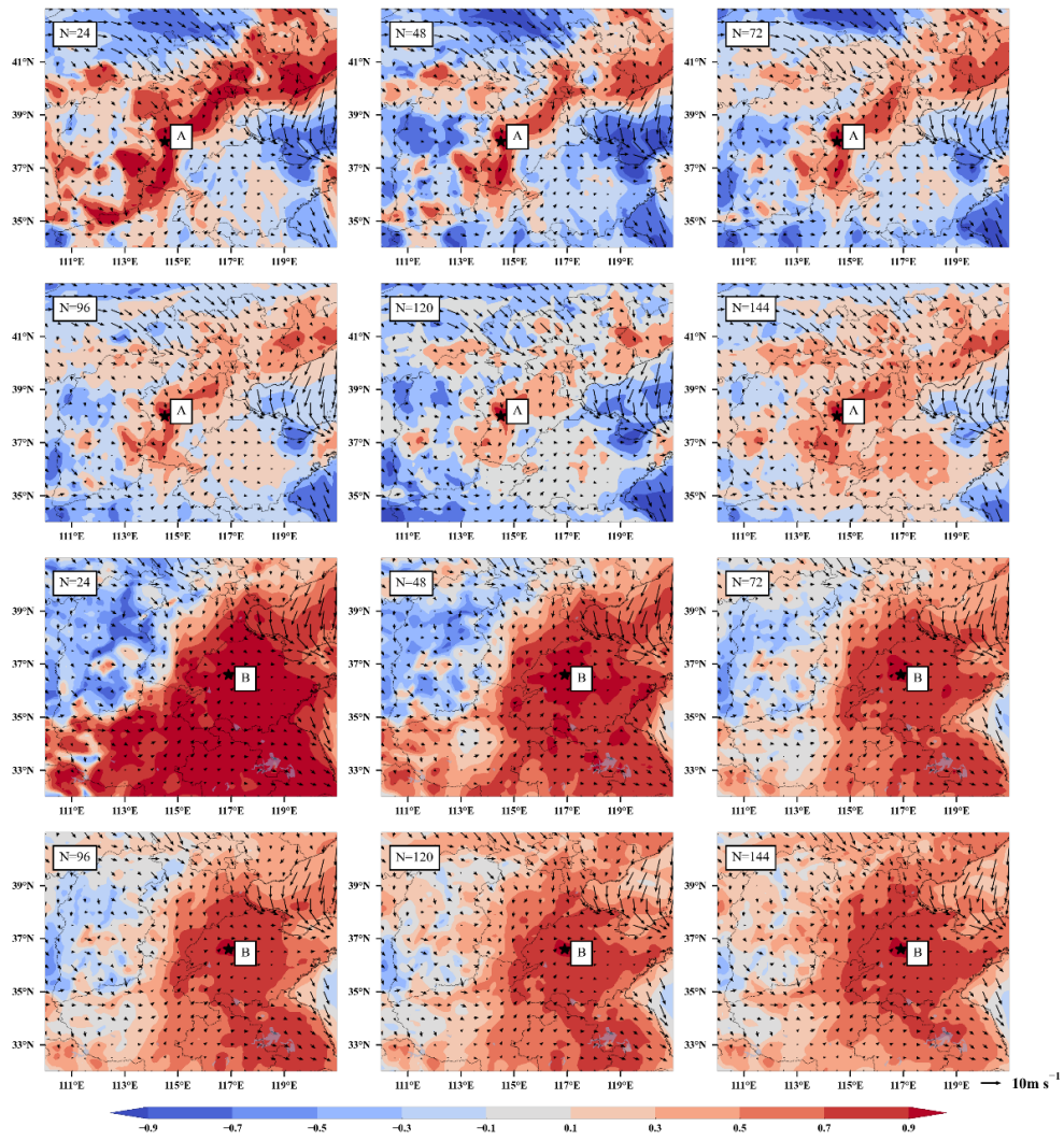
665 Figure 4. Spatial distribution of correlation coefficients of background error for site A (38.0° N, 114.5° E) (rows 1, 2) and site B (36.6° N, 116.9° E) (rows 3, 4) with different ensemble size N of 24, 48, 72, 96, 120, 144 and wind vectors at 0000 UTC on 15 December 2016.
