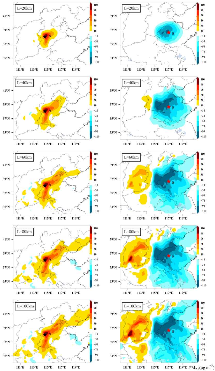
660 Figure 3. Spatial distribution of PM_{2.5} analysis increments after assimilation of initial fields at 0000 UTC on 15 December 2016, for assimilation site A ( 38.0^{\circ} N, 114.5^{\circ} E) only (left column) and assimilation site B ( 36.6^{\circ} N, 116.9^{\circ} E) only (right column) with fixed ensemble size 48 and different localization length-scale of 20, 40, 60, 80, 100 km.
