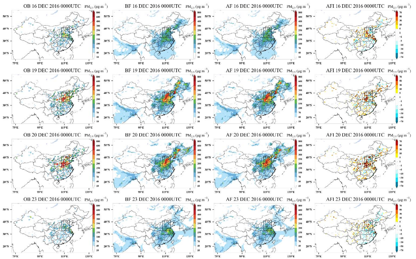
Figure 6. Snapshots of the horizontal distributions of PM_{2.5} observation (OB), before (BF) and after (AF) the application of EnOI technique, analysis field increment (AFI) at 0000 UTC on 16, 19, 20, and 23, December 2016. The black box area, representing North China (NC).
