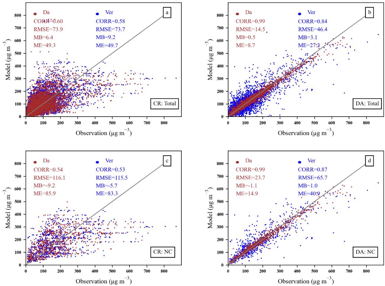
670 Figure 5. Scatter plot of PM 2.5 concentrations from the control experiment (a,c) and the assimilation experiment (b, d). The ensemble size in the assimilation experiment is 96 and the length-scale L is 40 km. Brown (Da) and blue (Ver) dots are assimilation sites and validation sites respectively. a, b is for mainland China (Total), c, d is for North China (NC).
