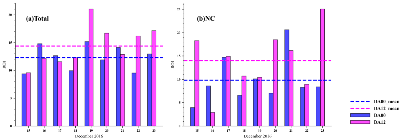
690 Figure 8. Rate of improvement (ROI, unit: %) by data assimilation in 1d (24 h) predictions for 15 to 23 December 2016 over Mainland China (a), North China (b). The ROI is the ratio of the reduced RMSE statistical metrics to those for the CR simulation. DA00 and DA12 represent the initial field assimilation using EnOI at 0000 UTC and 1200 UTC each day, respectively. DA00_mean and DA12_mean represent the mean ROI over 15 to 23 December 2016 of DA00 and DA12, respectively.
