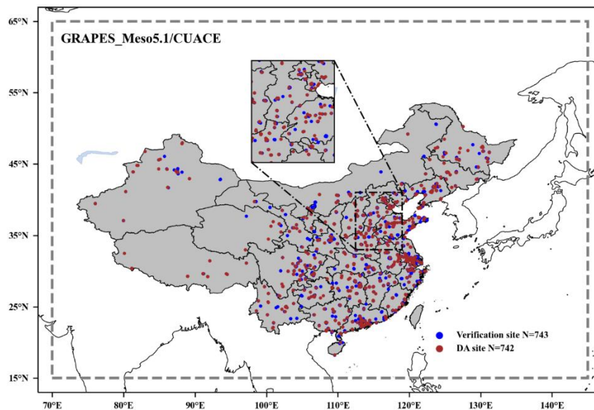
655 Figure 2. Simulation domain of GRAPES_Meso5.1/CUACE. Minor region represents North China (NC). The locations of ground stations in China mainland are marked on the maps with blue and brown dots. The blue and brown dots represent verification sites and assimilation sites, respectively. "N=743" means there are 743 verification sites. "N=742" means there are 742 DA sites.
