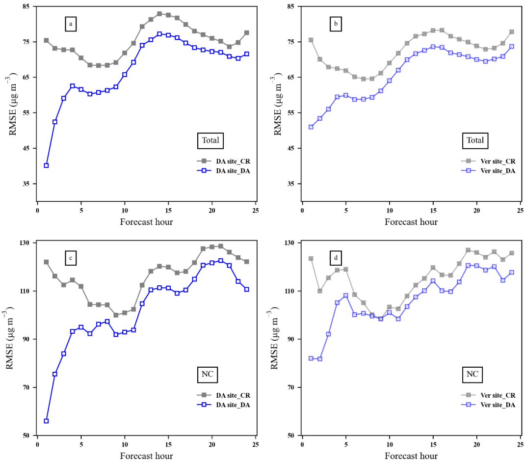
685 Figure 7. The average RMSE value of surface PM 2.5 forecasts as a function of forecast time over (a) China Mainland for DA sites, (b) China Mainland for verification sites, (c) North China for DA sites, (d) North China for verification site.
