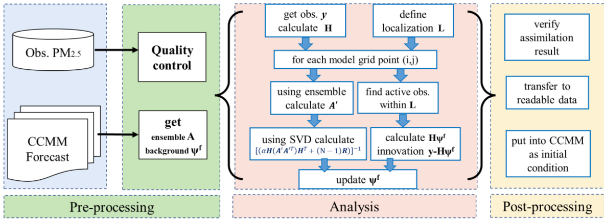
650 Figure 1. Flow chart of the main procedures for EnOI initial field assimilation system. The Obs. PM 2.5 is ground-based observation of PM 2.5 . The CCMM is coupled chemistry meteorology models. SVD is singular value decomposition
