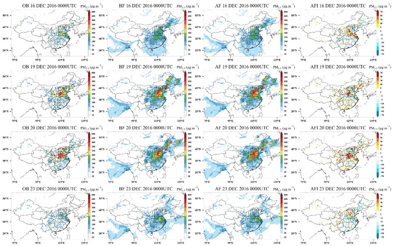
670 Figure 6. Snapshots of the horizontal distributions of PM 2.5 observation (OB), before (BF) and after (AF) the application of EnOI technique, analysis field increment (AFI) at 0000 UTC on 16, 19, 20, and 23, December 2016. The black box area, representing North China (NC).
