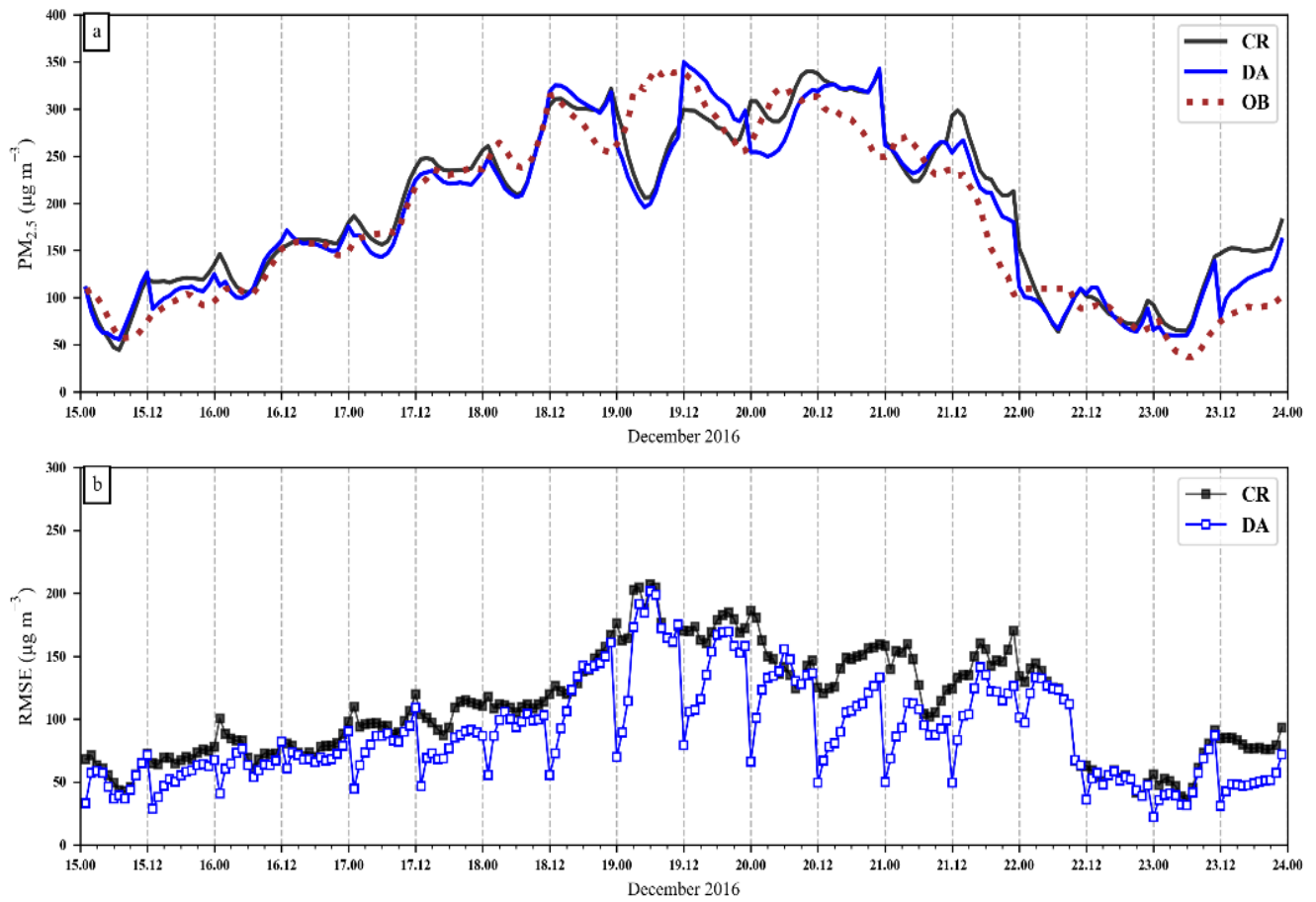
690 Figure 9. Time series of hourly PM_{2.5} concentration (a) and RMSE between forecasts and observations (b) from 15 December to 23 December 2016 in North China. Red dots: observations, black line: forecasts from control experiment (CR), blue line: forecasts from experiment with initial field assimilation at 0000UTC and 1200UTC (DA), black line with dots: RMSE between CR forecasts and observations, blue line with dots: RMSE between CR forecasts and observations. The values are averages calculated against all the observation sites in North China.
