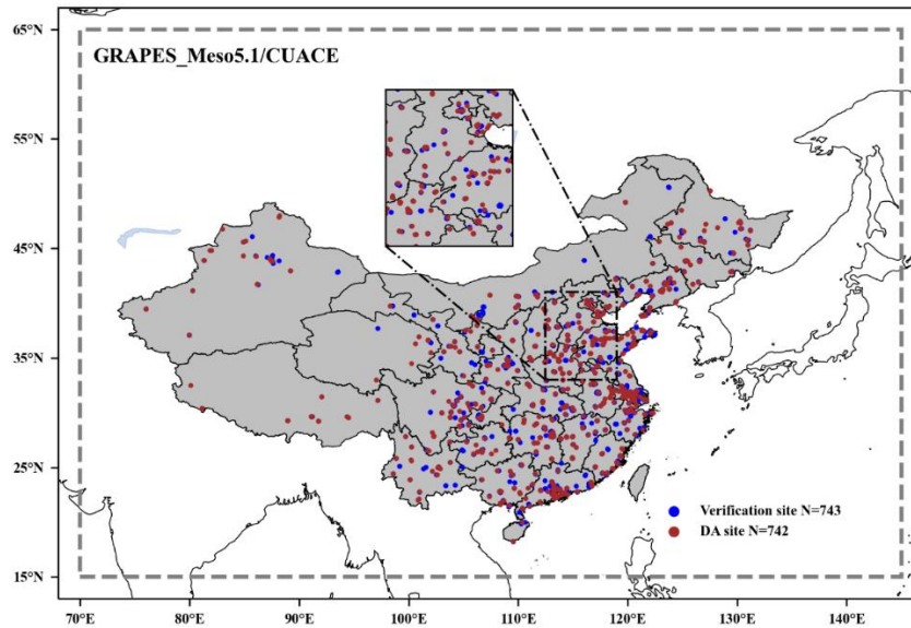
650 Figure 2. Simulation domain of GRAPES_Meso5.1/CUACE. Minor region represents North China (NC). The locations of ground stations in China mainland are marked on the maps with blue and brown dots. The blue and brown dots represent verification sites and assimilation sites, respectively. "N=743" means there are 743 verification sites. "N=742" means there are 742 DA sites.
