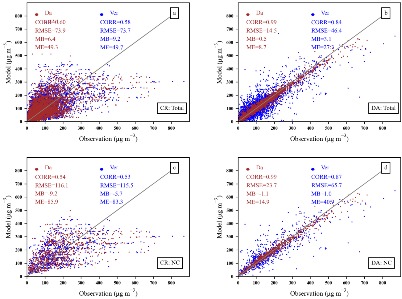
665 Figure 5. Scatter plot of PM 2.5 concentrations from the control experiment (a,c) and the assimilation experiment (b, d). The ensemble size in the assimilation experiment is 96 and the length-scale L is 40 km. Brown (Da) and blue (Ver) dots are assimilation sites and validation sites respectively. a, b is for mainland China (Total), c, d is for North China (NC).
