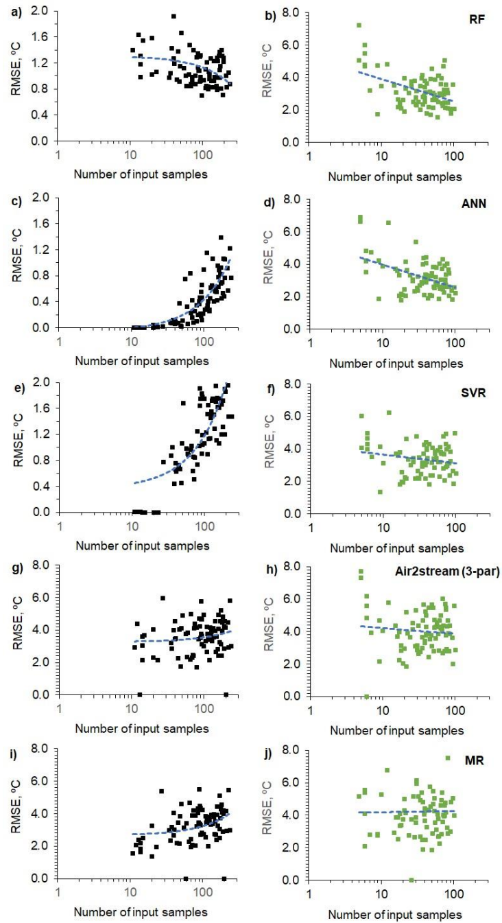
Figure 46: Root-mean-square error between observed and predicted WT values obtained with all models during the training (black dots) and validation-testing (green dots) phases, ordered by the number of values in the training and validation-testing datasets (from smallest to largest)
