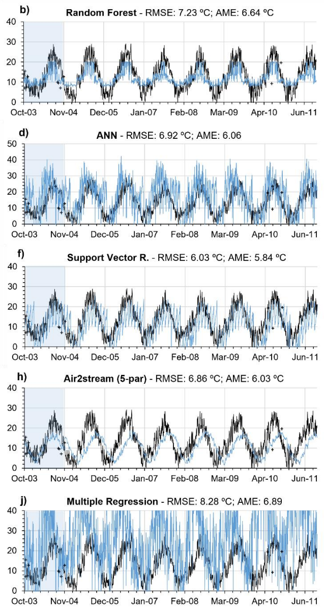
Figure 57: Root-mean-square error between observed (black dots) and predicted WT (Blue line) values obtained during the calibration (blue shadow area) and validation-testing phase (white shadow area) with all models for Station 59 (graphs on left) and Station 2 (graphs on right). Air temperature (black line)
