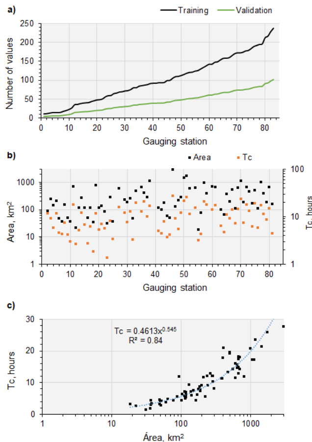
570 Figure 68: a) Number of training and validation-testing datasets of each station. b) Watershed time of concentration and area of each station. c) Watershed time of concentration versus watershed area
