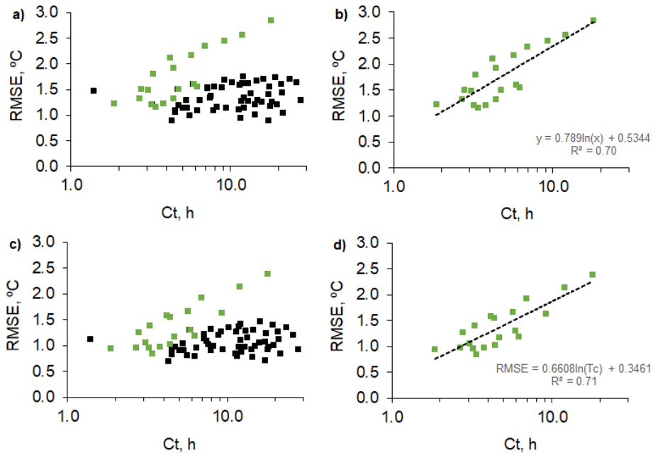
Figure 79: a) RMSE between observed and simulated river WT with the Random Forest best model run versus the watershed time of concentration. b) Data extraction from a). c) RMSE between observed and simulated river WT with the Random Forest ensemble aggregation approach versus the watershed time of concentration. d) Data extraction from c)
