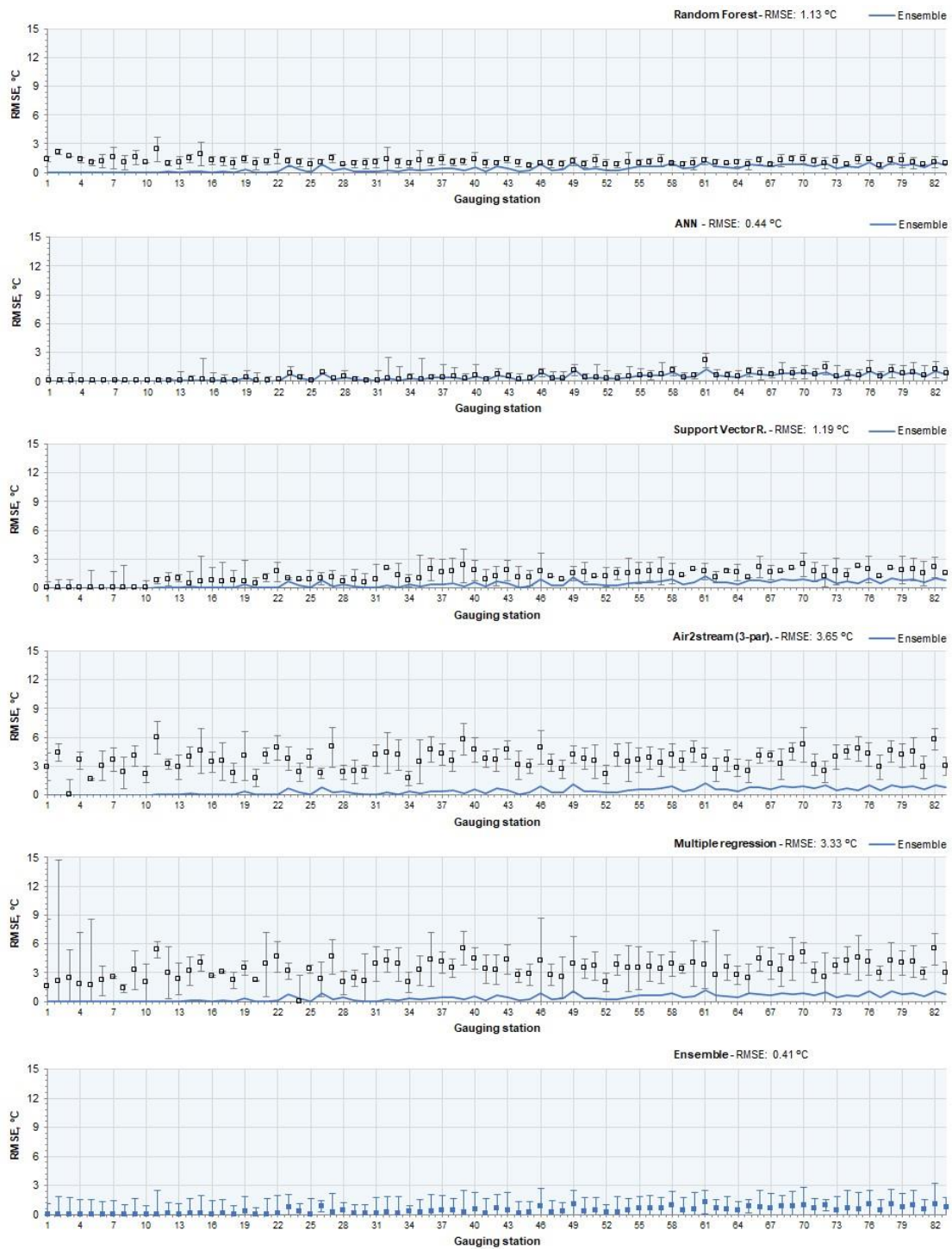
Figure 24: Root-mean-square error between observed and predicted WT values obtained during the training phase with all models (with standard deviation of interannual RMSE), considering the model results and the ensemble of all models results. Stations are ordered by the number of training dataset values, from smallest to largest
