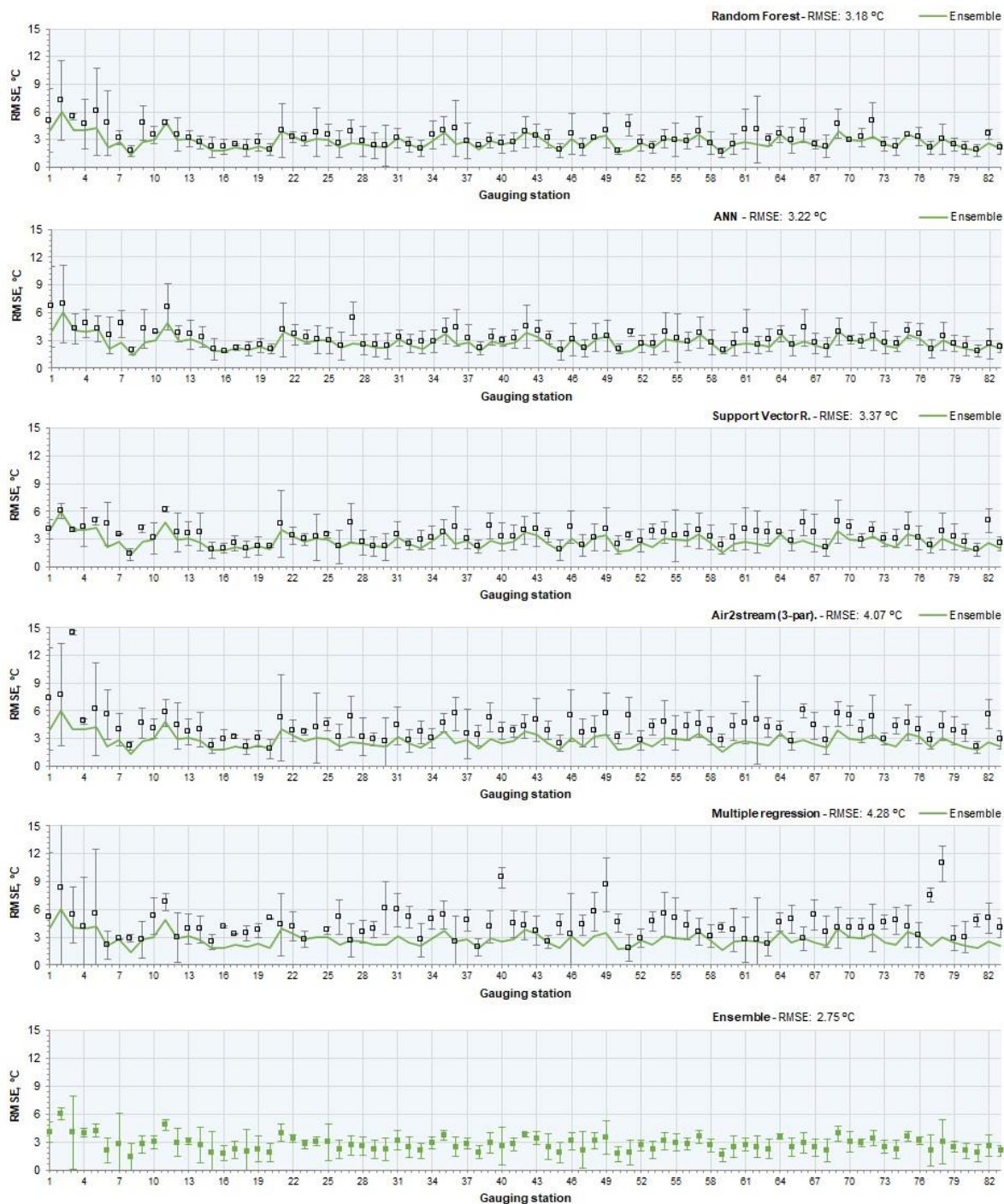
Figure 35: Root-mean-square error between observed and predicted WT values obtained during the validation-testing phase with all models (with standard deviation of interannual RMSE), considering the model results and the ensemble of all models results. Stations are ordered by the number of validation-testing dataset values, from smallest to largest
