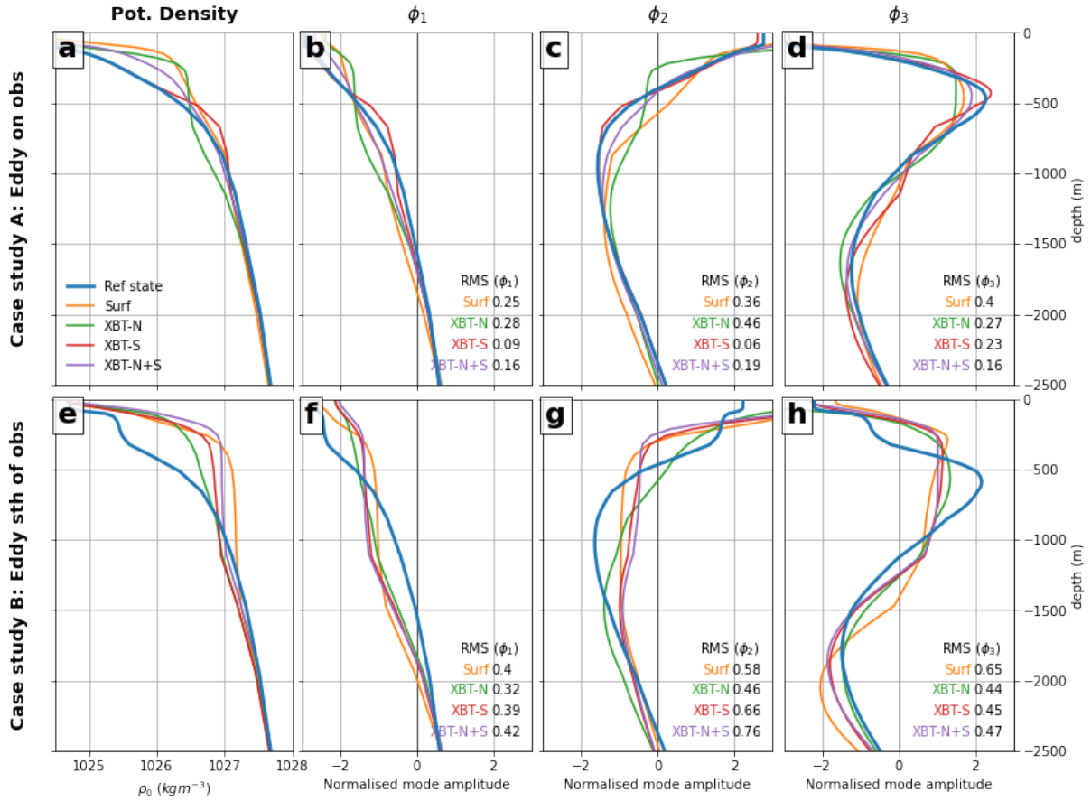
Figure 9. For case study A, the (a) potential density profile is shown for each OSSE, and the amplitude of the baroclinic modes (b) \phi_1 , (c) \phi_2 and (d) \phi_3 are shown for the Ref state, each OSSE. For case study B, the (e) potential density profile, and baroclinic modes (f) \phi_1 , (g) \phi_2 and (h) \phi_3 are shown for each OSSE. The barotropic mode ( \phi_0 ) is excluded, as by normalisation it has unity value at all depths. Potential densities are referenced to surface pressure. In panels b-d and f-h, we show the RMS difference of the OSSE mode shape compared to that of the Ref state. Note that the vertical axis has been limited to the top 2500 m .
