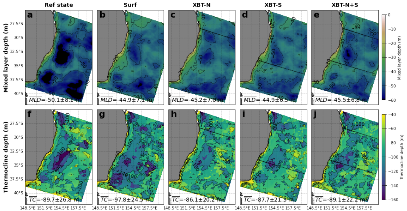
Figure 2. The mean mixed layer depth (first row) is shown for the Ref state (a) and each OSSE (b-e). The mixed layer depth is calculated as the depth at which temperature is 0.5^\circ\text{C} less than the SST. The thermocline depth (second row) is shown for the Ref state (f) and each OSSE (g-j). The thermocline depth is calculated as the depth equal to twice the distance from the bottom of the mixed layer to the depth of maximum change in temperature with depth. \overline{MLD} and \overline{TC} shows the spatial means and standard deviations of the mixed layer and thermocline depth, respectively. The XBT-N and XBT-S transect locations are marked in respective panels. Axes with latitudes are labelled ^\circ\text{S} and axes with longitudes are labelled ^\circ\text{E} .
