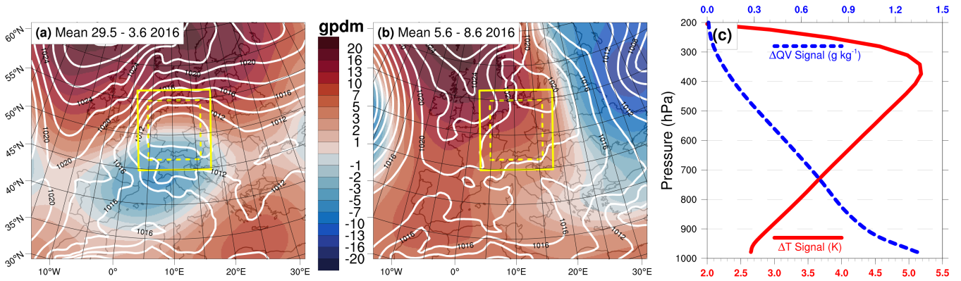
Figure 1. 500 hPa geopotential height anomaly ( gpdm , shading; reference is 1979–2015 mean) and sea level pressure ( hPa , white lines) averaged over the periods (a) 29.5–3.6 and (b) 5.6–8.6, 2016. The maps cover the spatial extent of the 0.11^\circ simulation domain and the solid and dashed yellow lines mark the 0.025^\circ simulation domain and analysis region, respectively. (c) Climate-change signal of temperature and specific humidity added to the initial and boundary conditions of the 0.11^\circ PGW simulations. The signal is computed based on an area average over the 0.11^\circ domain; change profiles for winds and pressure, and equivalent plots on height levels, are presented in Fig. S1.
