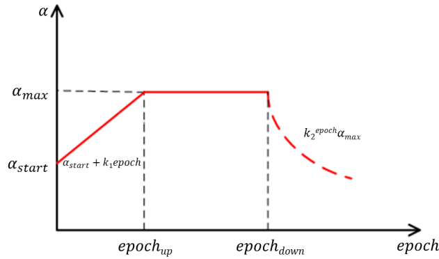
Figure 4. The variable learning rate change line.
