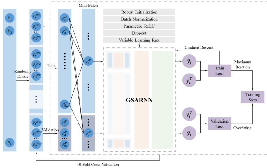
Figure 3. The network training framework of the GSARNN model.
