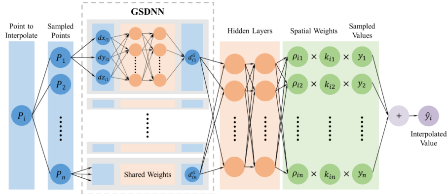
Figure 2. The GSARNN model structure.
