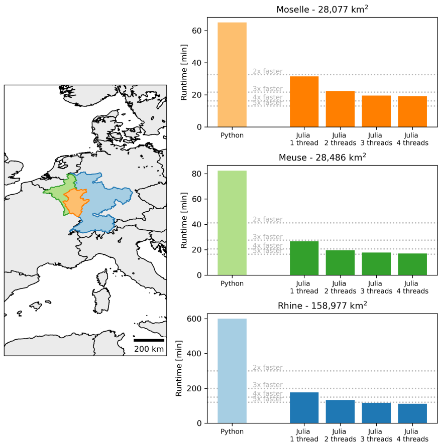
Figure 2. Simulation times of the wflow_sbm model in three large catchments with the wflow Python version 2020.1.2 (Schellekens et al., 2020) and Wflow.jl v0.7.3 (van Verseveld et al., 2024), including multithreading in the Julia version.
