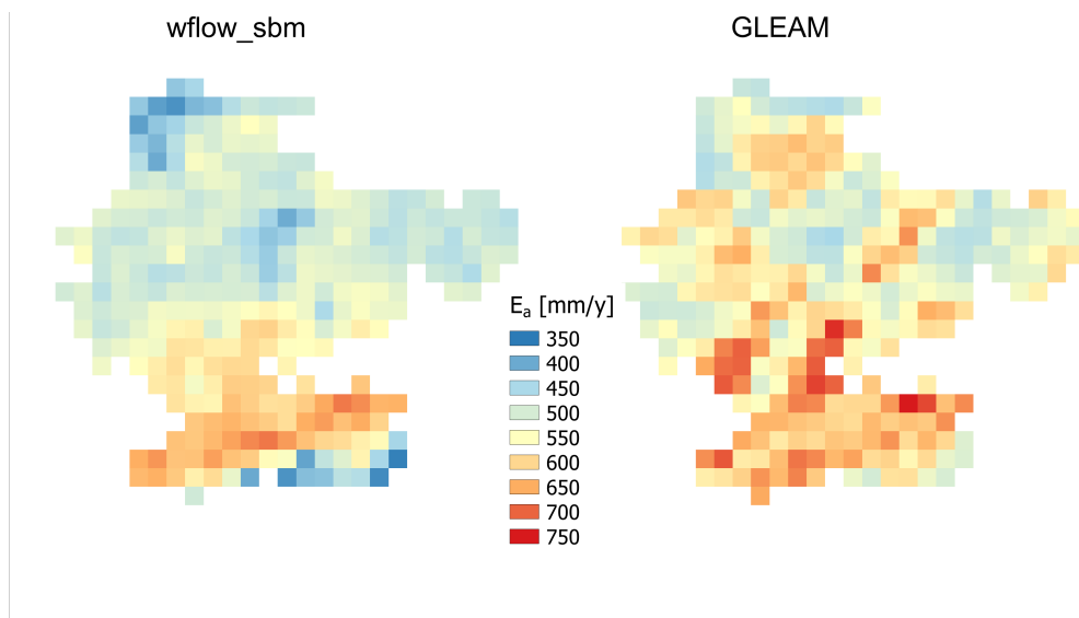
Figure 13. Wflow_sbm simulated and GLEAM long-term (2015-2019) average annual evapotranspiration ( E_a ) for the Rhine catchment.
