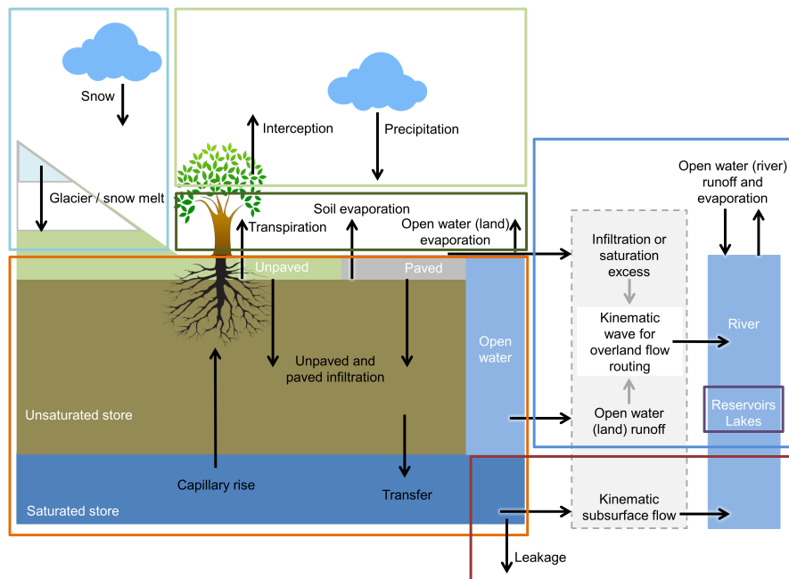
Figure 1. An overview of the different processes and fluxes in the wflow_sbm model (adopted from van Verseveld et al., 2024). The model includes the following routines: Interception (green, section 2.2), Snow and glaciers (light blue, section 2.3), Soil module and evapotranspiration (orange, section 2.4), Lateral subsurface flow (brown, section 2.5), Surface routing (dark blue, section 2.6) and Reservoirs and lakes (black, section 2.7).
