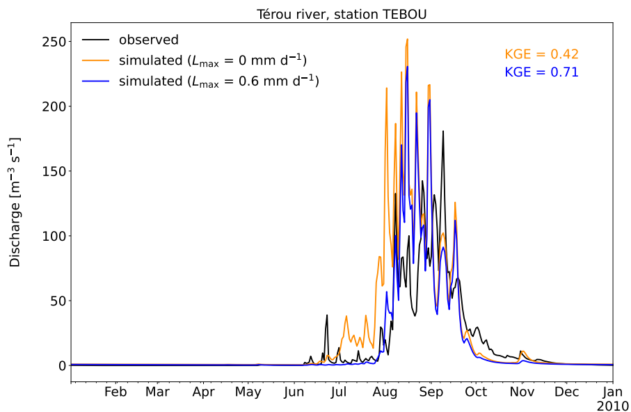
Figure 17. Simulated (with and without groundwater loss) and observed discharge for station TEBOU for 2010.
