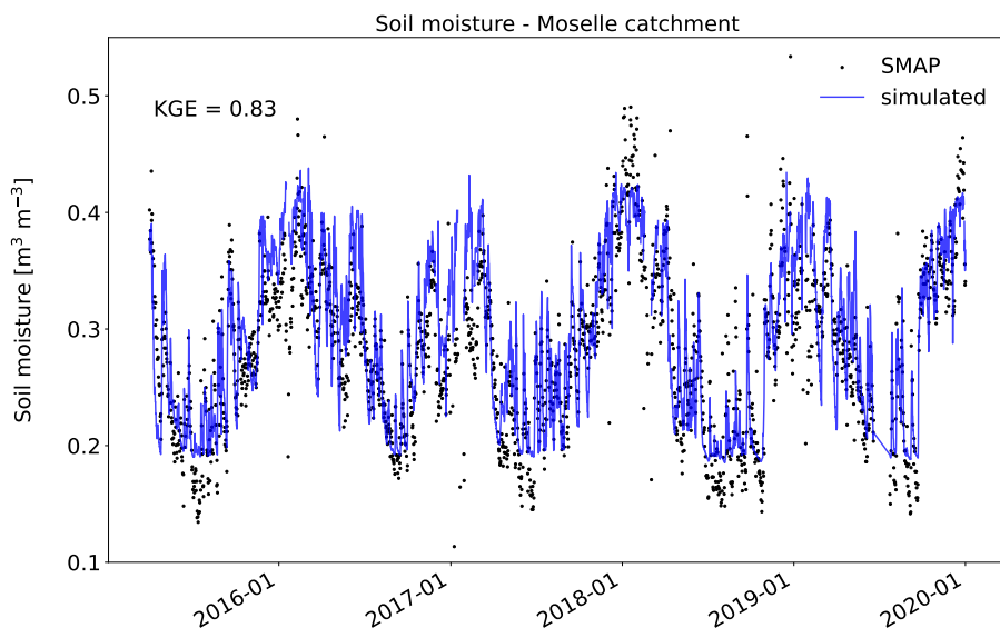
Figure 11. Catchment-average simulated and SMAP soil moisture for the Moselle catchment.
