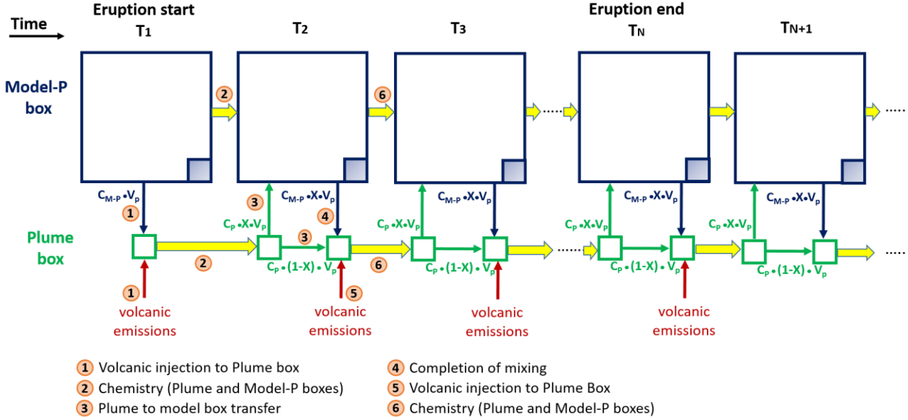
Figure 1: Schematic representation of the plume parameterization. At the timestep corresponding to the start of the eruption the Plume box and the Model-P box are defined: Plume box has a volume ( V_p ) of 0.025^\circ \times 0.025^\circ \times \text{height} and Model-P Box is defined as the Model box ( 0.5^\circ \times 0.5^\circ \times \text{height} ) minus V_p (big blue square minus the shaded blue square) which volume is noted V_{M-P} . The concentrations in the Plume box and Model-P boxes are noted C_p and C_{M-P} , respectively. (Step 1) At T_1 , the Plume box initial chemical concentrations are the background concentrations from the Model-P box plus the volcanic emissions over the timestep (15 min). (Step 2) The chemistry is applied separately to the Plume Box and to the Model-P Box (big arrows in yellow colour). (Step 3) At T_2 , a fraction X of the molecules contained in the Plume box C_p \cdot (X \cdot V_p) are transferred to the Model-P box and (1-X) \cdot V_p kept in the Plume box. (Step 4). To complete the mixing between Plume and Model-P boxes, the Model-P box transfers C_{M-P} \cdot X \cdot V_p to the Plume box. This is at this step that the concentrations in the Model box are output from adding Model-P+Plume concentrations. (Step 5) The concentration of the Plume box is then updated by adding the volcanic emissions calculated from the emission flux (Table 1) over the 15 min model timestep. (Step 6) The chemistry is applied separately to the Plume Box and to the Model-P Box. (big arrows in yellow colour). For the subsequent model timesteps until the end of the eruption, steps 3 to 6 are repeated. After the end of the eruption, Steps 3, 4 and 6 are repeated, i.e. excluding the step of volcanic emissions.
