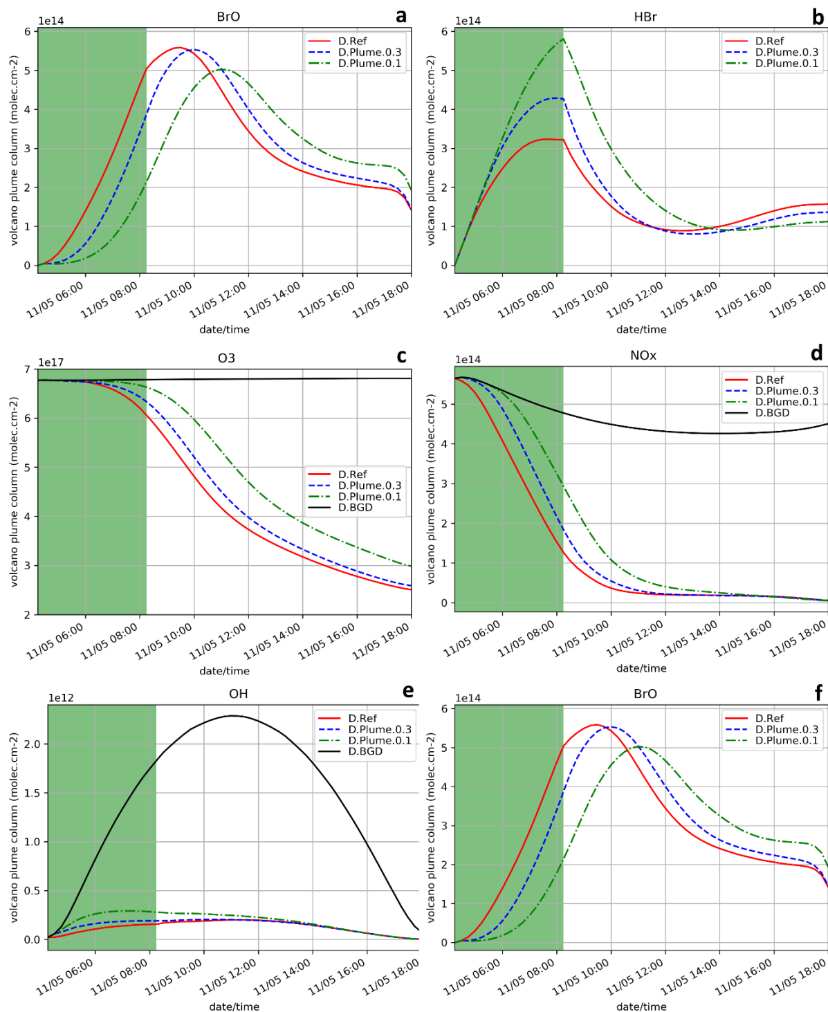
Figure 4: Similar to Fig. 2 but for the daytime simulations D.Ref, D.Plume.0.3 and D.Plume.0.1 from 04:15 UTC. The green zone corresponds to the 4 hours of the volcanic eruption emission (04:15-08:15 UTC).
