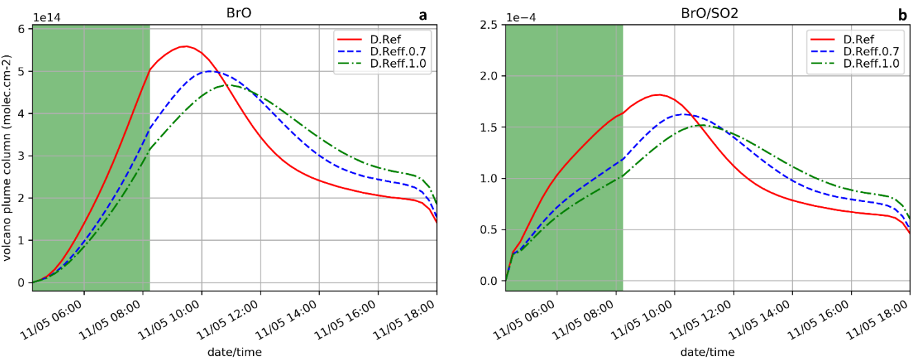
Figure 9: Similar to Fig. 4a and 4f but the simulations testing the sensitivity to the effective radius of sulphate aerosols: D.Ref, D.Reff.0.7 and D.Reff.1.0.
