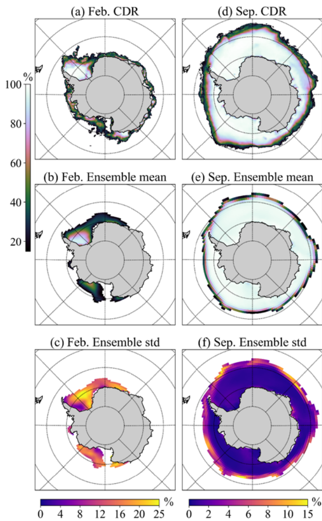
670 Fig. B2. (a-b) Observed (NOAA/NSIDC Climate Data Record of Passive Microwave Sea Ice Concentration, Version 4; CDR) and model ensemble mean February SIC climatologies (only SIC > 15% are shown), (c) standard deviation of all model runs. (d-f) The same as (a-c) but for September.
