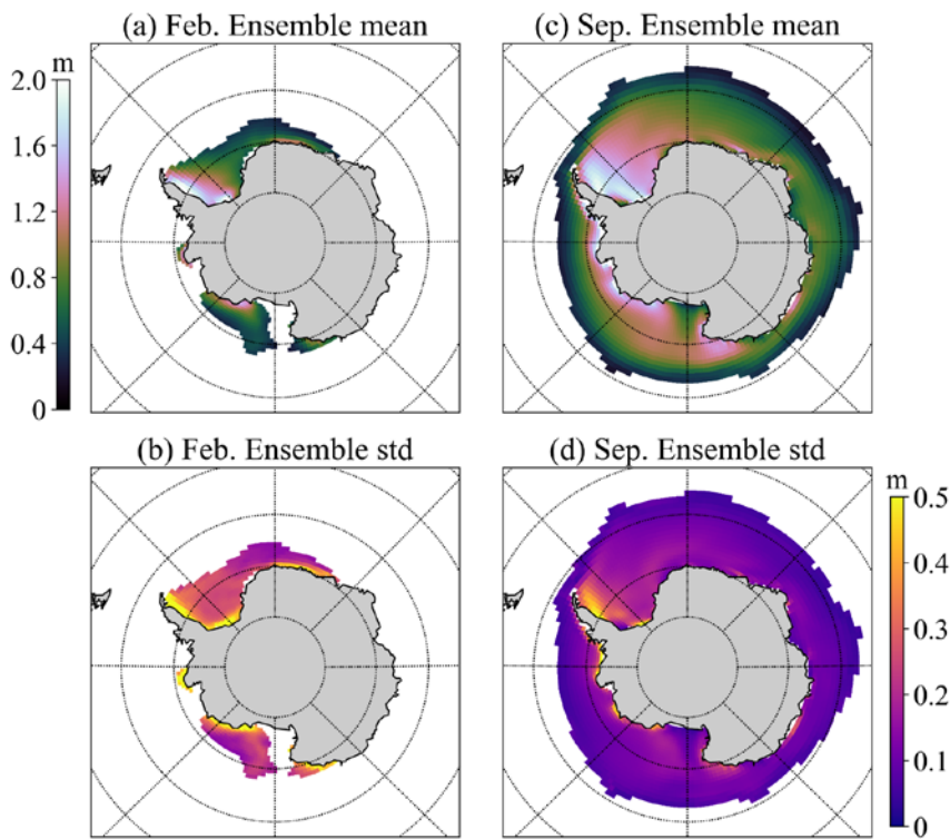
Fig. B3. (a) Ensemble model mean February sea ice thickness climatologies (only SIC > 15% are shown) and (b) the standard deviation. (c-d) The same as (a-b) but for September.
