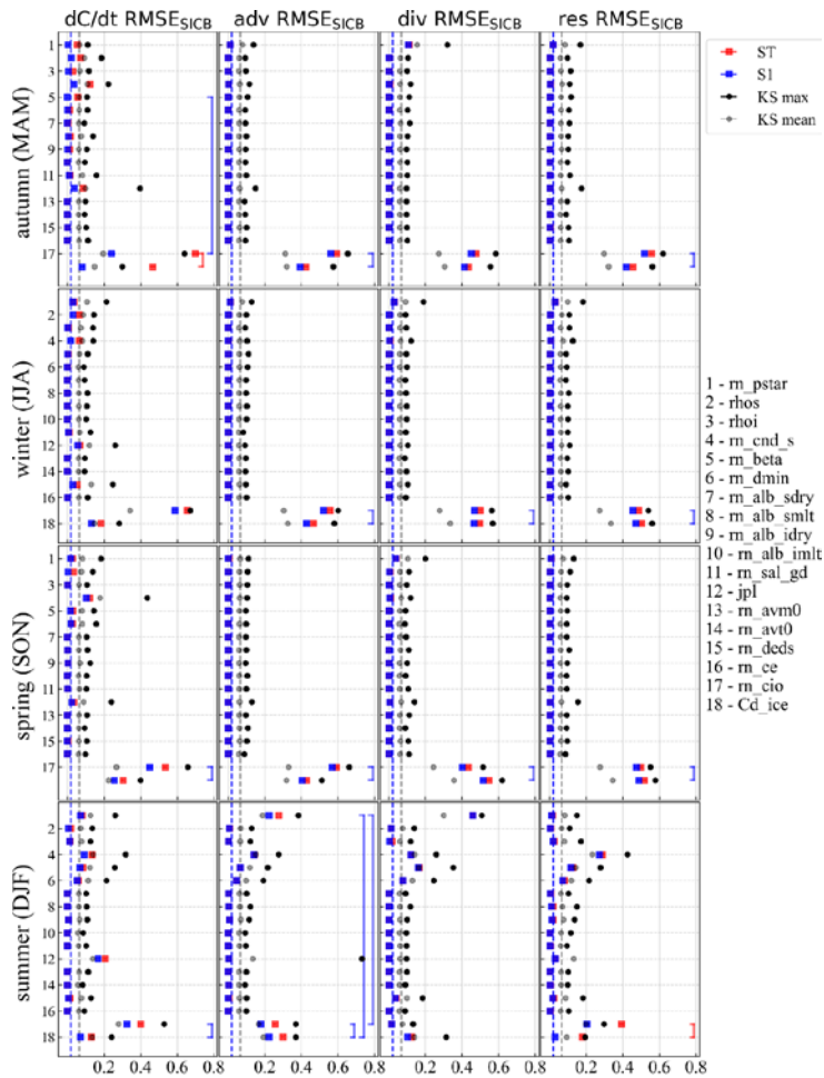
Figure 9. As Fig. 8, but for the sensitivity of the RMSE between SIC budgets of the model and the observational data to 18 parameters. The red connecting lines are the same as the blue ones but for the Sobol second-order index larger than 0.1.
