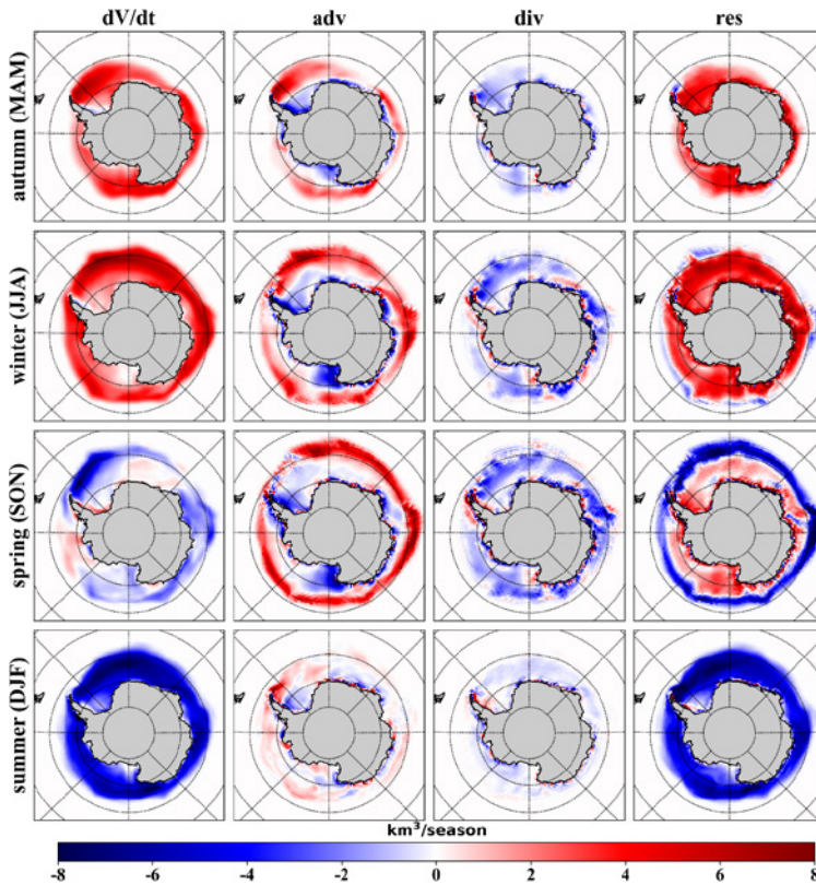
310 Figure 5. As Fig. 3, but for SIV budget. A positive/negative value indicates an increase/decrease in SIV, respectively.
