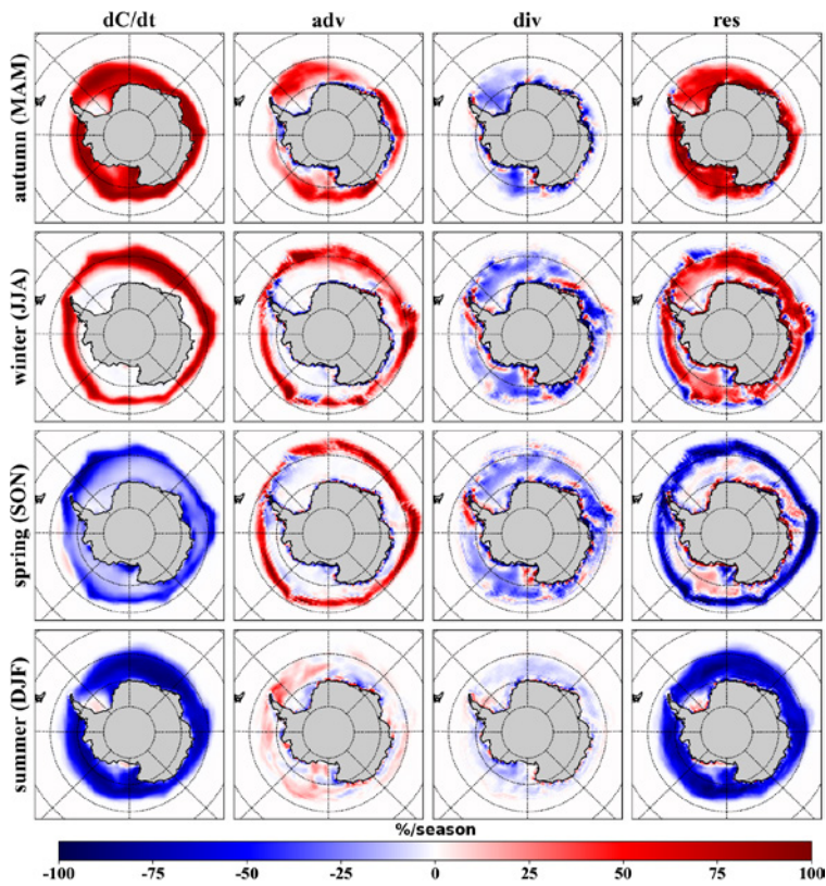
290 Figure 3. Mean seasonal SIC budget components for the ensemble of 449 model runs from 2008 to 2017. The specific meaning of each term has been described in section 2.5. A positive/negative percentage value indicates an increase/decrease in SIC during the season. The first column is the sum of other columns. The SIC budget for each member was first calculated separately and then averaged together.
