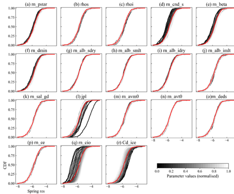
455 Figure 11. Cumulative distribution function (CDF) of the area integral of the res component in the spring SIC budget (cf. Fig. 3). Red lines are the unconditional CDF for the ensemble of 449 model runs, and the grey lines stand for conditional CDF at different fixed values of parameters calculated by the GP emulator. The units of the x-axis are 10^6 \text{ km}^2 .
