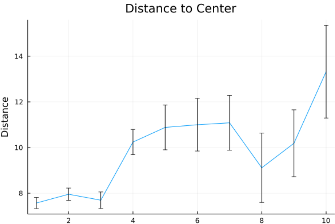
651 Figure 24: Measurement distance to center, POMCPOW without action constraints, single body with variable location. The plot 652 shows the average distance between the measurement location and the mineralization center for the measurements at each time step. 653 One standard error bars are also presented.
