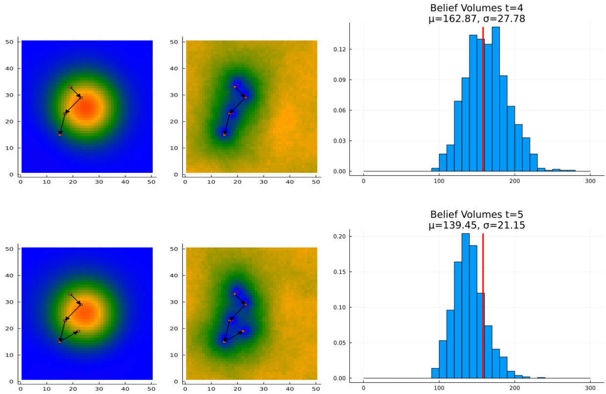
Figure 9: Initial measurement trajectory. Each figure shows the belief resulting from the measurements taken by the agent. The circles show the locations at which measurements were taken. The arrows indicate the sequence in which actions were taken.
