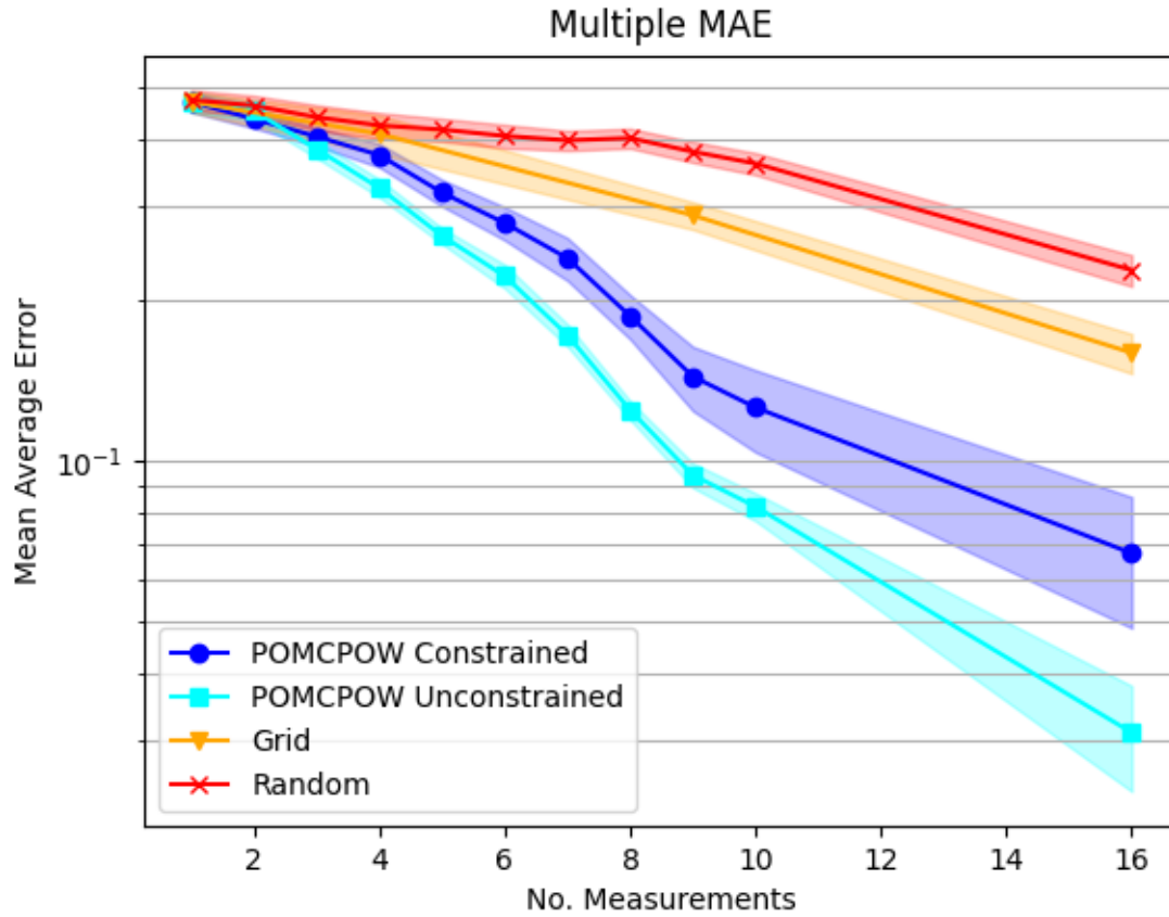
Figure 25: Relative MAE, two mineralization processes. The plot shows the mean relative absolute error after a given number of measurements taken under each tested method. The mean absolute error is shown along with one standard error bounds for each trend.
