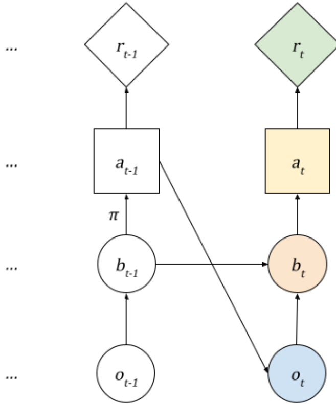
Figure 4: Exploration Markov Decision Process. Each decision step, the agent selects an action a_t based on its current belief over the world state using a planner ( \pi ). The agent takes the action in the world and observes some new data o_{t+1} . This data is used to update the belief b_{t+1} for the next step. Each action results in a reward.
