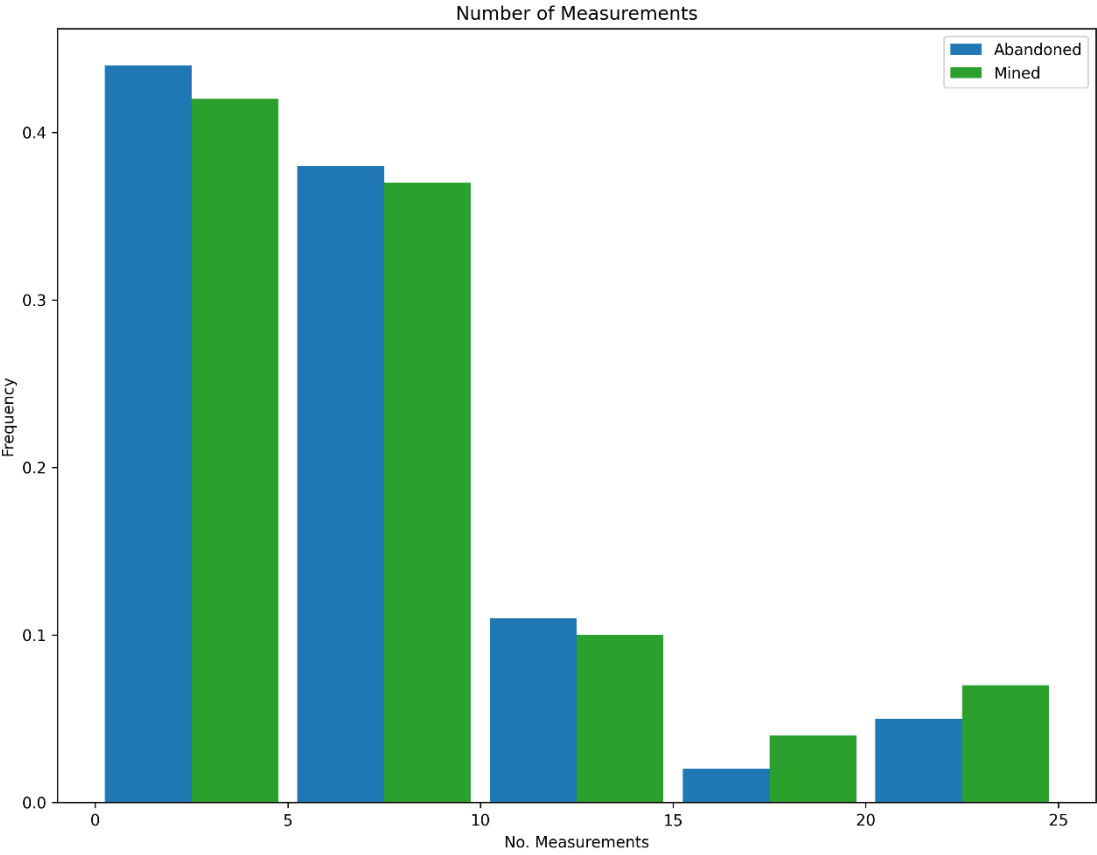
685 686 Figure 27: Measurement histogram, POMCPOW with action constraints, multiple ore-bodies. This figure shows histogram of the 687 number of measurements taken by the POMCPOW solver over all Monte Carlo trials. The trials were limited to a maximum of 25 688 measurements.
