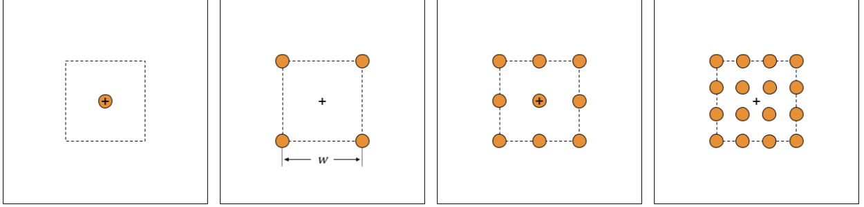
Figure 12: Baseline grid patterns. The figures show the baseline grid patterns for 2-by-2, 3-by-3 and 4-by-4 grids, each with a total of 4, 9, and 16 measurements respectively. The grids cover the extent of a w -by- w area in the center of the exploration domain. A single measurement at the center of the domain is also shown in the leftmost figure.
