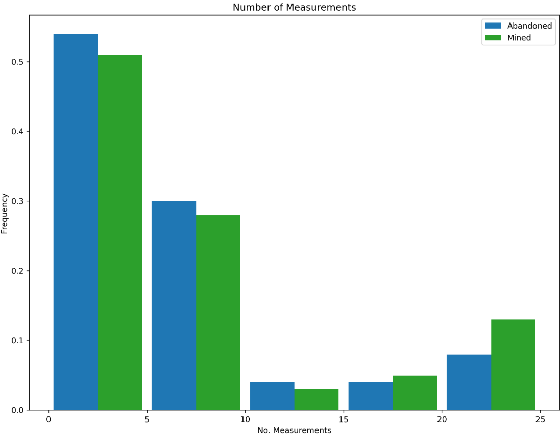
623 Figure 21: Measurement histogram, POMCPOW with action constraints, single body with variable location. This figure shows 624 histogram of the number of measurements taken by the POMCPOW solver over all Monte Carlo trials. The trials were limited to a 625 maximum of 25 measurements.
