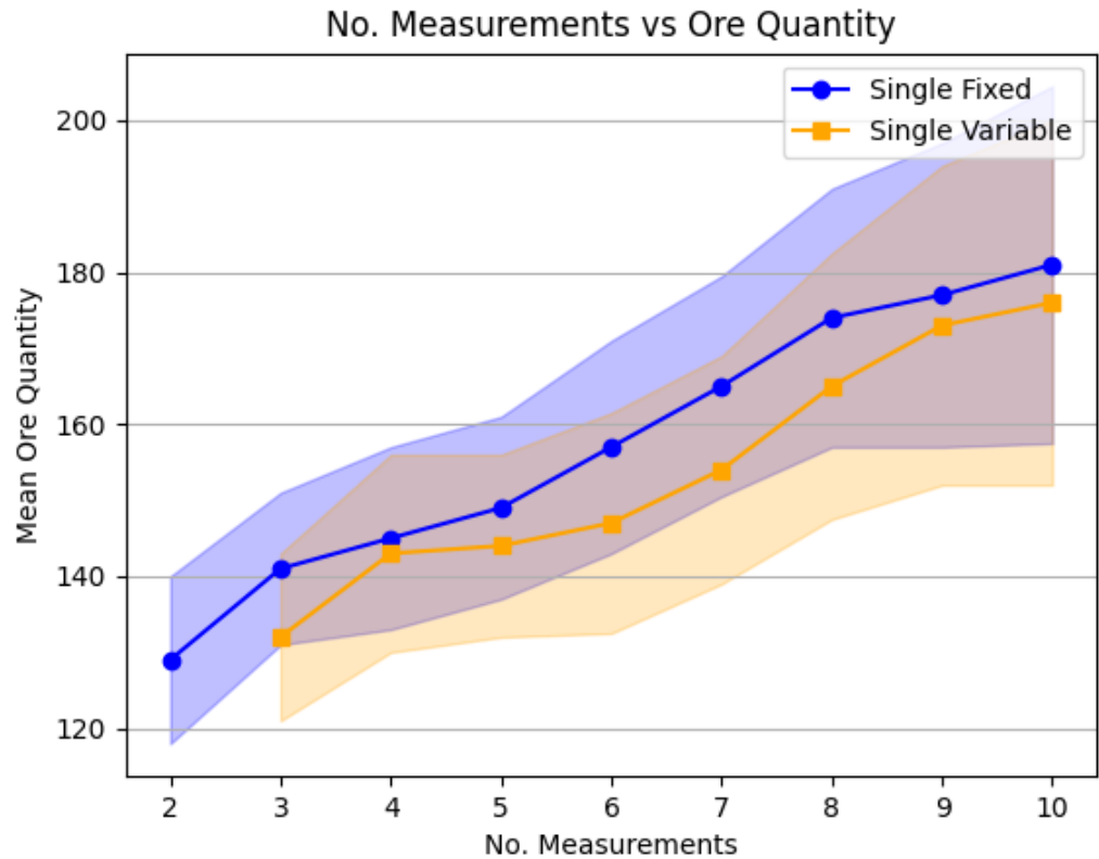
Figure 32: Measurement campaign length and deposit size. The mean deposit size is shown for different measurement campaign lengths, along with one standard-error bounds.
