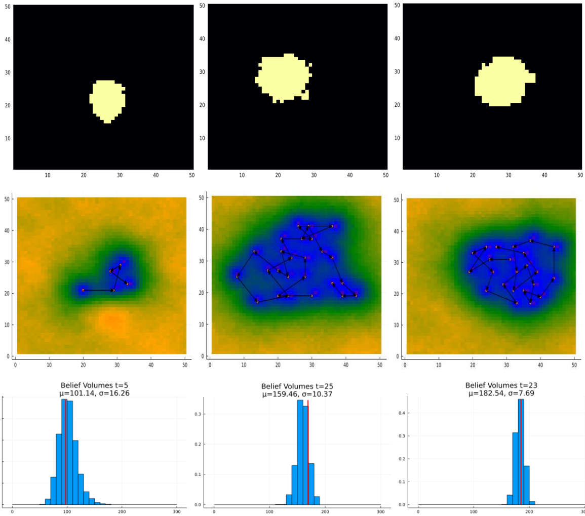
Figure 30: Deposit size study results for the single body with variable centroid location case. The sub-economic, borderline, and economic cases are shown in the left, center, and right columns, respectively. The top row shows the massive ore present in the tested case. The center row shows the trajectory taken by POMCPOW and the standard deviation of the resultant belief. The bottom row shows the histogram of the ore volumes in the final belief along with the true massive ore volume.
