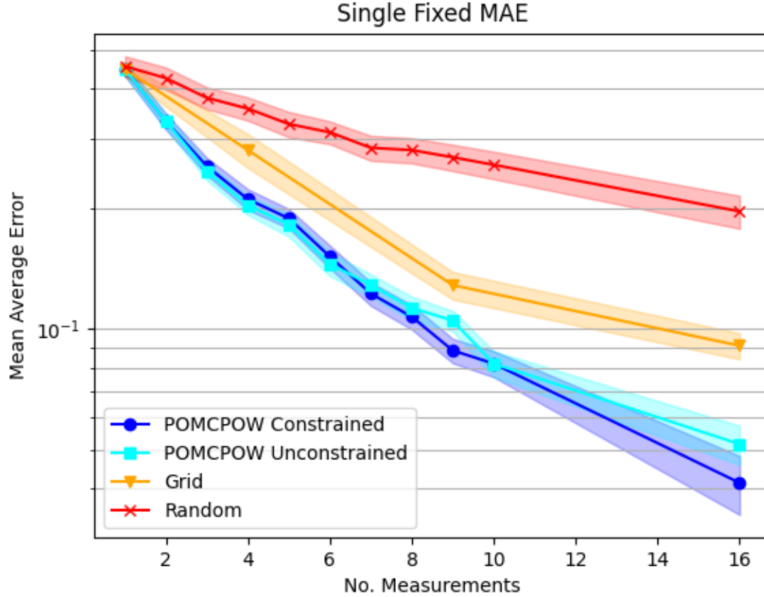
Figure 13: Relative MAE single mineralization, fixed location. The plot shows the mean relative absolute error after a given number of measurements taken under each tested method. The mean absolute error is shown along with one standard error bounds for each trend.
