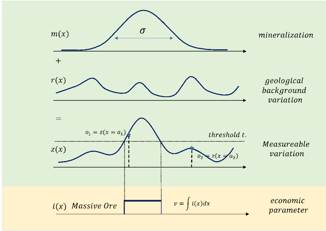
Figure 1. Example 1D Mineralization. Sub-figure (A) shows a mineralization that is altered by geological background variation (B), resulting in the measurable variation (C). The massive orebody (D), whose volume is the economic parameter of interest, exists at locations where z(x) exceeds a threshold value.
