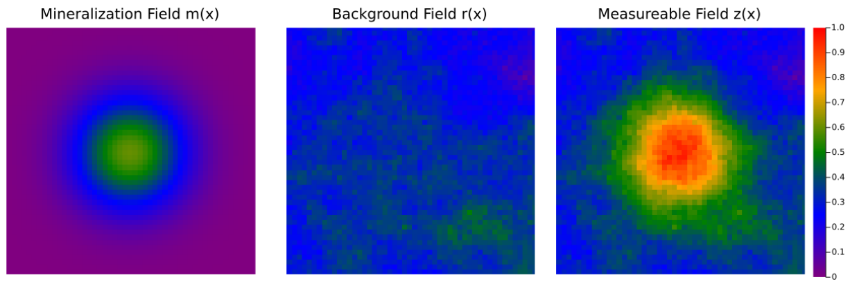
Figure 2. Two-dimensional exploration problem. The mineralization field m(x) (left), the background field r(x) (center) are summed to create the measurable field z(x) (right).
