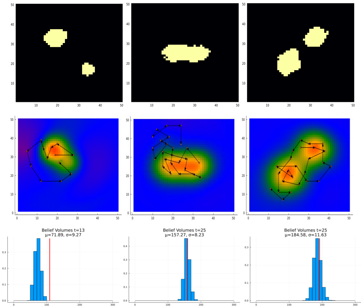
Figure 31: Deposit size study results for multi-body case. The sub-economic, borderline, and economic cases are shown in the left, center, and right columns, respectively. The top row shows the massive ore present in the tested case. The center row shows the trajectory taken by POMCPOW and the standard deviation of the resultant belief. The bottom row shows the histogram of the ore volumes in the final belief along with the true massive ore volume.
