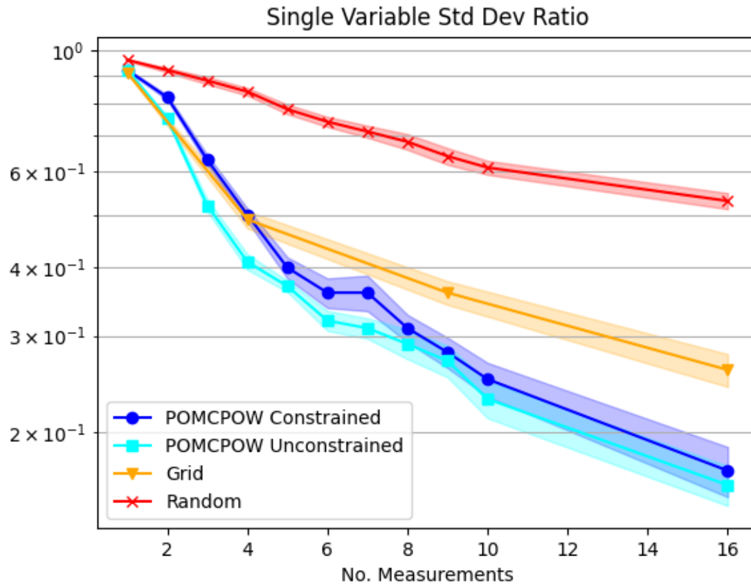
Figure 20: Single Body, variable location standard deviation ratios. The plot shows the mean standard deviation ratio after a given number of measurements taken under each tested method. The mean ratio is shown along with one standard error bounds for each trend.
