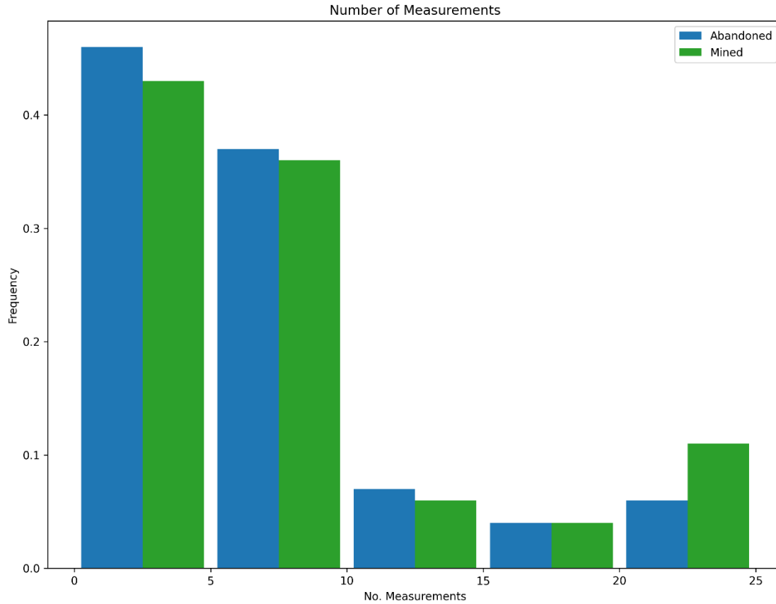
Figure 28: Measurement histogram, POMCPOW without action constraints, multiple ore-bodies. This figure shows histogram of the number of measurements taken by the POMCPOW solver over all Monte Carlo trials. The trials were limited to a maximum of 25 measurements.
