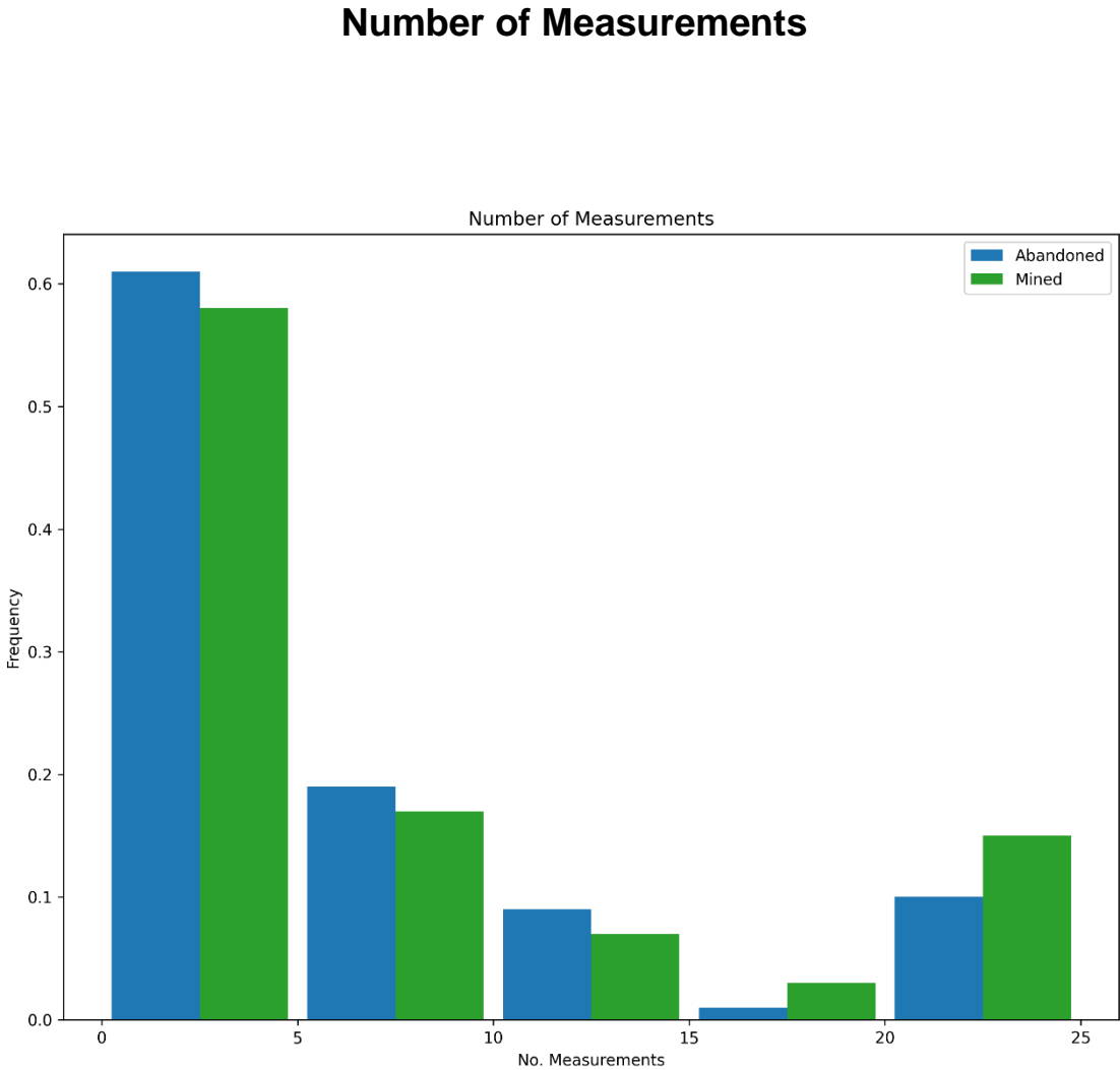
Figure 15: Measurement histogram, POMCPOW with action constraints, single body with fixed location. This figure shows histogram of the number of measurements taken by the POMCPOW solver over all Monte Carlo trials. The trials were limited to a maximum of 25 measurements.
