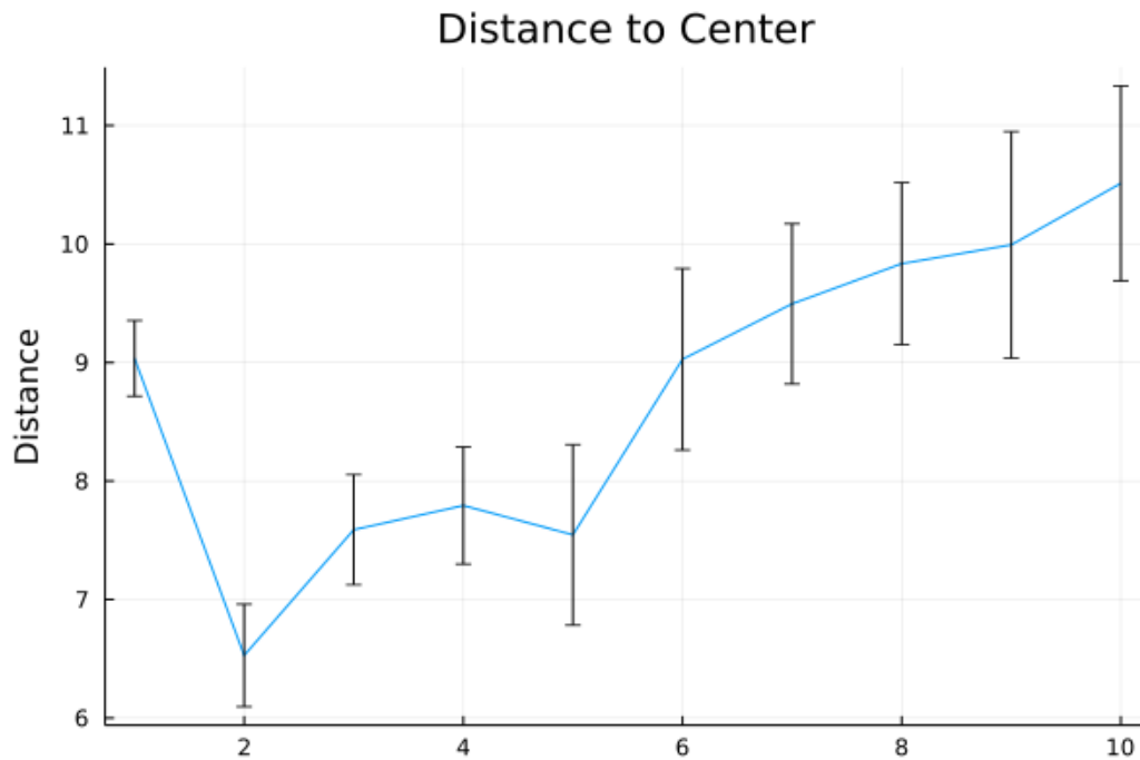
Figure 16: Measurement distance to center, POMCPOW with action constraints, single body with fixed location. The plot shows the average distance between the measurement location and the mineralization center for the measurements at each time step. One standard error bars are also presented.
