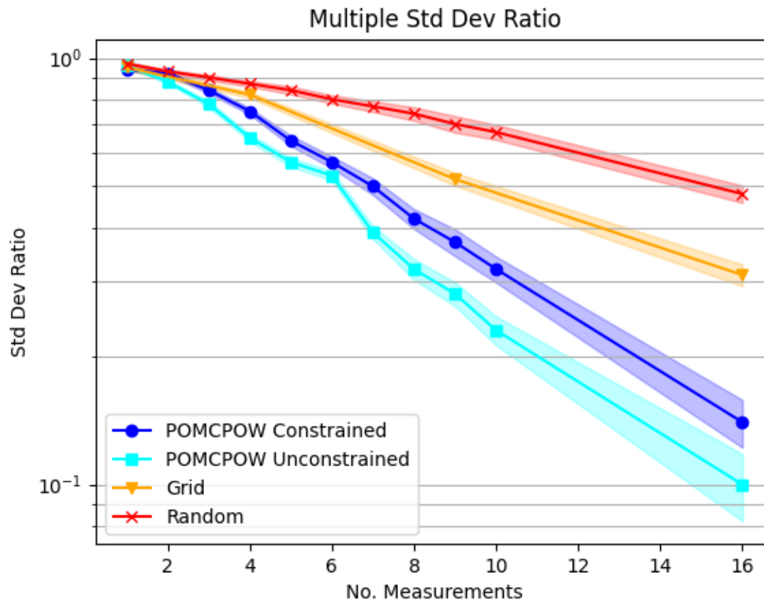
Figure 26: Two mineralization process standard deviation ratios. The plot shows the mean standard deviation ratio after a given number of measurements taken under each tested method. The mean ratio is shown along with one standard error bounds for each trend.
