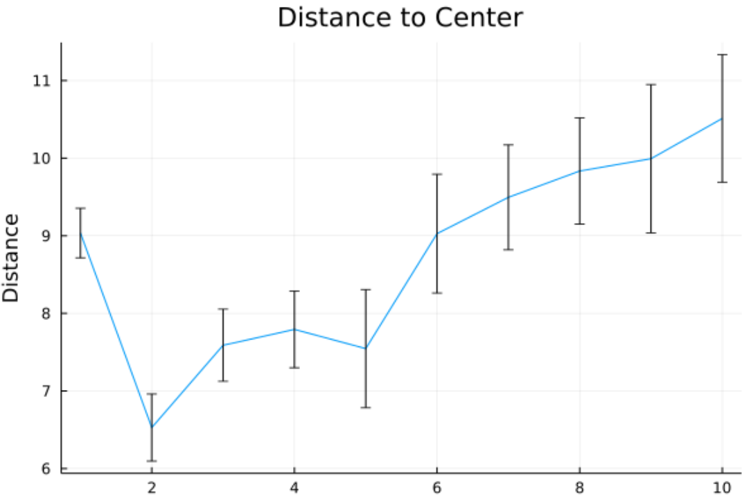
585 Figure 18: Measurement distance to center, POMCPOW without action constraints, single body with fixed location. The plot shows 586 the average distance between the measurement location and the mineralization center for the measurements at each time step. One 587 standard error bars are also presented.
