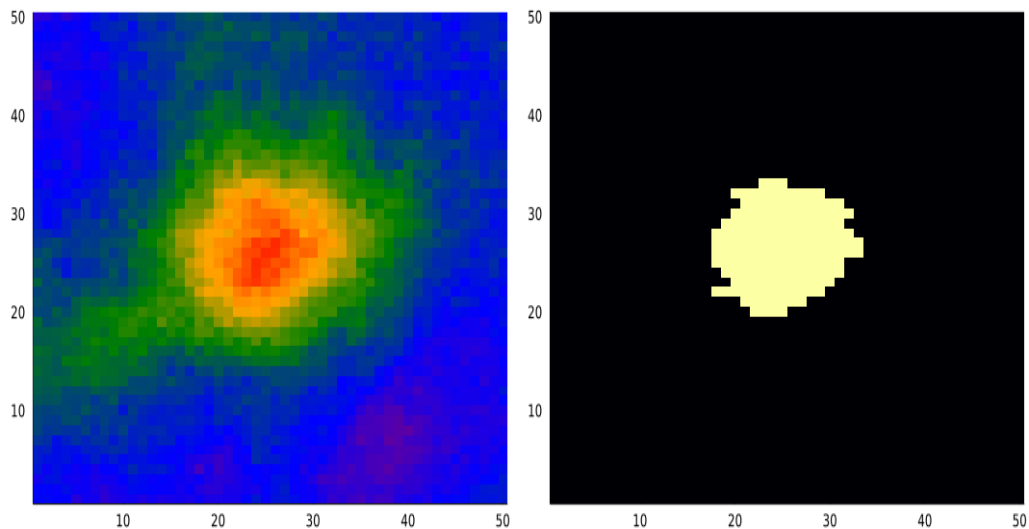
Figure 6: Illustration case. The left figure shows the mineralization z(x) of the example case. The right figure shows the massive ore mass of the mineral field i(x) .
