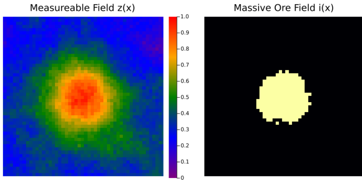
Figure 3. Two-dimensional economic field. The massive ore field i(x) shows where the measurable field z(x) exceeds the economic threshold z_{threshold} .
