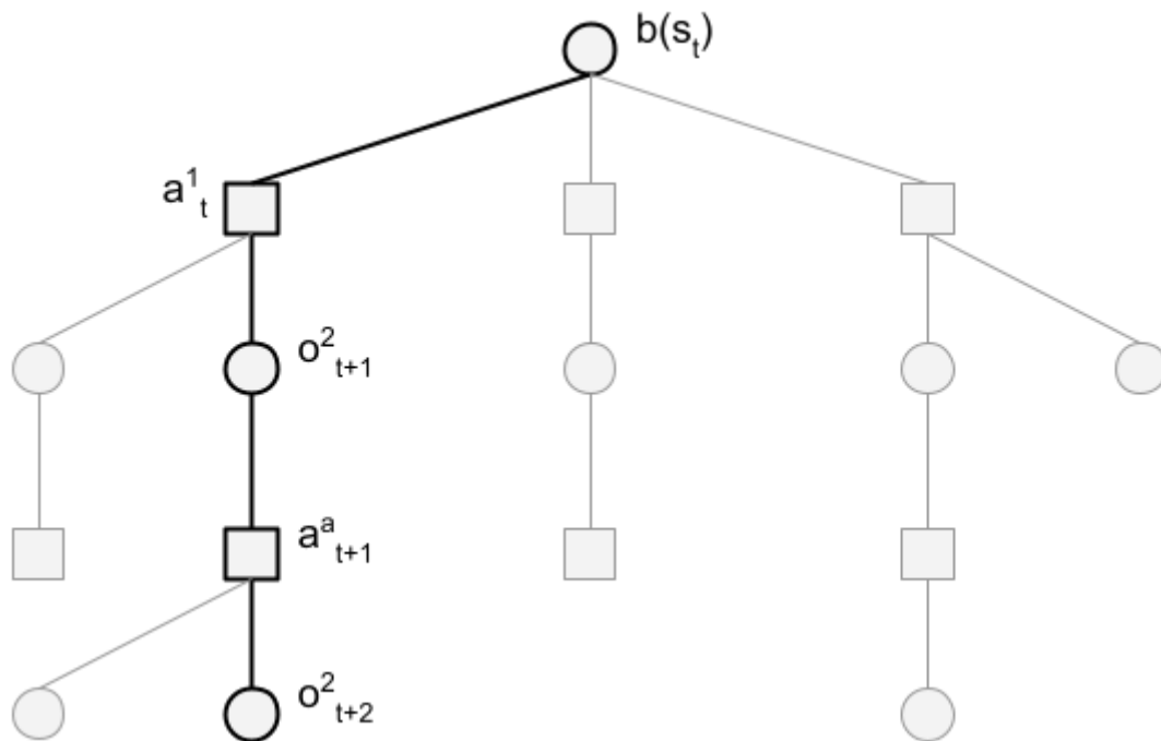
Figure 5: Monte Carlo search tree. Each simulation in an MCTS algorithm is encoded into a search tree. The example tree is rooted at the belief, b(s_t) given at the start of search. Paths from the root to a leaf of the tree represent a simulated trajectory of alternating actions, a_t^i and observations, o_t^i . An example trajectory in the tree is shown in bold.
