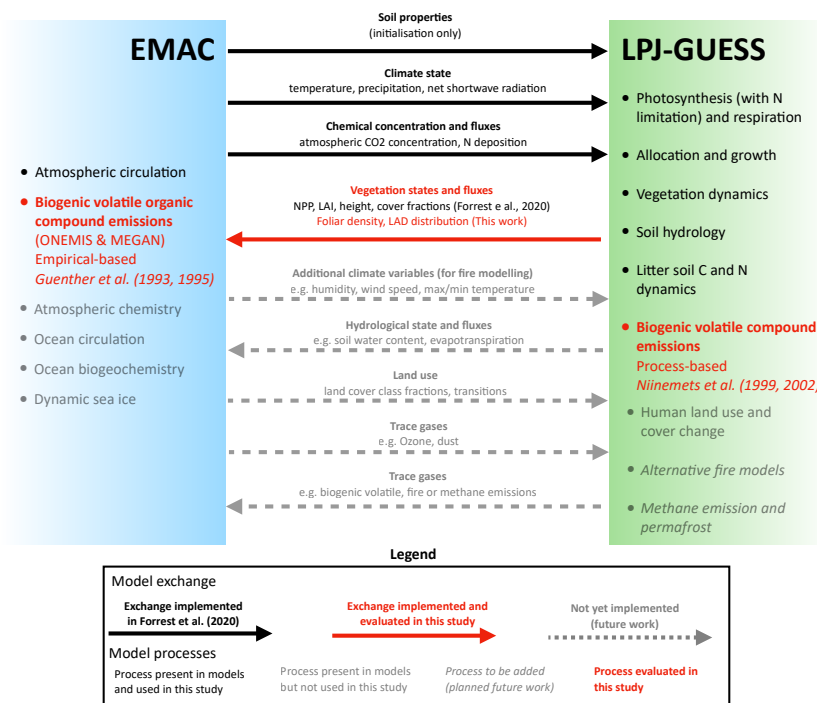
Figure 1. The main processes and exchanges in the coupled model framework adopted from Forrest et al. (2020). The work in this study is highlighting in red.
