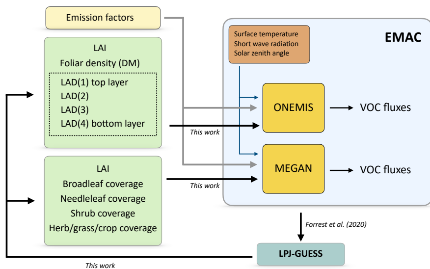
Figure 2. Model setup for BVOC emission estimates in EMAC. The vegetation variables needed in ONEMIS and MEGAN are now provided by LPJ-GUESS, replacing offline climatological datasets.
