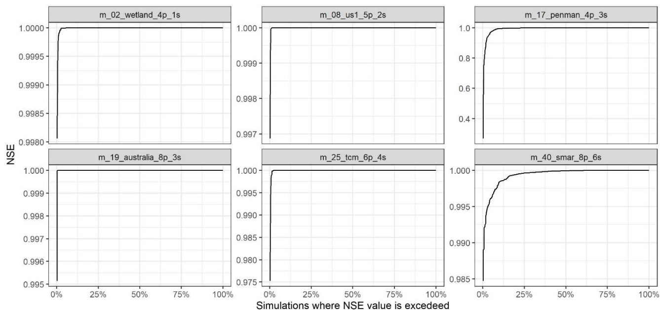
Figure 4: NSE values calculated between streamflow simulated with MARRMoT v2.0 and v2.1. All models not shown had NSE > 0.999 for all simulations.
