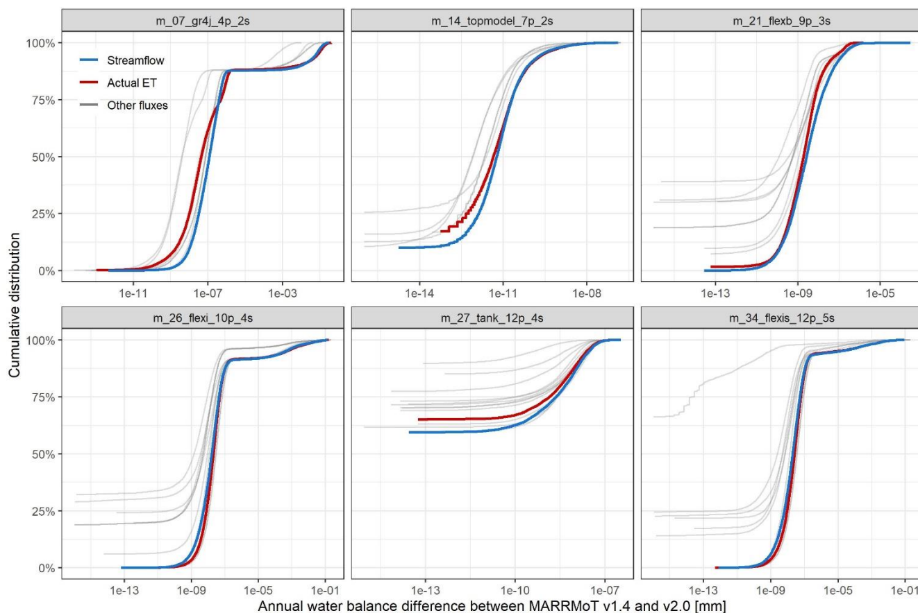
Figure 2: Differences in the annual water balance of simulations from MARRMoT v1.4 and v2.0. All models not shown have differences smaller than 1 \times 10^{-16} \text{ mm} . Cumulative distributions are calculated across all years and catchments aggregated.
