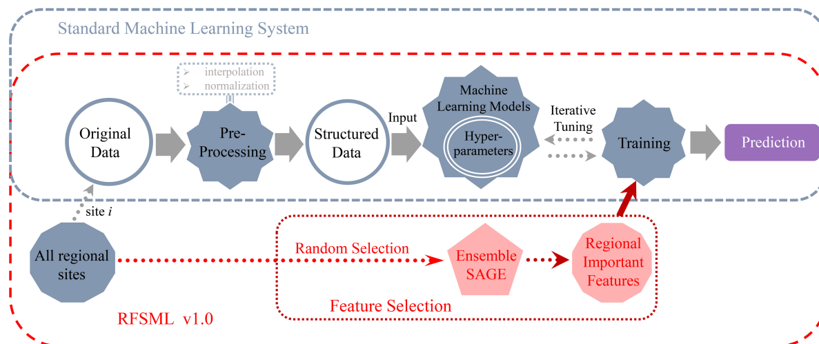
Figure 3. RFSML versus standard machine learning system framework.
