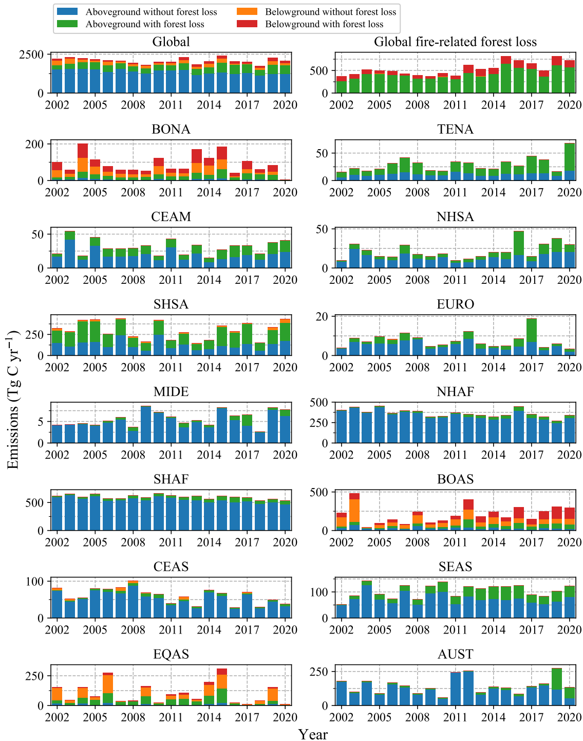
Figure 7: Annual 2002–2020 emissions for the global total, global fire-related forest loss, and the 14 GFED regions. Bars are subdivided in aboveground and belowground emissions, and in fire without forest loss and with forest loss (i.e. fire-related forest loss).
