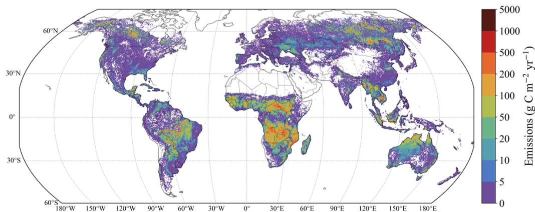
Figure 5: Global annual (a) burned area, (b) fuel consumption, and (c) emissions, averaged over 2002–2020. Burned area displayed in panel a is the total burned area derived from combining the MODIS MCD64A1 product and additional fire-related forest loss burned area from active fire detections that overlap forest loss. Maps are aggregated to 0.25° for display.
