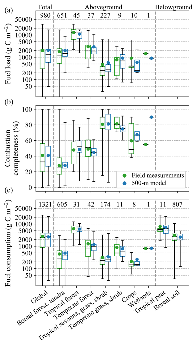
1075 Figure 3: Comparison of field measurements of (a) fuel load, (b) combustion completeness and (c) consumption versus model estimates for all field data (Table 2), grouped per biome class. The number of measurement records included is given above each boxplot. Aboveground and belowground fuel classes are grouped separately. Belowground fuel classes (Tropical peat, boreal soil) are only reported for fuel consumption measurements because our model relied on static SOC density maps for calculating soil fire emissions (See Methods). Global values are for the total measured fuel available, which in case of (a) and (b) are aboveground values, and for (c) is the sum of above- and belowground for each measurement record. Note that the number of fuel consumption 1080 measurements for the individual biomes does not sum to the global total number of sites (1321) because measurement records with both aboveground and belowground values are being counted as one record in the Global class. The y-axis of panel (a) and (c) are logarithmic and the y-axis of panel (b) is linear. Boxplot whiskers give the range of data.
