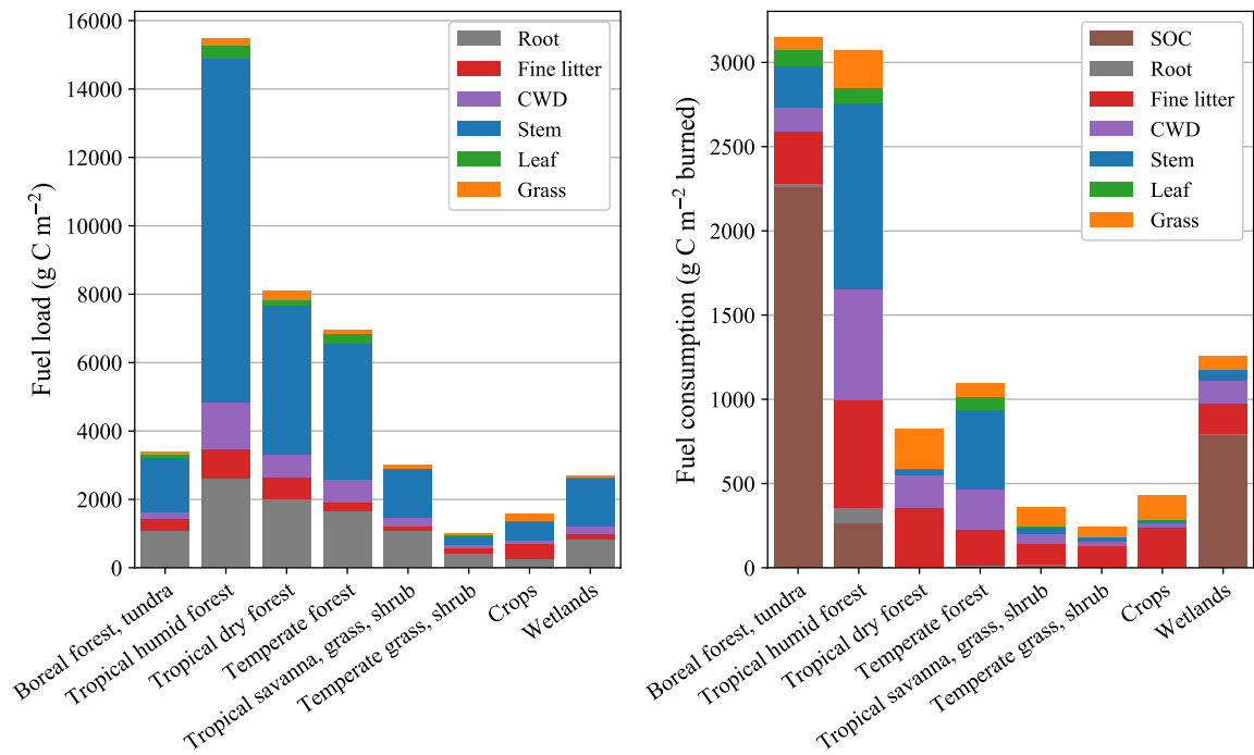
Figure 4: 2002–2020 average (a) fuel load and (b) fuel consumption per biome. Bars are subdivided in model biomass and litter pools. Because of the use of static SOC maps, panel a does not include soil organic carbon fuel loads.
