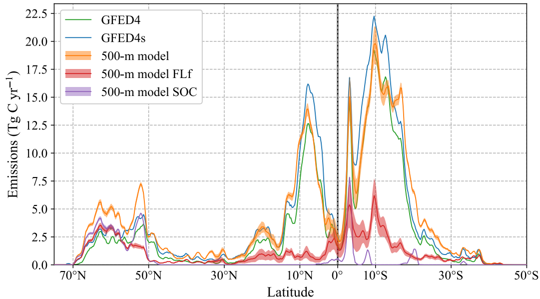
Figure 8: Annual global emissions for the 500-m model for 2002–2020 versus GFED4s for the same time period and GFED4 for 2002–2016 as (a) time series and (b) latitudinal total emissions. Contributions to 500-m model emissions from fire-related forest loss (FLf) and SOC burning are displayed separately. Note that these sub-categories partly overlap: fire-related forest loss emissions include part of SOC burning emissions and vice versa. Transparent bands around estimates show the range between minimum- and maximum-probability fire-related forest loss. All lines are based on 0.25° aggregated data and smoothed using a moving-average filter with a window size of 4 grid cells, i.e. 1° latitude.
