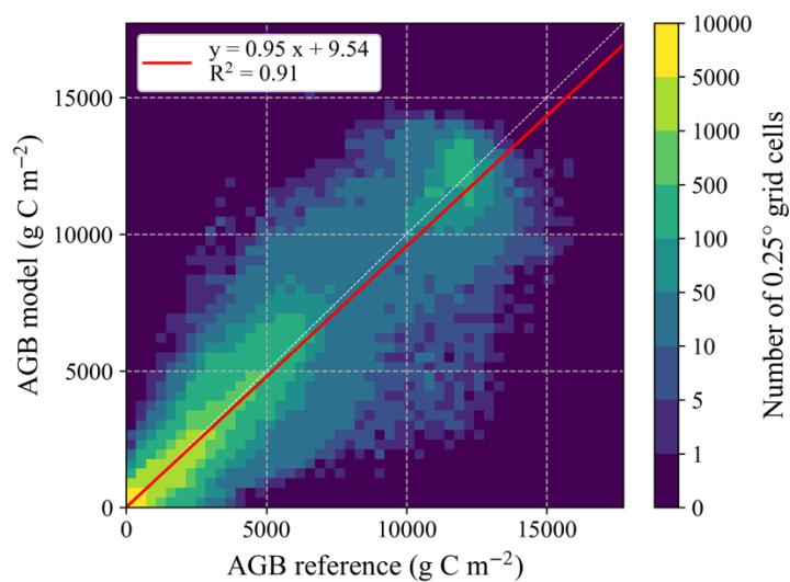
1070 Figure 2: (a) Modelled aboveground biomass (AGB) averaged over 2002–2020, (b) comparison of modelled versus reference aboveground biomass at an aggregated 0.25° grid cell level. Model AGB comprises the stem, leaf and grass model pools and does not include litter pools. Panel (a) is aggregated to 0.25° for display.
