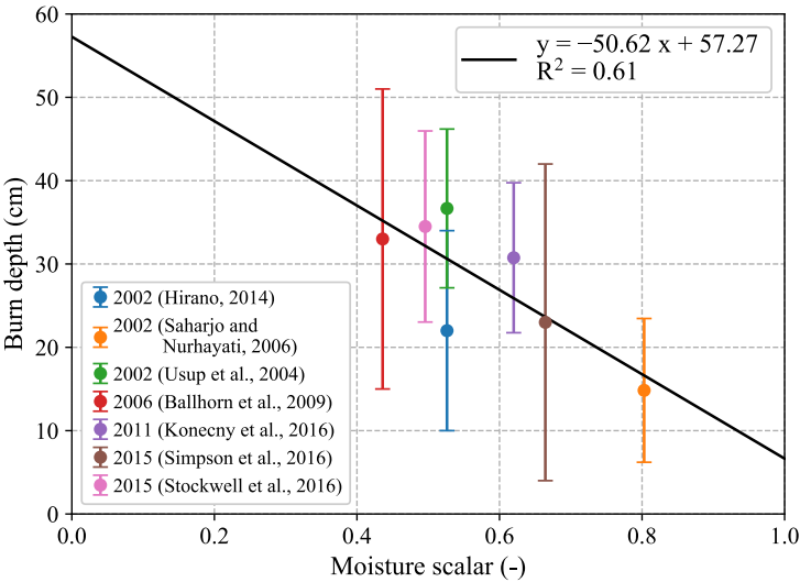
Figure 1: Parameterization of burn depth in tropical peat lands ( D_{burn\_tropicals} ) as a function of the soil moisture scalar. The tropical peat burn depth was based on a linear regression function derived from the relationship between field measurements of burn depth and the soil moisture scalar. The soil moisture scalar was based on the depth-weighted average volumetric soil water content over the ERA5-land model depths of 0–7 cm, 7–28 cm, and 28–100 cm (Muñoz Sabater, 2019).
