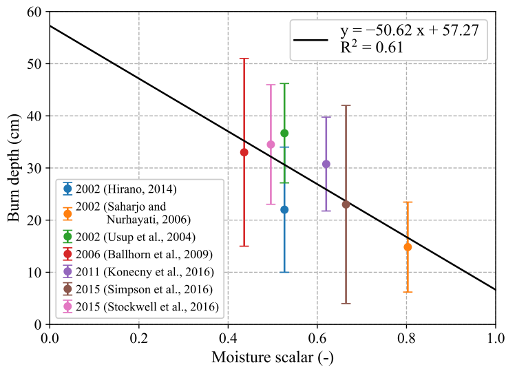
1065 Figure 1: Parameterization of burn depth in tropical peat lands ( D_{burn\_tropics} ) as a function of the soil moisture scalar. The tropical peat burn depth was based on a linear regression function derived from the relationship between field measurements of burn depth and the soil moisture scalar. The soil moisture scalar was based on the depth-weighted average volumetric soil water content over the ERA5-land model depths of 0–7 cm, 7–28 cm, and 28–100 cm (Muñoz Sabater, 2019).
