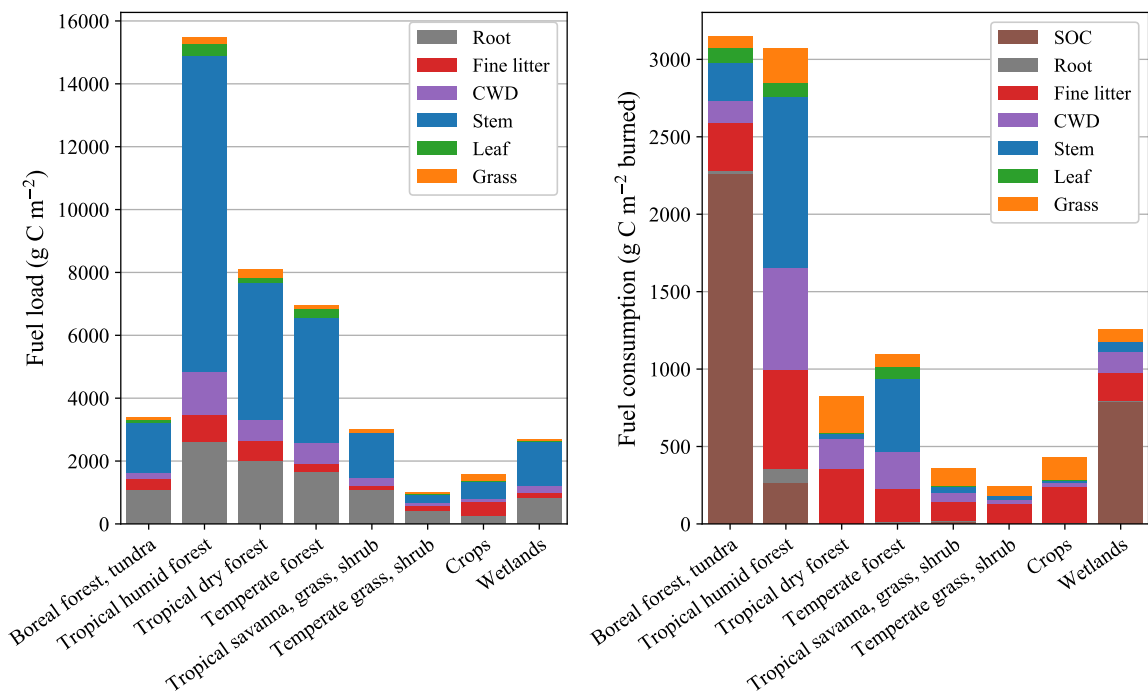
|095 Figure 4: 2002– 2019 –2020 average (a) fuel load and (b) fuel consumption per biome. Bars are subdivided in model biomass and litter pools. Because of the use of static SOC maps, panel a does not include soil organic carbon fuel loads.
