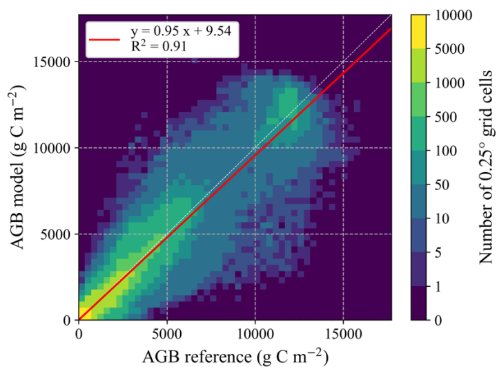
Figure 2: (a) Modelled aboveground biomass (AGB) averaged over 2002– 2019 2020, (b) comparison of modelled versus reference aboveground biomass at an aggregated 0.25° grid cell level. Model AGB comprises the stem, leaf and grass model pools and does not include litter pools. Panel (a) is aggregated to 0.25° for display.
