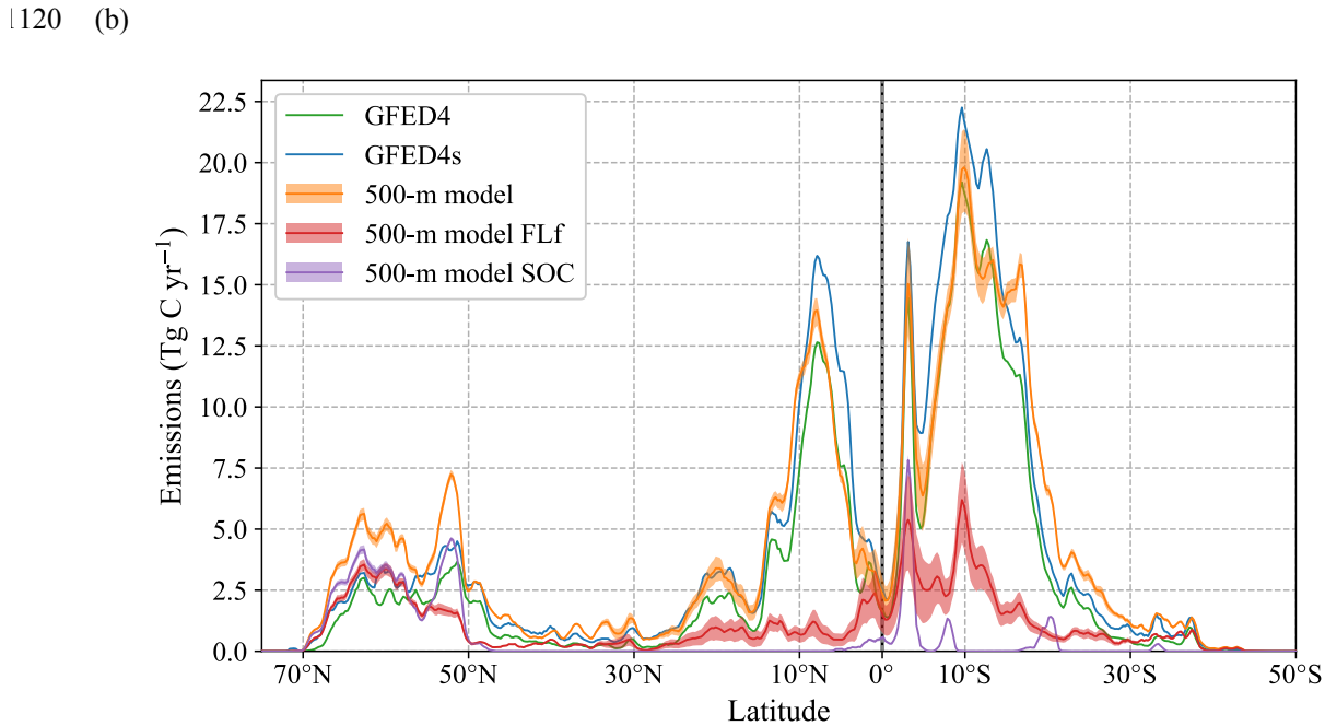
Figure 8: Annual global emissions for the 500-m model for 2002–2019–2020 versus GFED4s for the same time period and GFED4 for 2002–2016 as (a) time series and (b) latitudinal total emissions. Contributions to 500-m model emissions from fire-related forest loss (FLf) and SOC burning are displayed separately. Note that these sub-categories partly overlap: fire-related forest loss emissions include part of SOC burning emissions and vice versa. Transparent bands around estimates show the range between minimum- and maximum-probability fire-related forest loss. All lines are based on 0.25° aggregated data and smoothed using a moving-average filter with a window size of 4 grid cells, i.e. 1° latitude.
