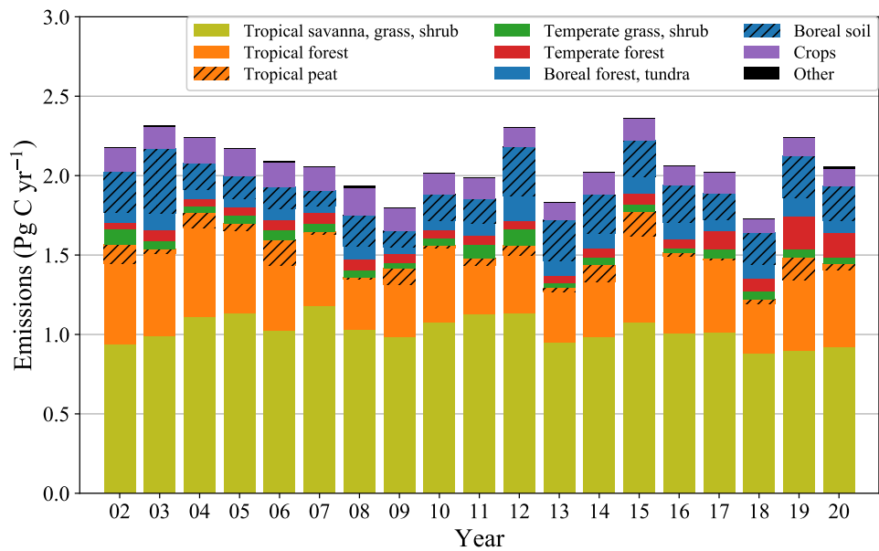
Figure 6: Global annual emissions for 2002– 2019 –2020 based on the 500-m model. Bars are subdivided into biomes, with belowground emissions in two separate classes (Tropical peat, boreal soil).
