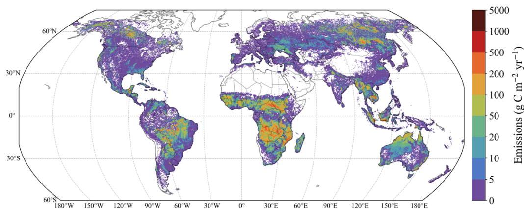
105 Figure 5: Global annual (a) burned area, (b) fuel consumption, and (c) emissions, averaged over 2002–20192020. Burned area displayed in panel a is the total burned area derived from combining the MODIS MCD64A1 product and additional fire-related forest loss burned area from active fire detections that overlap forest loss. Maps are aggregated to 0.25° for display.
