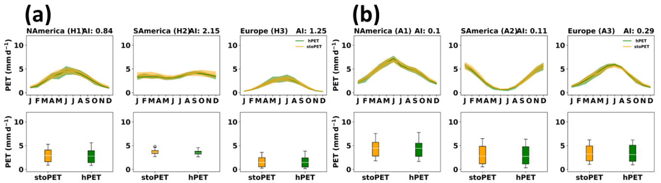
Figure 8: The seasonal PET and box plots for North America, South America, and Europe for the (a) humid and (b) arid locations as located in Fig. 7. The box plots show the distribution of each dataset over the 20 years period. The box indicates the IQR (25 th -75 th ) while the upper whiskers are set to (75 th + 1.5 * IQR) and the lower whiskers are set to (25 th - 1.5 * IQR).
