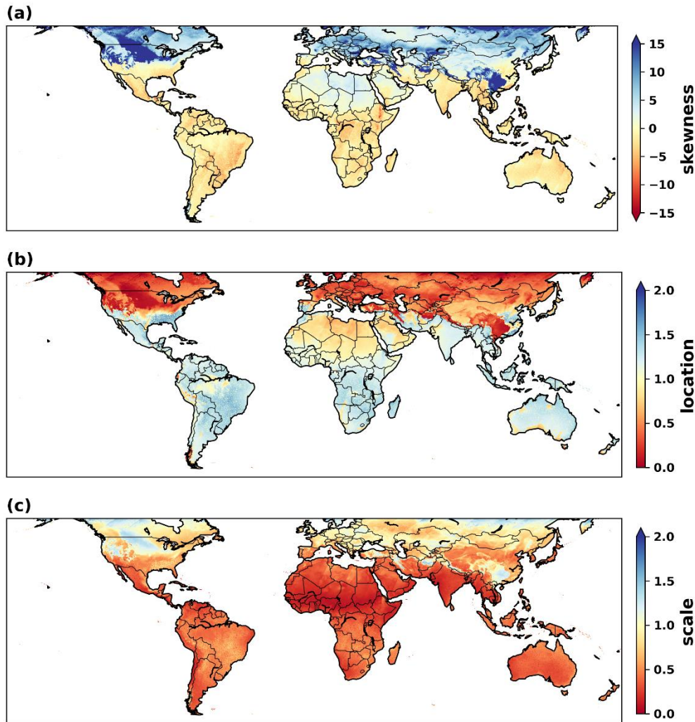
10 Figure 3: The parameters representing the noise ratio (a) skewness, (b) location, and (c) scale for January over the spatial domain of the stoPET model.
