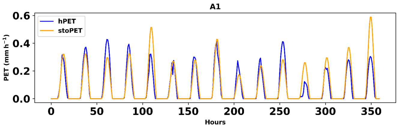
Figure 12: Time series of hPET and stoPET data for the last 15 days of 2020 (for A1 in Fig. 7). The figure indicates that stoPET capture the diurnal cycle of PET and the difference among each day shows the stochasticity of the model.
