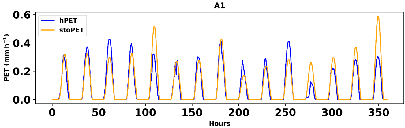
Figure 12: Time series of hPET and stoPET data for the last 15 days of 2020 (for A1 in Fig. 7). The figure indicates that stoPET capture the diurnal cycle of PET and the difference among each day is an expression of the stochasticity of the model.
