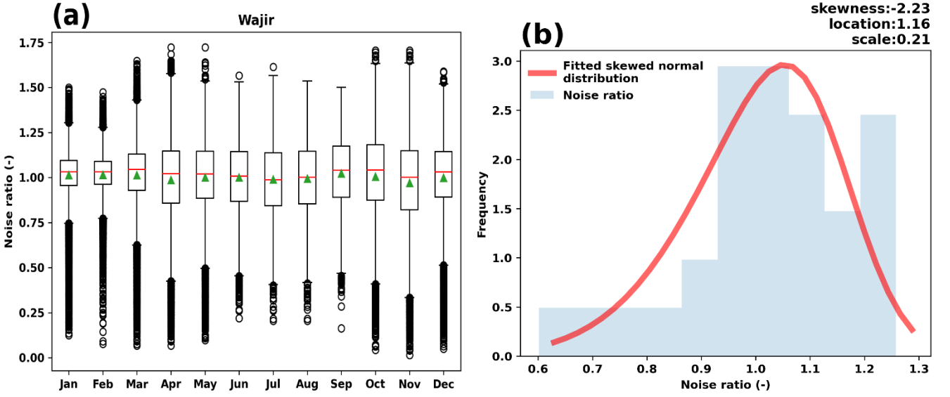
Figure 4: (a) Noise ratio box plot for a single location in Wajir (Kenya). The box plots indicate that the noise ratio is variable over each month with the green triangle showing the mean and the red line in the box plot indicating the median (b) A histogram for the January noise ratio is shown in blue, with the fitted skewed normal distribution shown in red. The corresponding distribution parameters are indicated in the top left of the plot.
