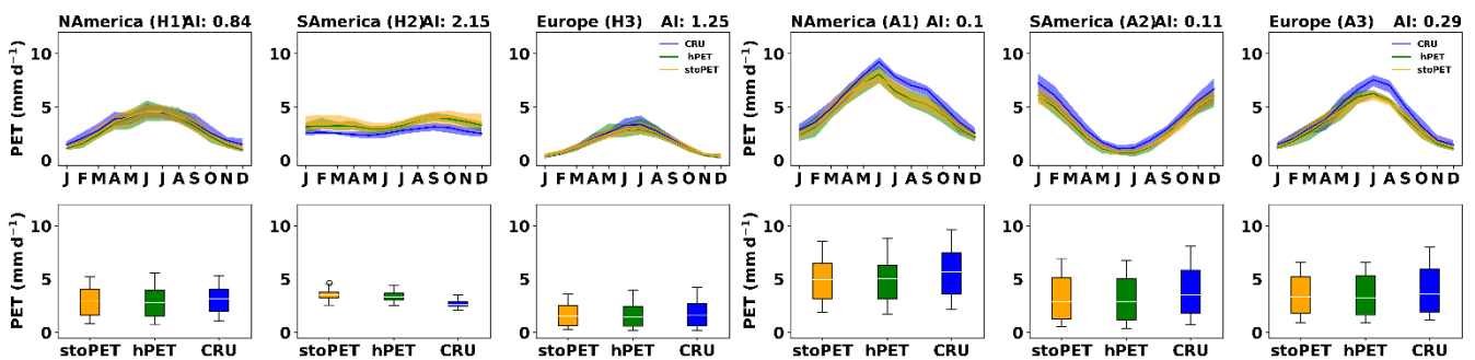
Figure 8: The seasonal PET and box plots for three datasets over North America, South America, and Europe for the (a) humid and (b) arid locations as located in Fig. 7. The box plots show the distribution of each dataset over the 20 years period. The box indicates the IQR ( 25^{th} - 75^{th} ) while the upper whiskers are set to (75^{th} + 1.5 * IQR) and the lower whiskers are set to (25^{th} - 1.5 * IQR) .
