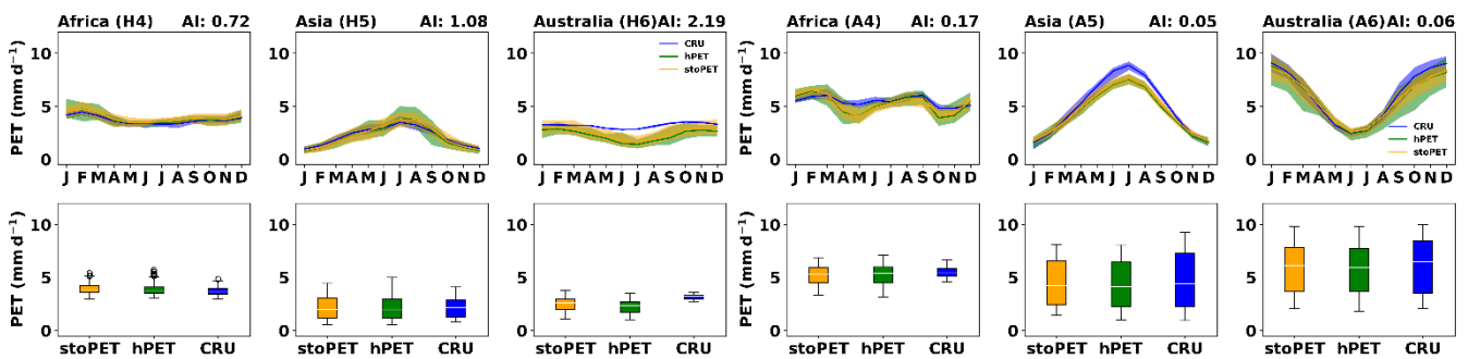
Figure 9: The seasonal PET and box plots for three datasets over Africa, Asia, and Australia (including Oceania region) for (a) humid and (b) arid locations as located in Fig. 7. The box plots show the distribution of each dataset over the 20 years period. The box indicates the IQR ( 25^{th} - 75^{th} ) while the upper whiskers are set to (75^{th} + 1.5 * IQR) and the lower whiskers are set to (25^{th} - 1.5 * IQR) .
