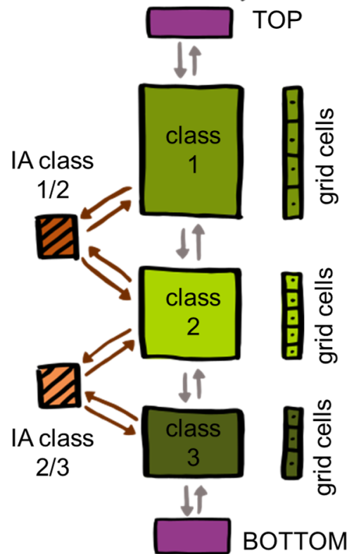
Figure 2. Example of a CryoGrid stratigraphy in the tile class TILE_1D_standard , consisting of the stratigraphy classes 1 to 3 coupled by interaction (IA) classes that specify the exchange of heat and mass between pairs of stratigraphy classes. The stratigraphy is realized as a linked list, with pointers between classes and interaction classes (symbolized by arrows), and the top and bottom of the list represented by a dedicated TOP and BOTTOM class (which have no other functionality). Each stratigraphy class has its own model grid and state variables.
