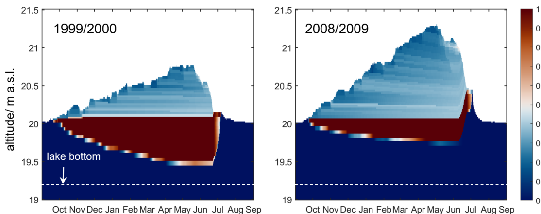
Figure 22. Simulated ice dynamics (volumetric ice content) for the water body simulation (red in Fig. 21) for a winter with low and high snow depths. As snow melt water is assumed to pass through the water body ice in the model, the ice rises in elevation during the melt period which is particularly evident in 2008/2009.
