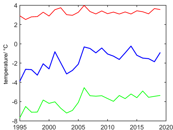
Figure 21. Simulated annual average temperatures at 1.3 m depth. Blue: reference simulation for soil material; red: 0.8 m deep water body overlying soil material (as for the reference simulation); green: glacier.
