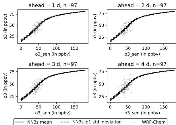
Figure 11. Sensitivity of NN3s forecasts for an exemplary station located at 50.770382^{\circ}\text{N} and 9.459403^{\circ}\text{E} with respect to ozone. Light grey lines correspond to individual test set's samples. Solid black line represents the mean, while dashed lines represent \pm one standard deviation. Light grey dots (97) represent each sample's daily aggregated WRF-Chem values at timestep t_0 . The solid black line represents the mean sensitivity across all samples, and the dashed black lines represent \pm one standard deviation, respectively. Sensitivities are shown individually for all lead times (1d to 4d).
