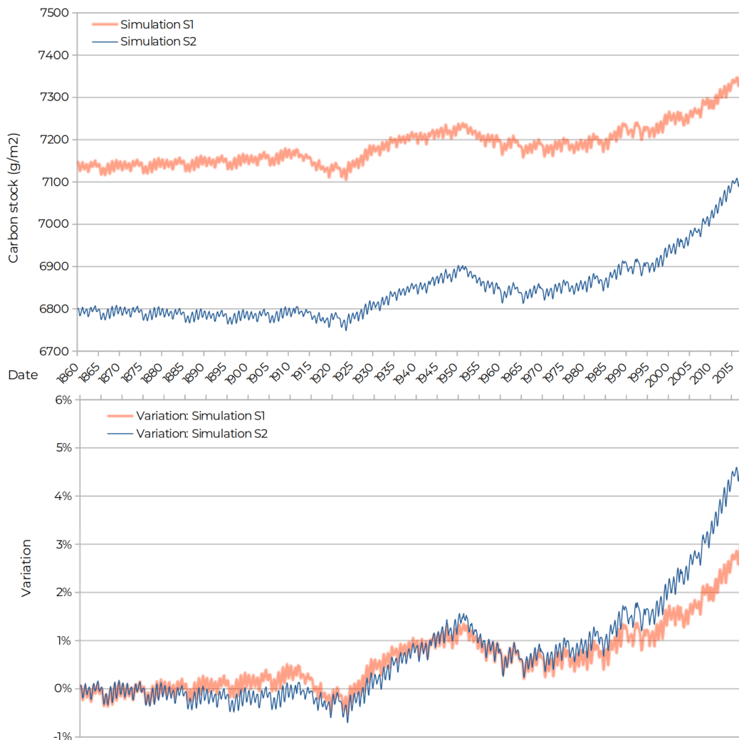
Figure 10. Results for the depositional site: absolute values of carbon stock (g/m 2 ) (top), relative difference (bottom).
