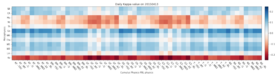
Figure S1. The heat map of average kappa for every configuration for the clusters of microphysics (Y axis) with the cluster of cumulus parameterization and PBL (x-axis) on the simulation case 2015-04-13. The data is only use the last 36 hours of simulations for calculating the kappa.
