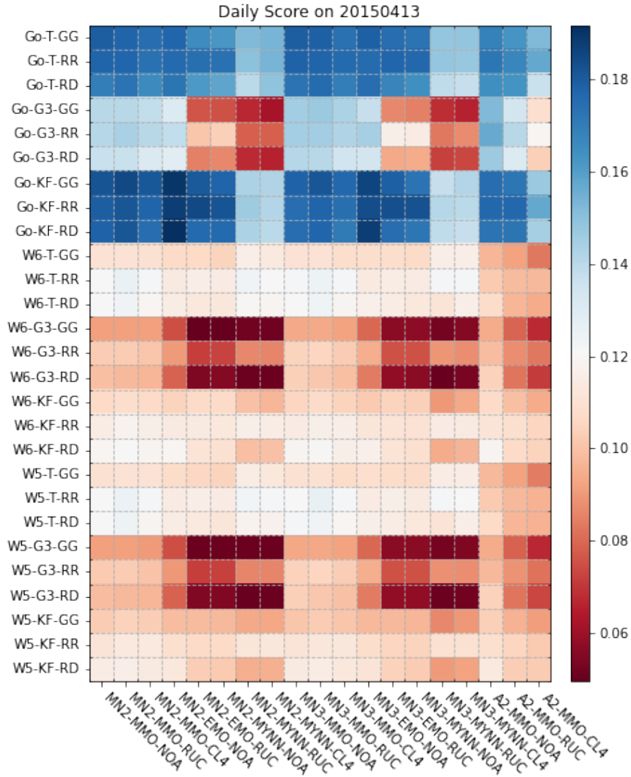
Figure S5. The heat map of the average kappa for the configuration for the clusters of microphysics, cumulus parameterization, and the radiation physics (Y axis) with the cluster of PBL-physics, surface physics, and the land surface model (x-axis) on the simulation case 2015-04-13. The data is only use the last 36 hours of simulations for calculating the kappa.
