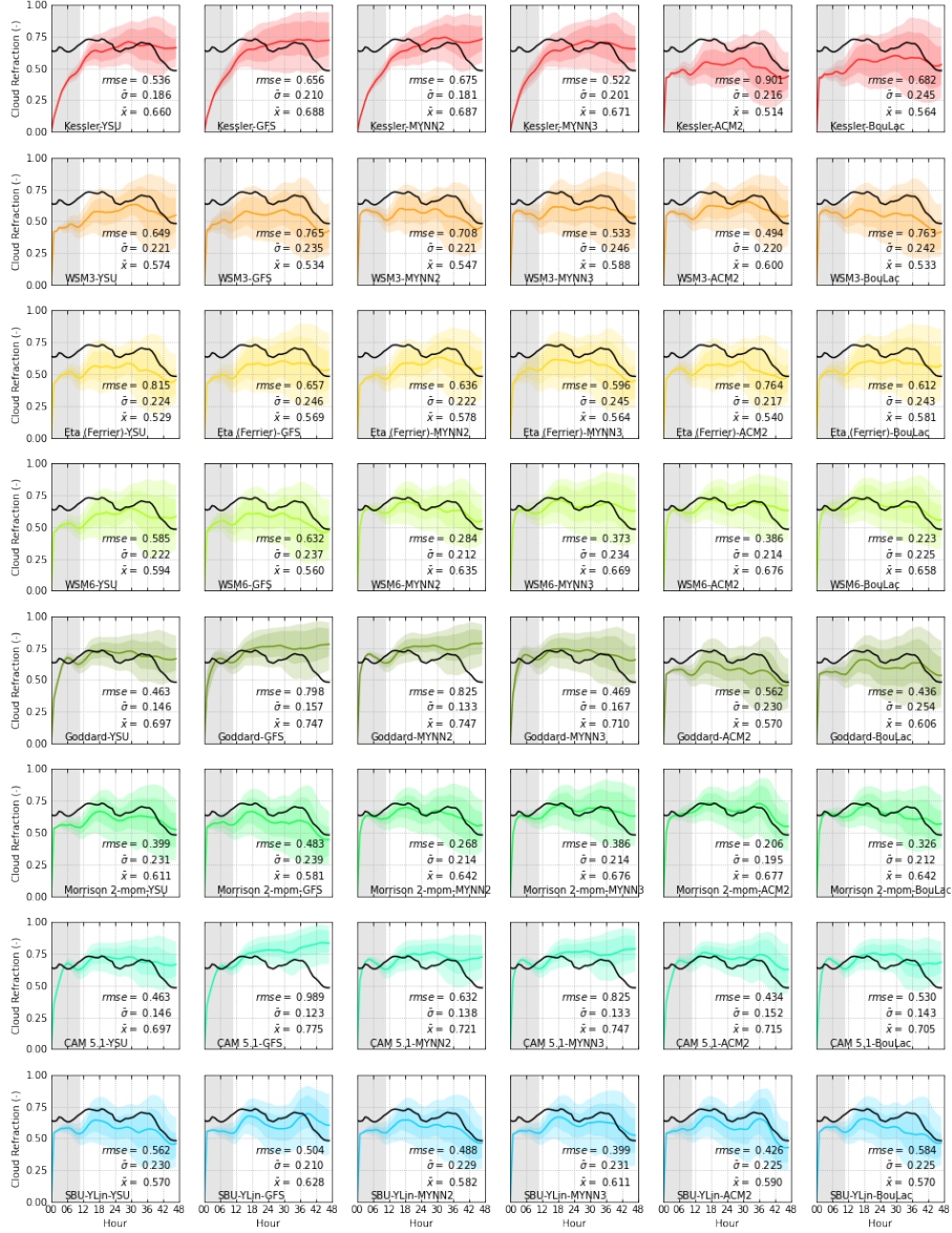
Figure S12. The mean cloud cover fraction (-) the observation from the satellite (black line) and by simulation (color line) from the combination of microphysics (by different color) and PBL physics (in different row) in case 2015-07-19. The color block represents the range of percentiles, the darker block is limited between 25% and 75%, and the lighter block is limited between 5% and 95%. The grey block indicates the spin-up time for ESIAS-met, which is not included in the root mean square error rmse , standard deviation ( \bar{\sigma} ), and the mean simulated cloud cover fraction ( \bar{x} ).
