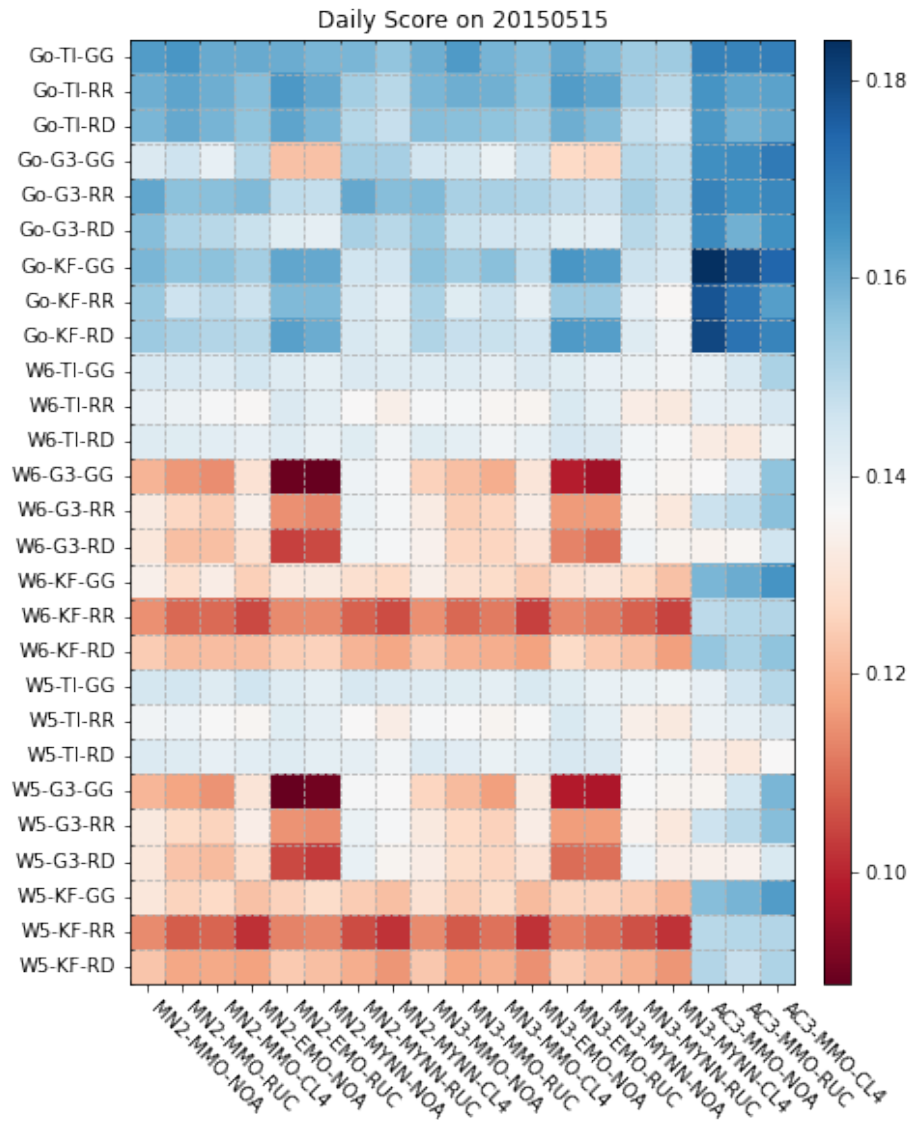
Figure S6. The heat map of the average kappa for the configuration for the clusters of microphysics, cumulus parameterization, and the radiation physics (Y axis) with the cluster of PBL-physics, surface physics, and the land surface model (x-axis) on the simulation case 2015-05-15. The data is only use the last 36 hours of simulations for calculating the kappa.
