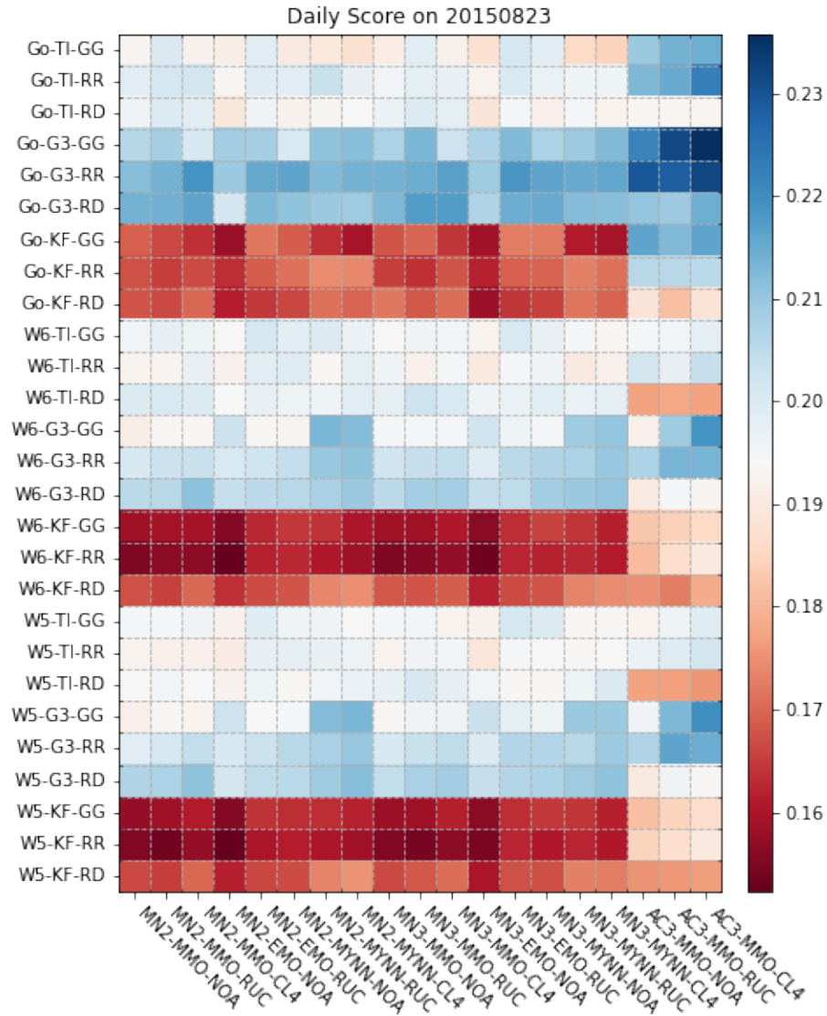
Figure S8. The heat map of the average kappa for the configuration for the clusters of microphysics, cumulus parameterization, and the radiation physics (Y axis) with the cluster of PBL-physics, surface physics, and the land surface model (x-axis) on the simulation case 2015-08-23. The data is only use the last 36 hours of simulations for calculating the kappa.
