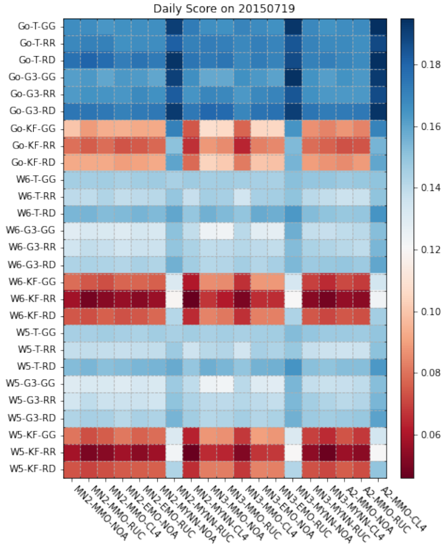
Figure S7. The heat map of the average kappa for the configuration for the clusters of microphysics, cumulus parameterization, and the radiation physics (Y axis) with the cluster of PBL-physics, surface physics, and the land surface model (x-axis) on the simulation case 2015-07-19. The data is only use the last 36 hours of simulations for calculating the kappa.
