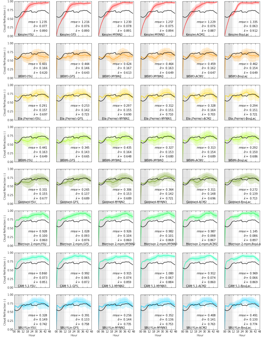
Figure S9. The mean cloud cover fraction (-) the observation from the satellite (black line) and by simulation (color line) from the combination of microphysics (by different color) and PBL physics (in different row) in case 2015-04-13. The color block represents the range of percentiles, the darker block is limited between 25% and 75%, and the lighter block is limited between 5% and 95%. The grey block indicates the spin-up time for ESIAS-met, which is not included in the root mean square error rmse , standard deviation ( \hat{\sigma} ), and the mean simulated cloud cover fraction ( \hat{x} ).
