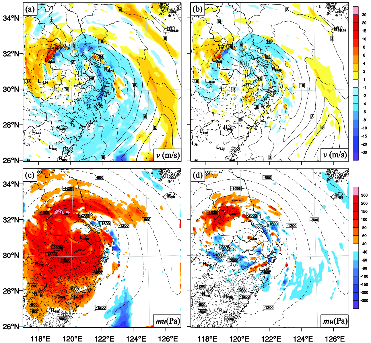
985 Figure 19 The difference in (a, b) meridional wind and (c, d) the dry-air mass in column ( \mu ) between the truth (contours) and forecast (shading) at 18 UTC 26 July 2021 (the last analysis cycle) for (a, c) Ens_noFLTR_6h and (b, d) Hybrid_5band_DSL_6h .
