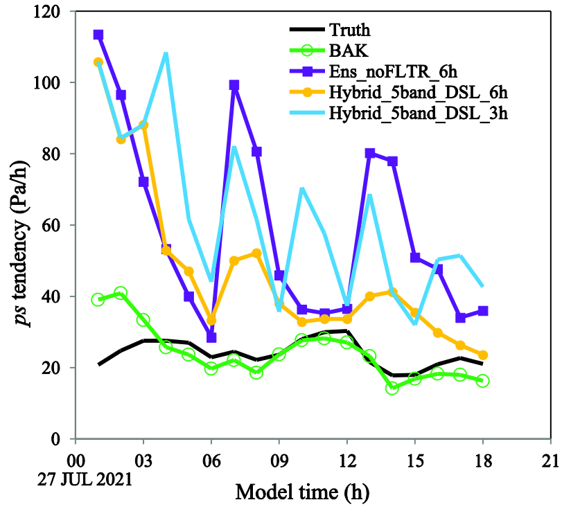
970 Figure 17 The tendency of surface pressure ( \text{Pa h}^{-1} ) for Truth (black), BAK (green), Ens_noFLTR (blue), Hybrid_5band_DSL_6h (orange), and Hybrid_5band_DSL_3h (light blue)
