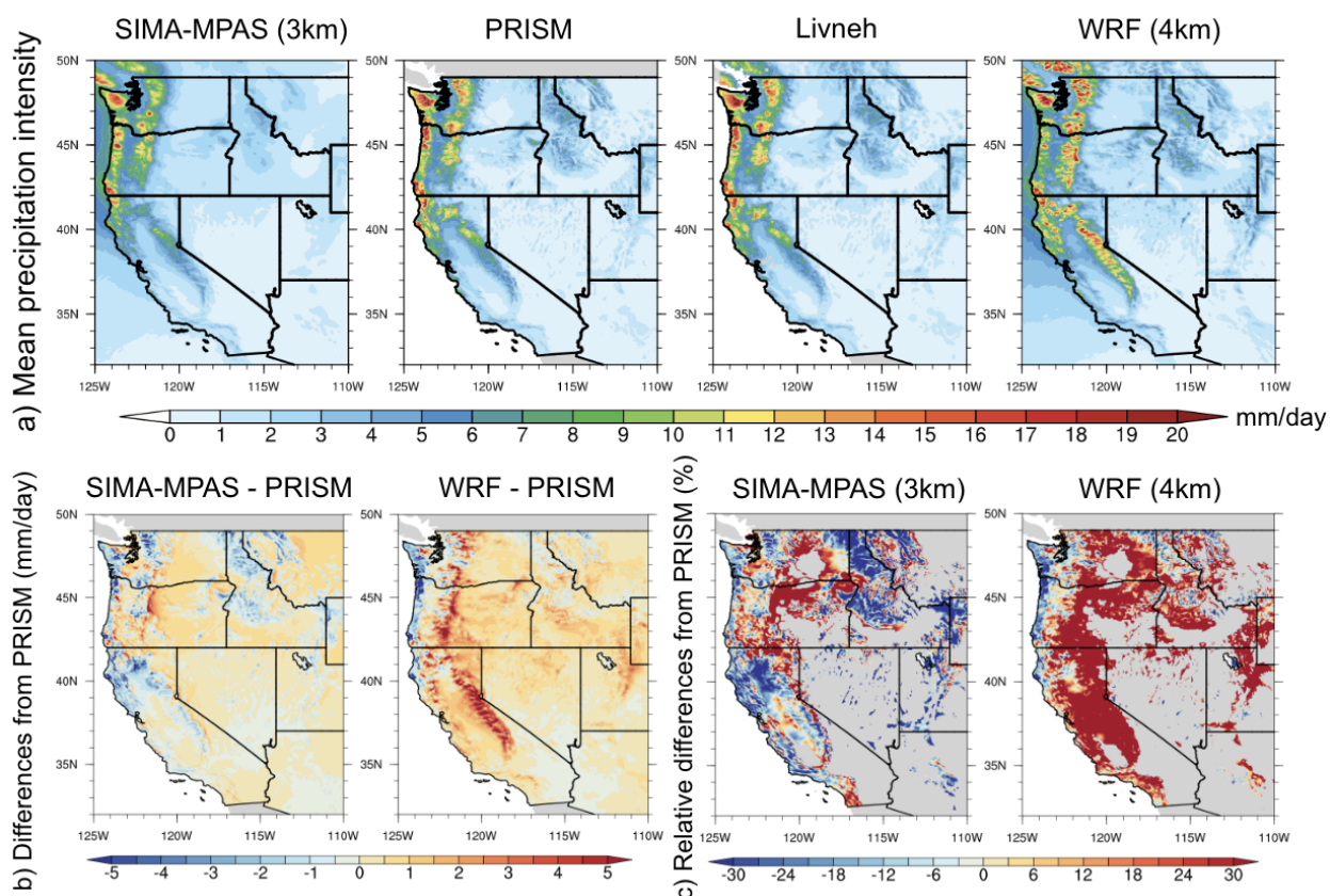
Figure 4: Mean simulated precipitation and differences from observation: a) Wet-season (mid-Nov to mid-March) daily precipitation intensity over western US (1999-2004); b) Absolute differences from PRISM reference; c) Similar as b, but for relative differences from PRISM (grid box values less than 1mm/day have been masked)) with the SIMA-MPAS model data regridded to the same resolution as the PRISM grid spacings (i.e., 4 km).
