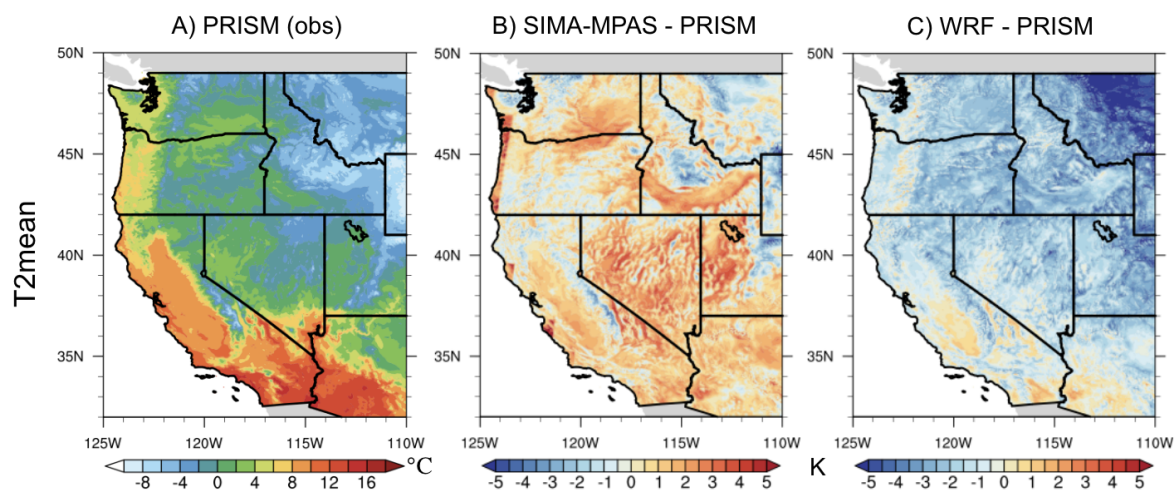
Figure 8: Daily mean 2m air temperature (T2mean) averaged over (1999-2004, Nov-March). A) PRISM observation dataset; B) and C) The differences between SIMA-MPAS and WRF from PRISM respectively; (Note: for difference plot, all data are regridded to the same resolution as PRISM).
