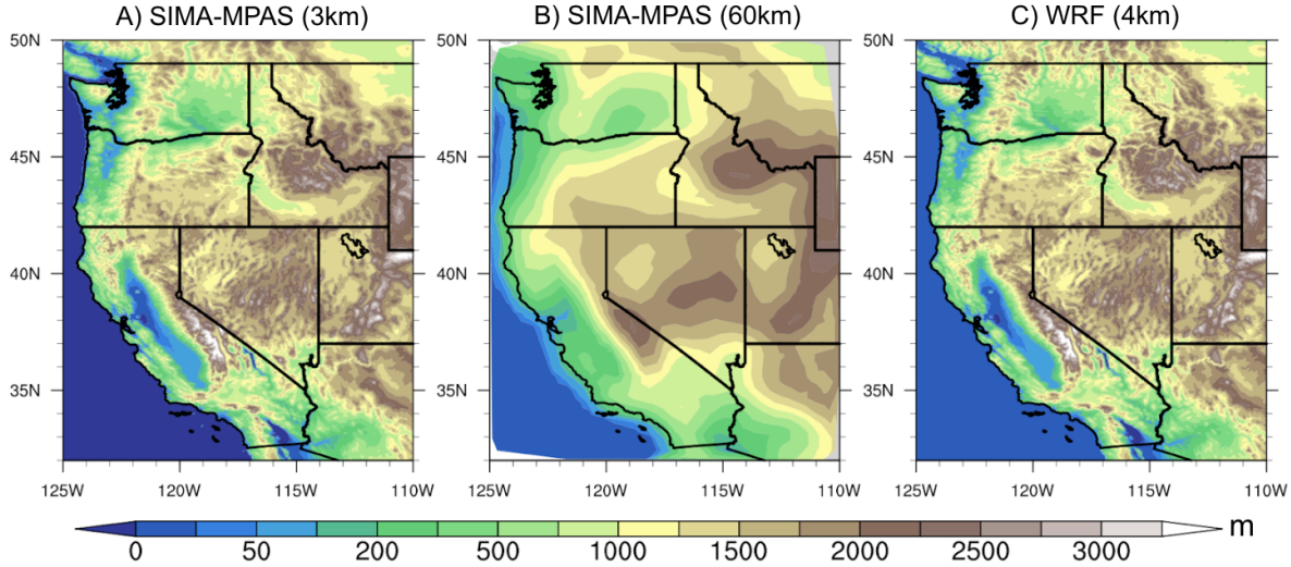
Figure 2: Topography over the western US region. A) SIMA-MPAS at 3km refinement, B) SIMA-MPAS uniform 60km grid mesh, and C) WRF simulations at 4km over CONUS.
