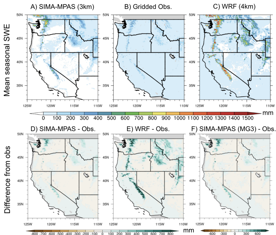
Figure 7: Wet-season snow water equivalent (SWE) over western US. First row: Seasonal mean SWE averaged over (1999-2004) from A) SIMA-MPAS, B) Gridded observation for SWE as described in the section 2.2, and C) WRF data; Second row (D, E, F): Absolute differences from observation with all data regridded to 4 km for SIMA-MPAS and WRF averaged over (1999-2004), and SIMA-MPAS (MG3) averaged over (1999-2002).
