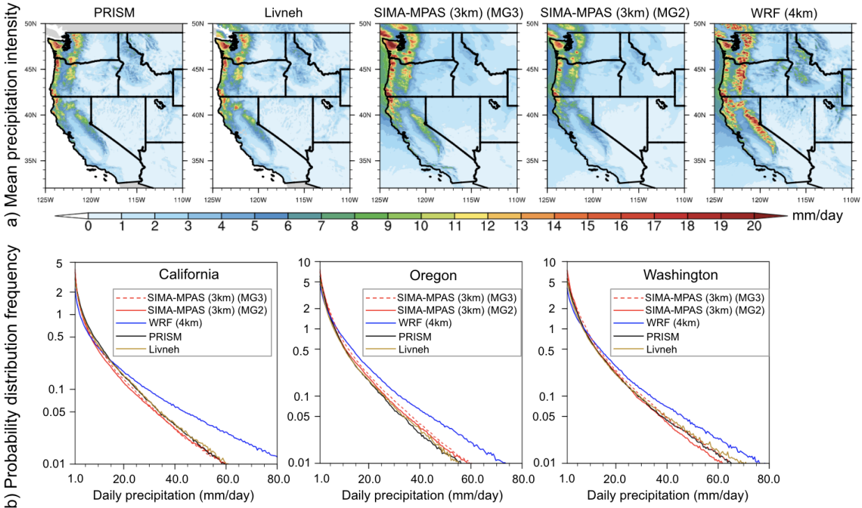
Figure 6: MG2 vs. MG3 microphysics used in SIMA-MPAS for the wet-season precipitation over western US (1999-2002). a) mean precipitation intensity; b) Probability distribution of daily precipitation frequency, like Figure 5 but for three wet seasons with SIMA-MPAS (MG3) added in dashed red lines; Again, the SIMA-MPAS model data is regridded to the same resolution as the PRISM grid spacings (i.e., 4 km).
