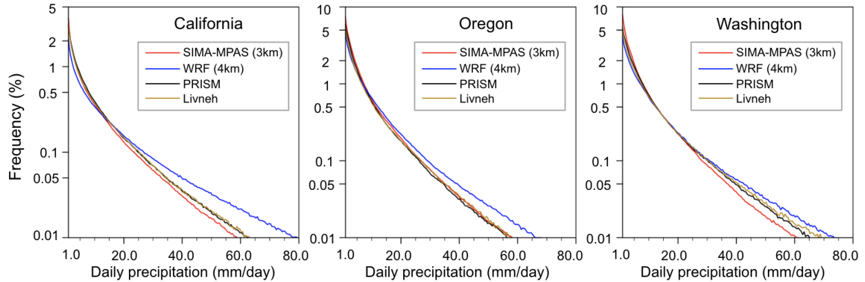
Figure 5: Probability distribution of daily precipitation frequency intensity. All the daily datasets from the five wet seasons for all grid points in each State are used to construct the distribution statistics. The blue lines refer to WRF reference data, the black lines are for the PRISM observation, the dark golden line refers to the Livneh observation, and the SIMA-MPAS results are in red-colored lines. The SIMA-MPAS model data is regridded to the same resolution as the PRISM grid spacings (i.e., 4 km). The x-axis starts from 1mm/day and the y-axis is transformed with a logarithmic scaling for better visualization of the upper tail distribution.
