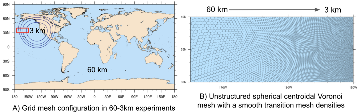
Figure 1: in-SIMA-MPAS mesh configuration for the 60-3km experiments . A) The global domain mesh configuration with total grid columns of 835586; B) The zoomed-in region (see the red box depicted in panel A)) for the mesh structure from 60km to 3km.
