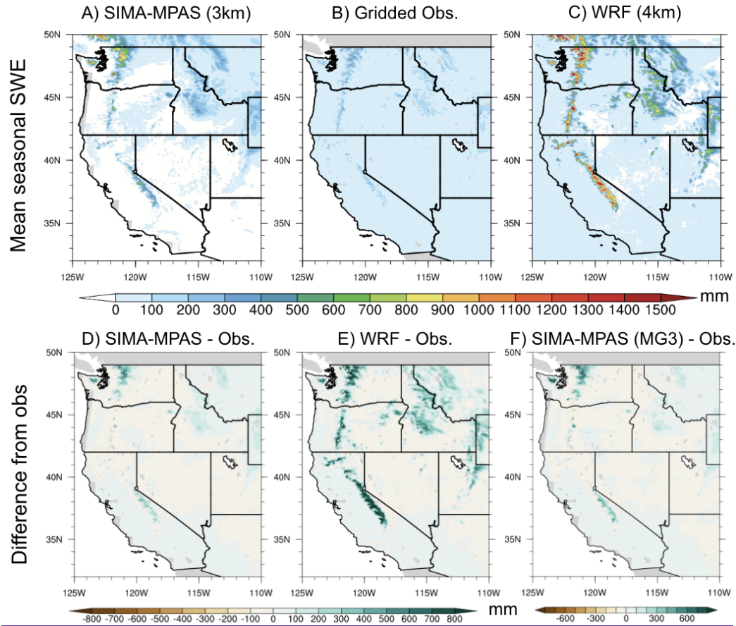
Figure 7: Wet-season (Nov. till March) snow water equivalent (SWE) over western US (1999-2004). First row: Seasonal mean SWE averaged over (1999-2004) from A) SIMA-MPAS, B) Daymet Gridded observation for SWE as described in the section 2.2, and C) WRF data; Second row: (D, E, F): Absolute differences from Daymet observation with all data regridded to 4 km for SIMA-MPAS and WRF averaged over (1999-2004), and SIMA-MPAS (MG3) averaged over (1999-2002).
