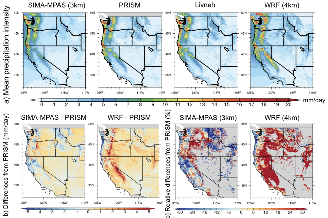
Figure 4: Mean simulated precipitation and differences from observation: a) Wet-season ( mid-Nov to mid-March ) daily precipitation intensity over western US (1999-2004); b) Absolute differences from PRISM reference; c) Similar as b, but for relative differences from PRISM (grid box values less than 1mm/day have been masked) with the SIMA-MPAS model data regridded to the same resolution as the PRISM grid spacings (i.e., 4 km).
